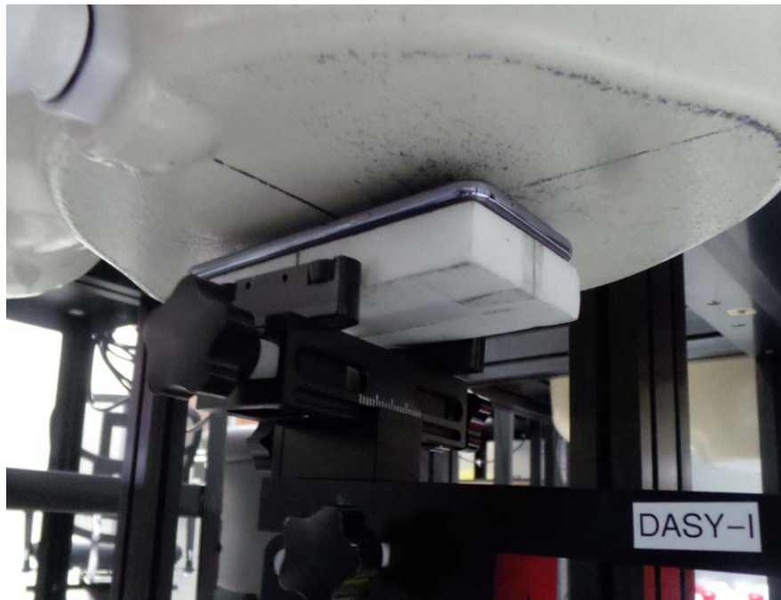
SAR Test Setup Photo 9: Front at 1.0 cm
