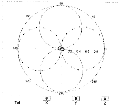
f=600 MHz,TEM,0°
