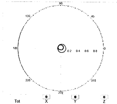
f=600 MHz,TEM,90°
