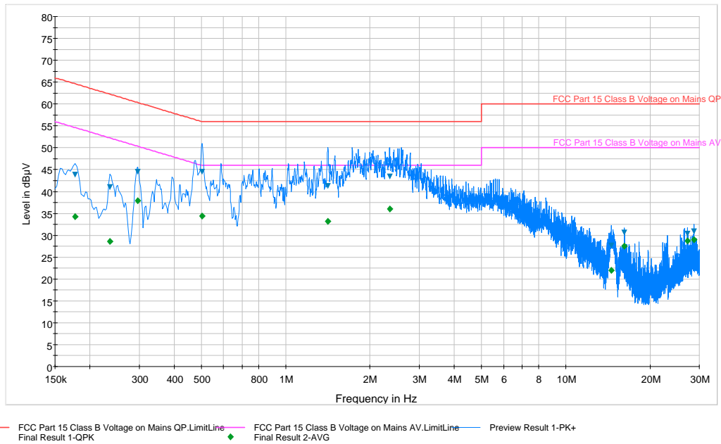
Plot 6-31. Line Conducted Plot with 802.11b (L1)
