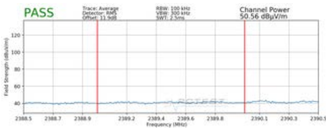
Plot 7-41. Radiated Restricted Lower Band Edge Measurement (Average)
