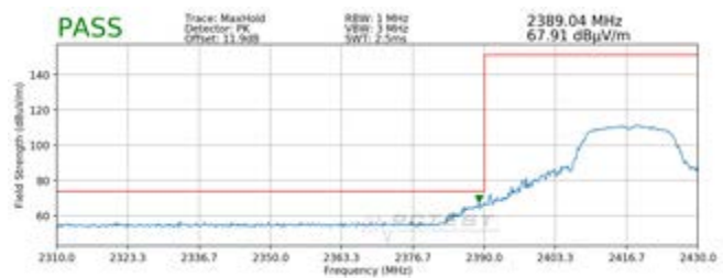
Plot 7-42. Radiated Restricted Lower Band Edge Measurement (Peak)
