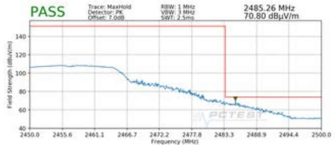
Plot 7-44. Radiated Restricted Upper Band Edge Measurement (Peak)
