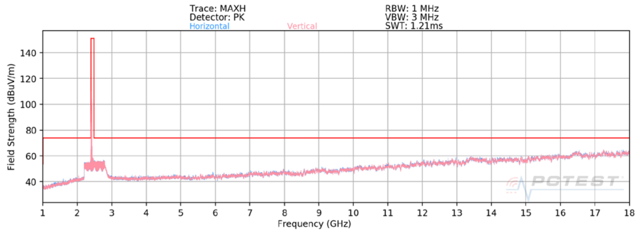
Plot 7-35. Radiated Spurious Plot above 1GHz (802.11b – Ch. 1)
