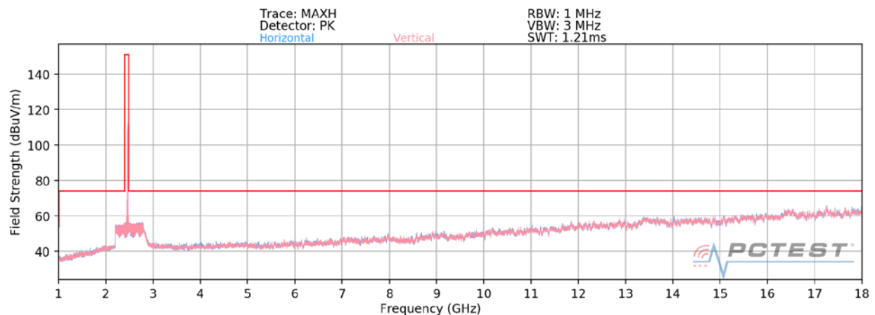
Plot 7-37. Radiated Spurious Plot above 1GHz (802.11b – Ch. 11)
