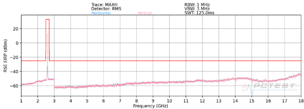
Plot 7-60. Radiated Spurious Plot (LTE Band 41(PC2))
