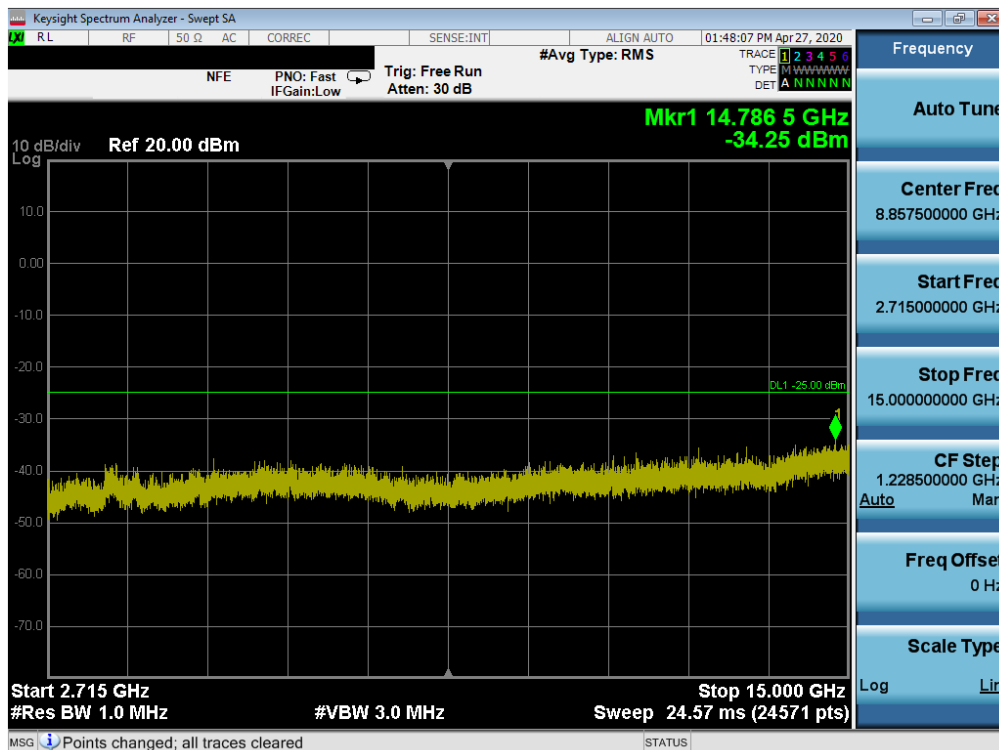
Plot 7-32. Conducted Spurious Plot (LTE Band 41(PC2) - 20MHz QPSK - RB Size 1, RB Offset 0 - High Channel)
