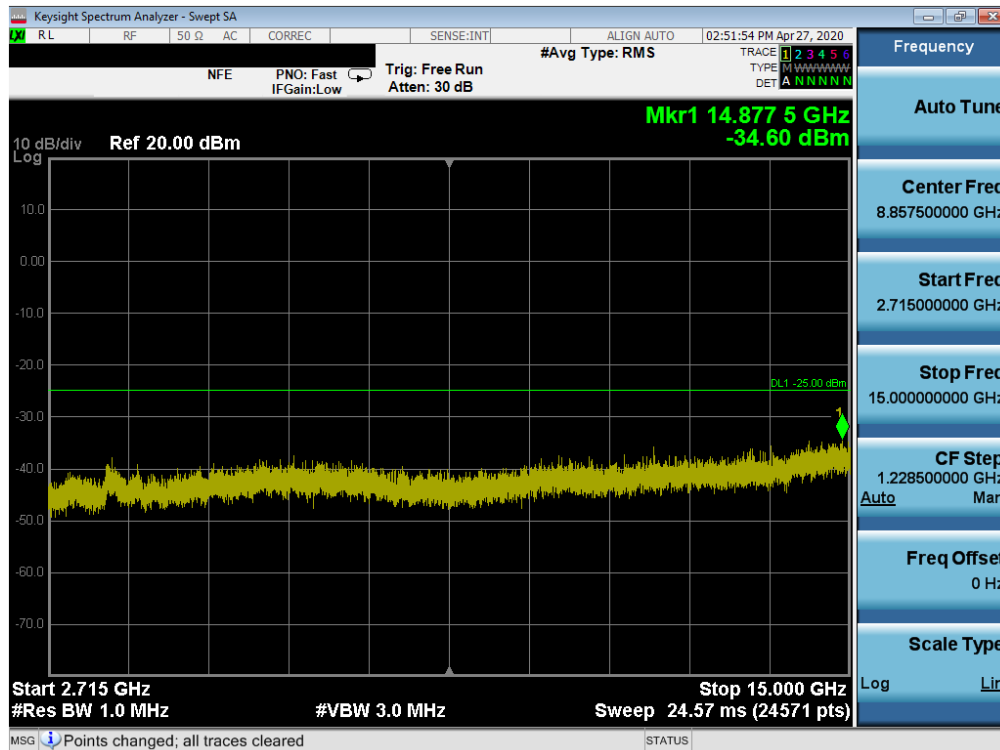
Plot 7-41. Conducted Spurious Plot (LTE Band 41(PCA) - 20MHz QPSK - RB Size 1, RB Offset 0 - High Channel)
