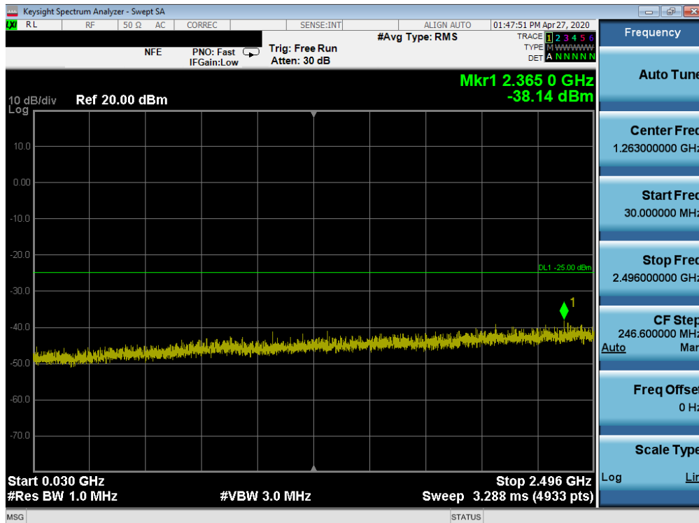
Plot 7-31. Conducted Spurious Plot (LTE Band 41(PC2) - 20MHz QPSK - RB Size 1, RB Offset 0 - High Channel)
