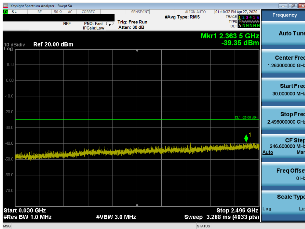
Plot 7-28. Conducted Spurious Plot (LTE Band 41(PC2) - 20MHz QPSK - RB Size 1, RB Offset 0 - Mid Channel)
