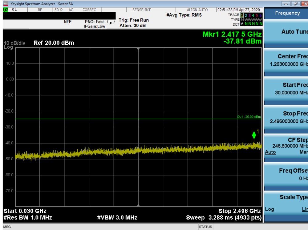
Plot 7-40. Conducted Spurious Plot (LTE Band 41(PCA) - 20MHz QPSK - RB Size 1, RB Offset 0 - High Channel)
