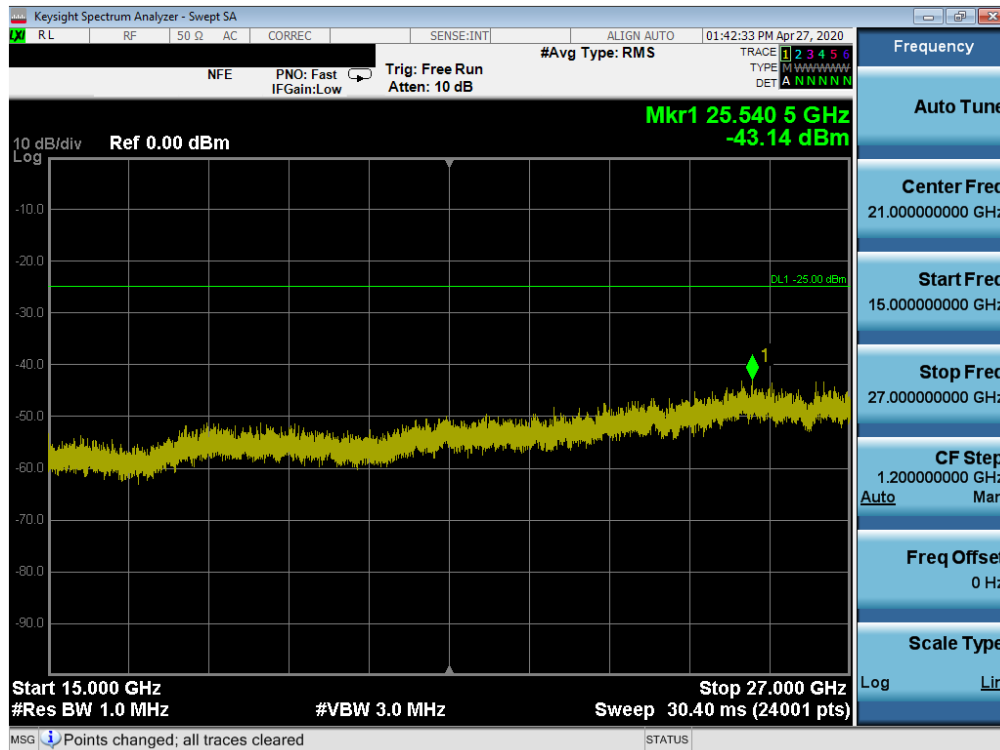
Plot 7-27. Conducted Spurious Plot (LTE Band 41(PC2) - 20MHz QPSK - RB Size 1, RB Offset 0 - Low Channel)
