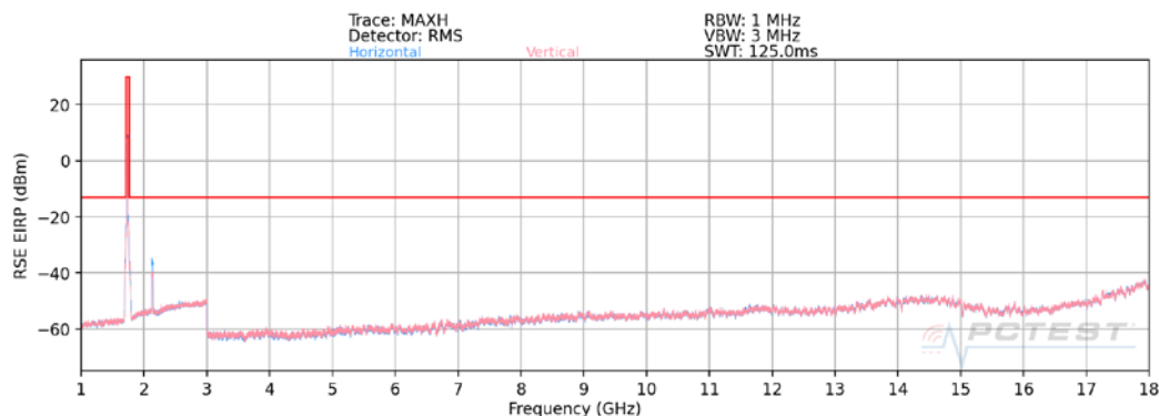
Plot 7-149. Radiated Spurious Plot (LTE Band 66/4)
