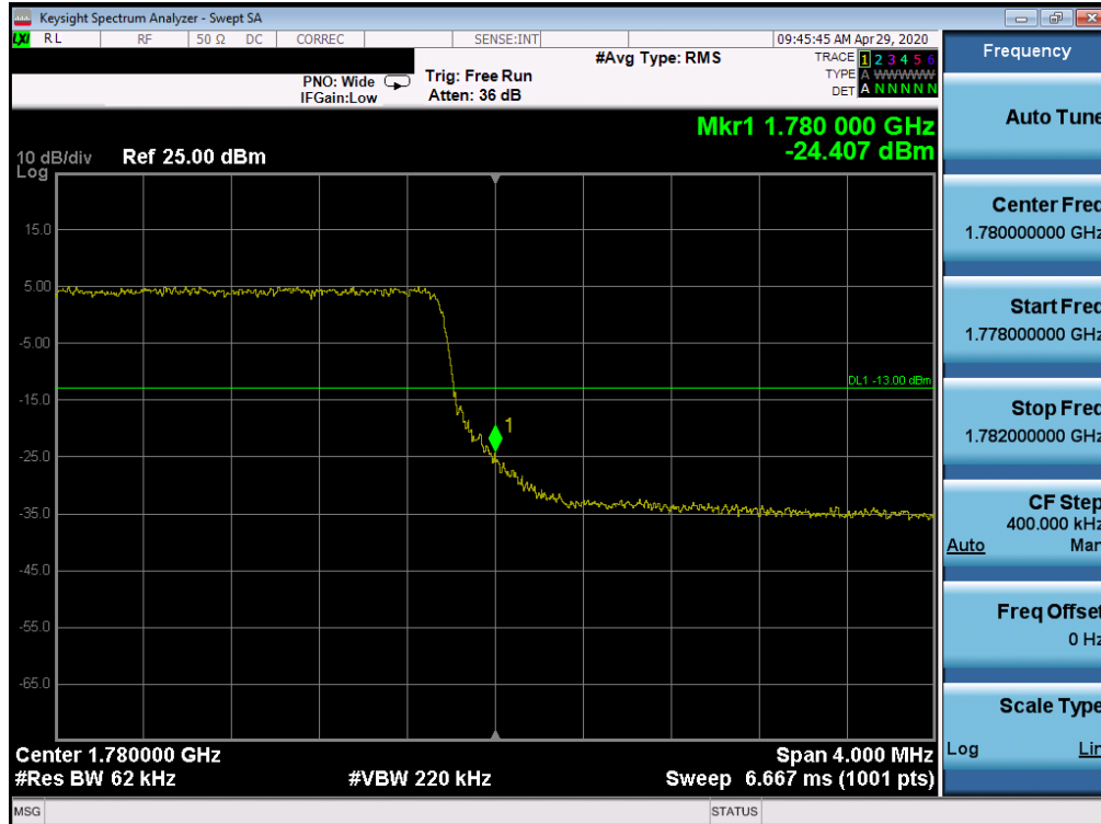
Plot 7-102. Upper Band Edge Plot (LTE Band 66 - 5MHz QPSK – Full RB Configuration)
