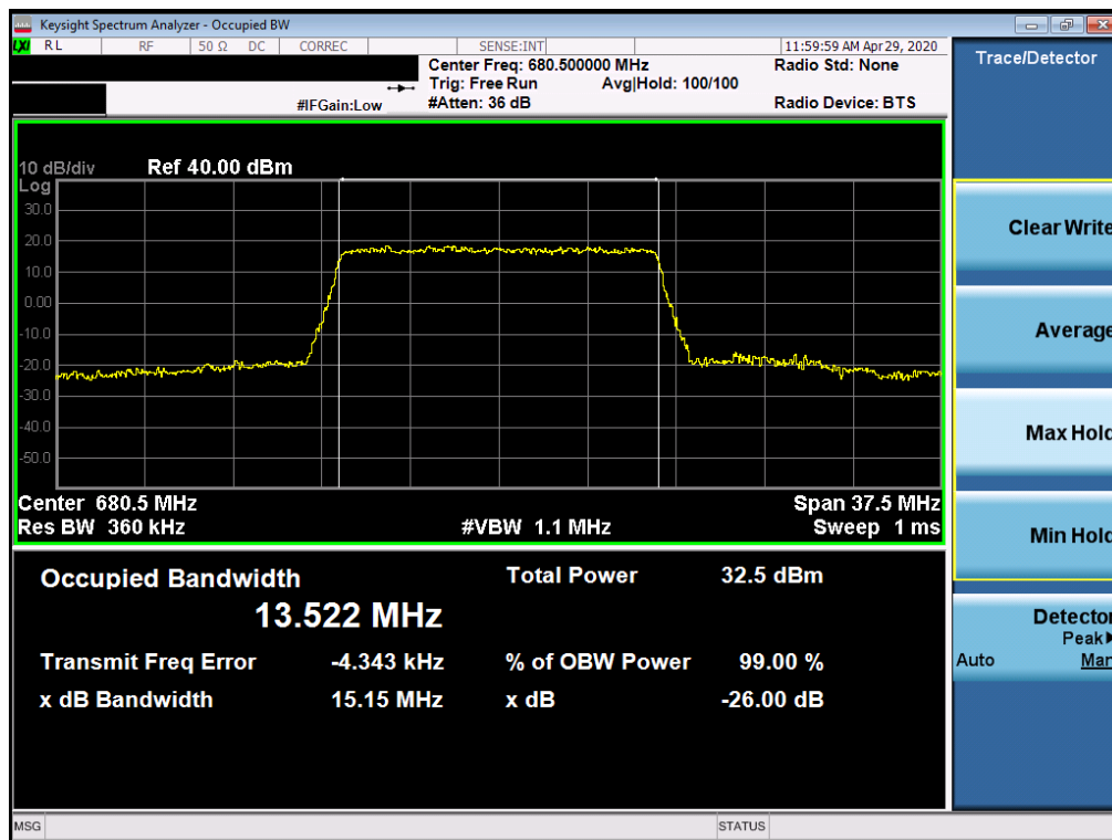
Plot 7-40. Occupied Bandwidth Plot (LTE Band 71 - 15MHz QPSK - Full RB Configuration)
