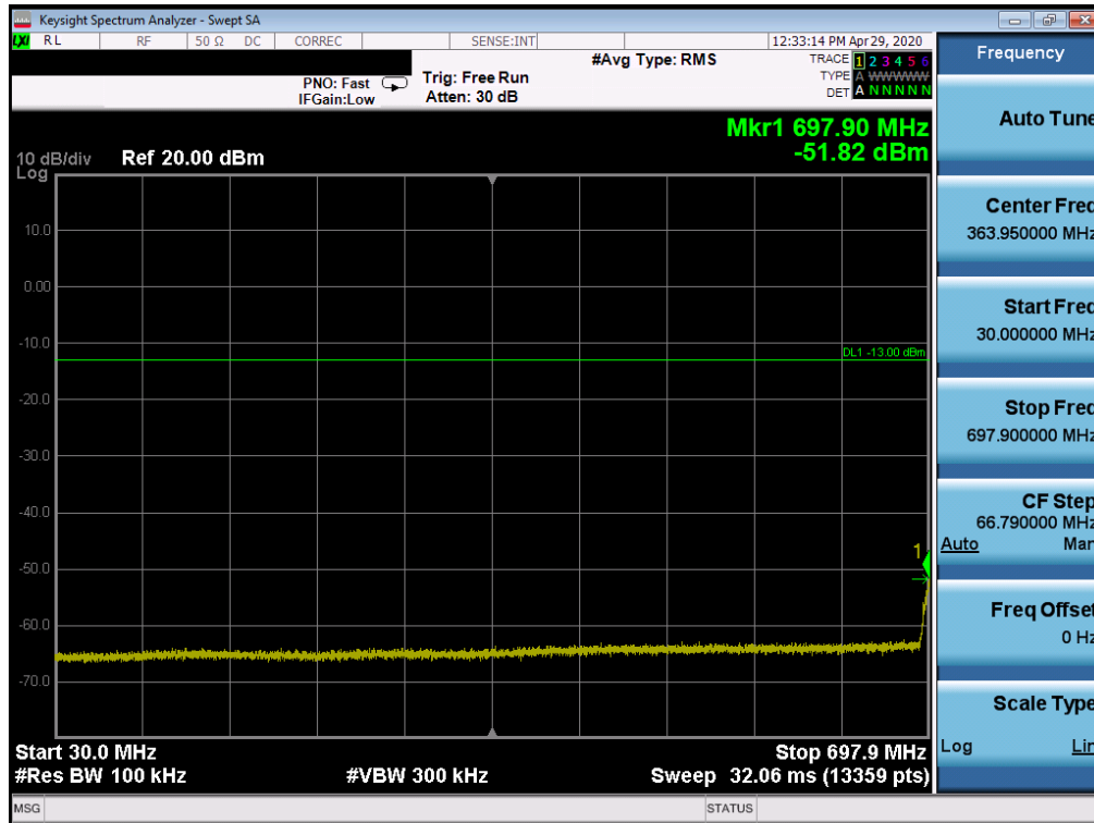
Plot 7-59. Conducted Spurious Plot (LTE Band 12 - 10MHz QPSK - RB Size 1, RB Offset 0 - Low Channel)
