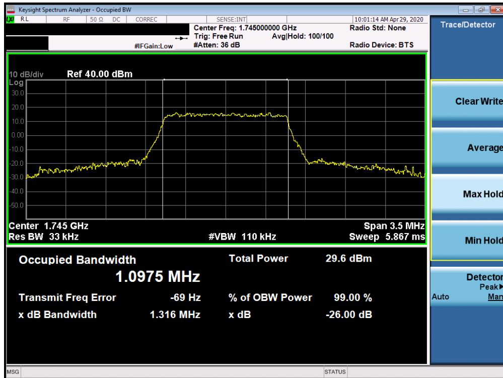
Plot 7-18. Occupied Bandwidth Plot (LTE Band 66/4 - 1.4MHz 64-QAM - Full RB Configuration)
