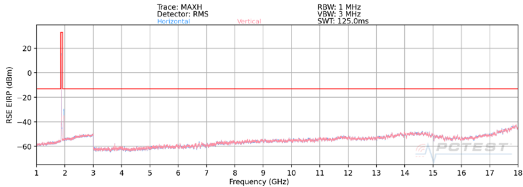
Plot 7-108. Radiated Spurious Plot (WCDMA PCS)
