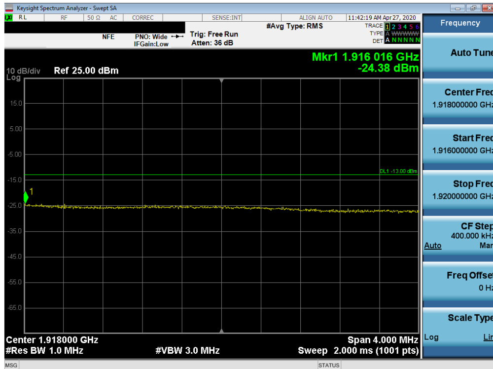
Plot 7-43. Extended Upper Band Edge Plot (LTE Band 25 - 15MHz QPSK – Full RB Configuration)
