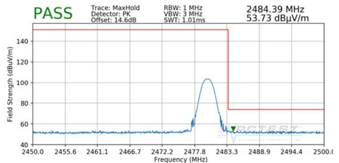
Plot 7-6. Radiated Restricted Upper Band Edge Measurement (Peak)
