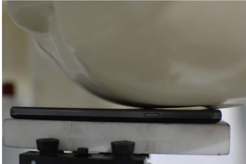
SAR Test Setup Photo – Left Cheek
