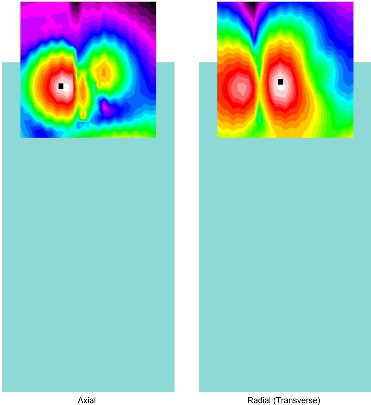
Figure 7-4 T-Coil Scan Overlay Magnetic Field Distributions
