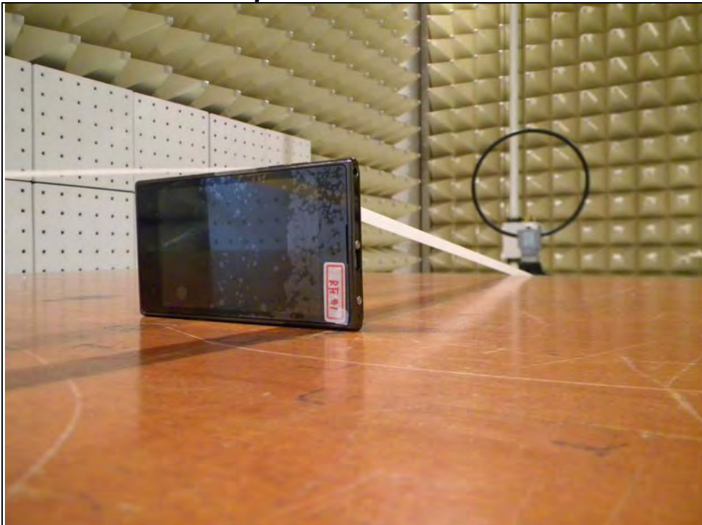
A. Photo of Fundamental & Spurious Emission Test for NFC
