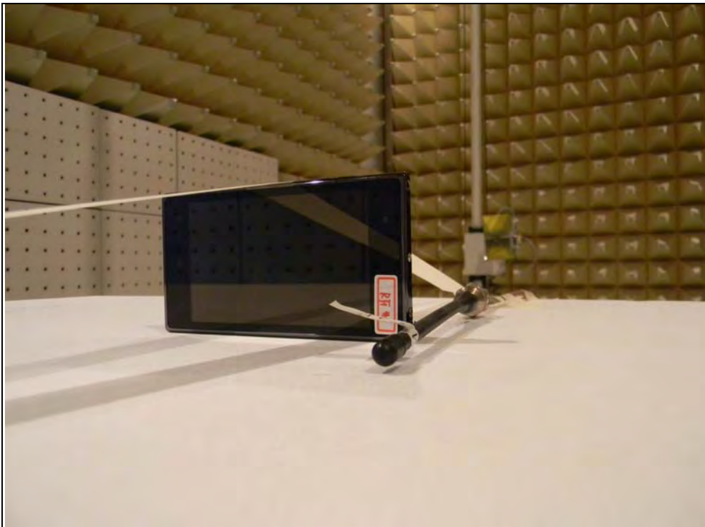
B. Photo of Field Strength & Spurious Emission Test for BT, WLAN & GSM
