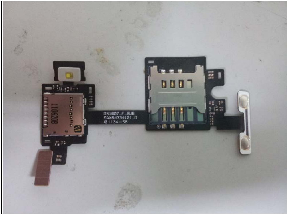
Bottom view of FPCB
