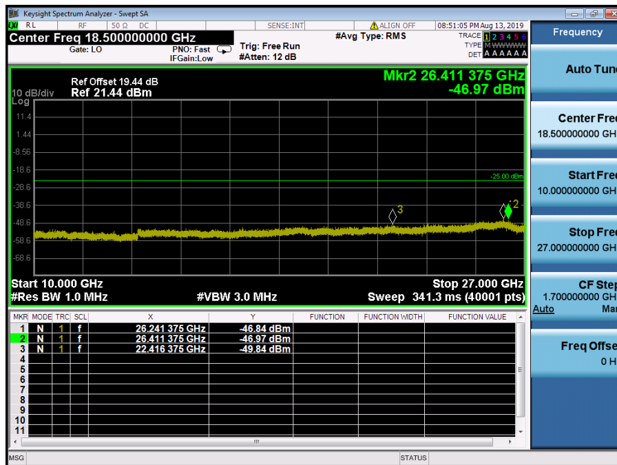
LTE Band 41 / 5MHz / 64QAM - RB Size/Offset (12/6) – Low Channel
