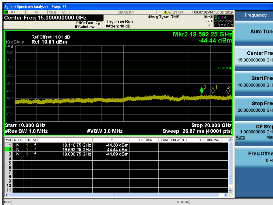
LTE Band 4 / 5MHz / QPSK - RB Size/Offset (12/0) – Low Channel
