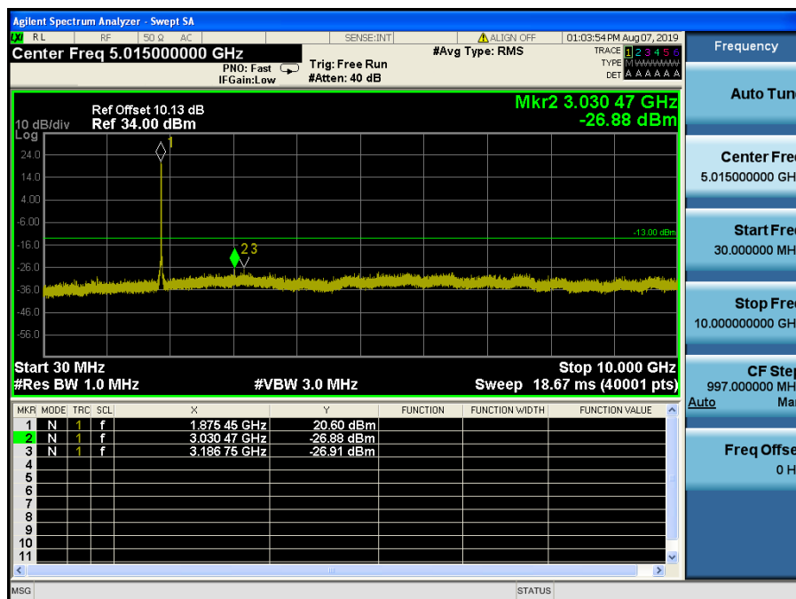
LTE Band 2 / 20MHz / 16QAM - RB Size/Offset (100/0)–Mid Channel
