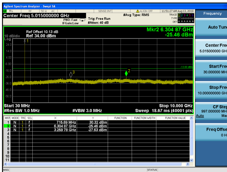
LTE Band 12, 17 / 10MHz / 64QAM - RB Size/Offset (1/49) – High Channel
