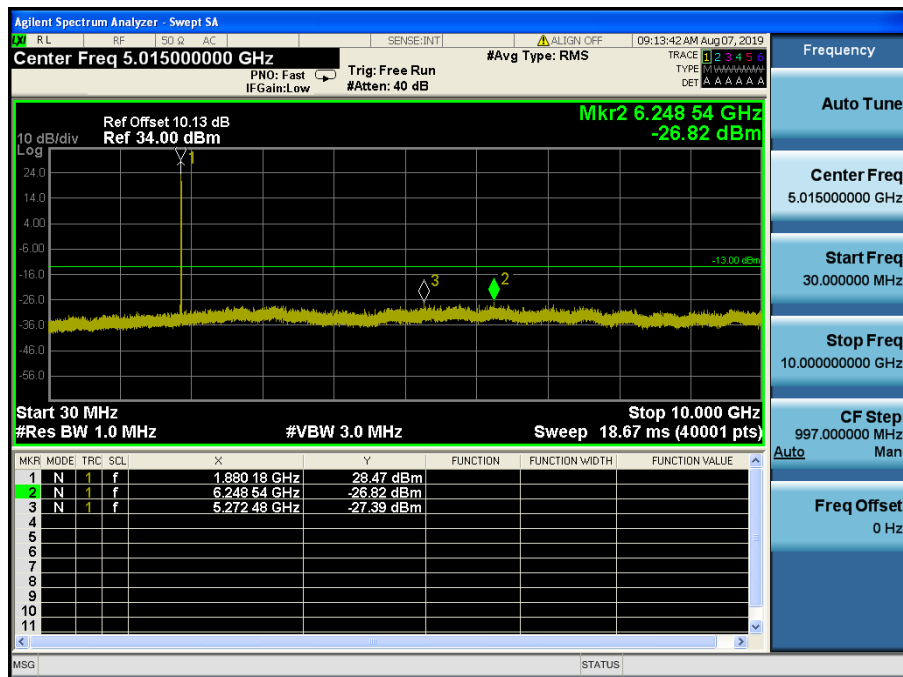
LTE Band 2 / 1.4MHz / 16QAM - RB Size/Offset (3/2) – Mid Channel
