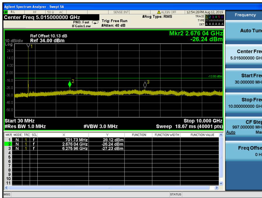
LTE Band 12 / 3MHz / 16QAM - RB Size/Offset (15/0) – Low Channel
