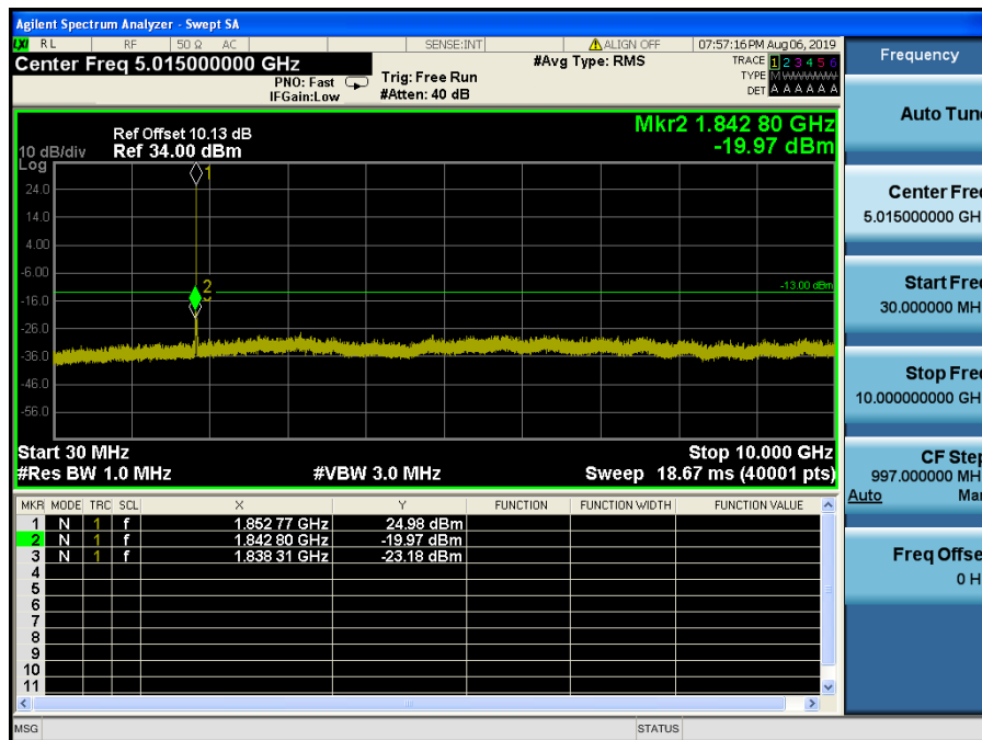
LTE Band 2 / 3MHz / QPSK - RB Size/Offset (15/0) – Low Channel
