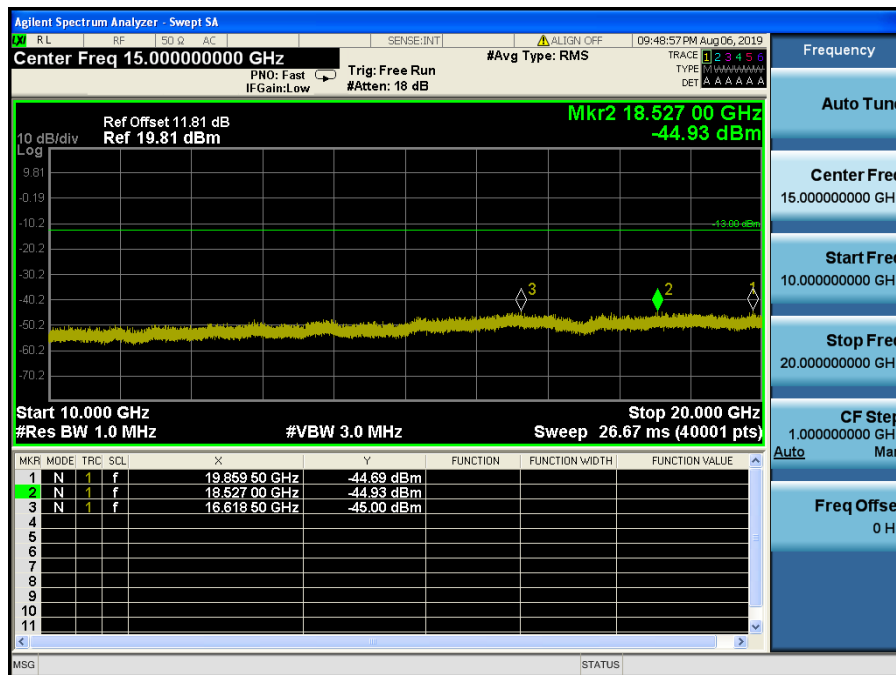
LTE Band 2 / 10MHz / QPSK - RB Size/Offset (1/25) – High Channel
