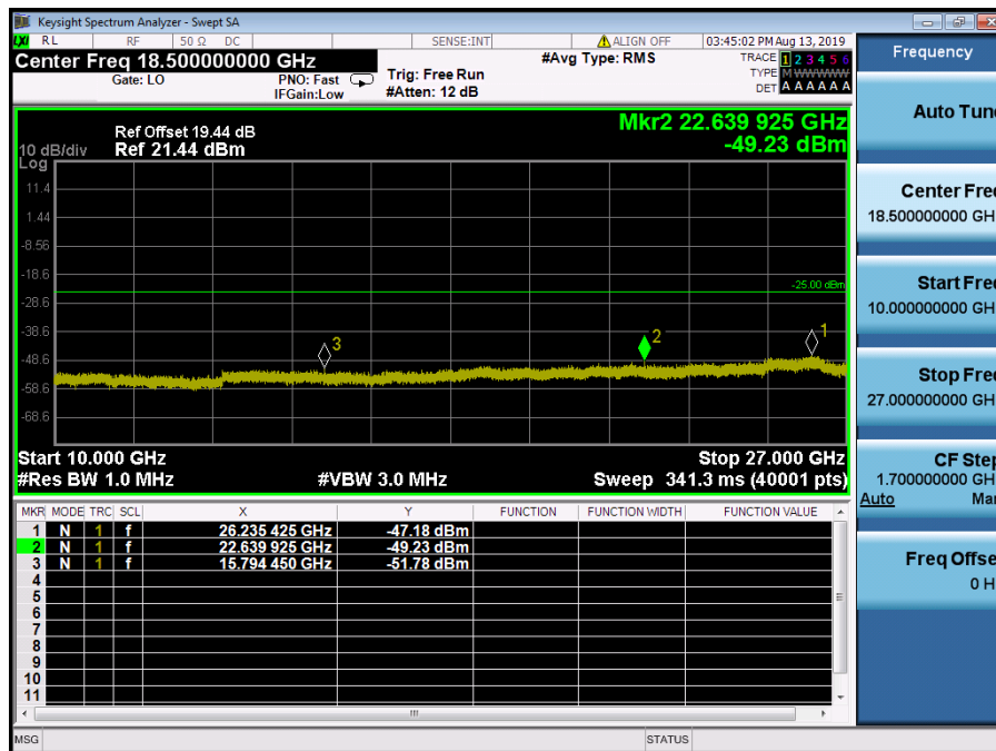
LTE Band 41 / 10MHz / QPSK - RB Size/Offset (1/0) – Mid Channel
