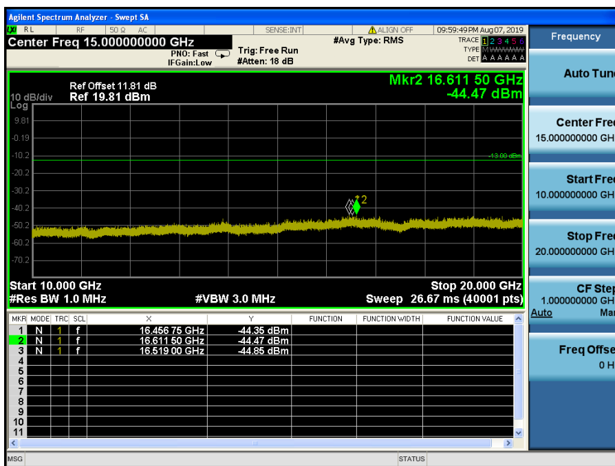
LTE Band 4 / 3MHz / QPSK - RB Size/Offset (8/0) – Mid Channel
