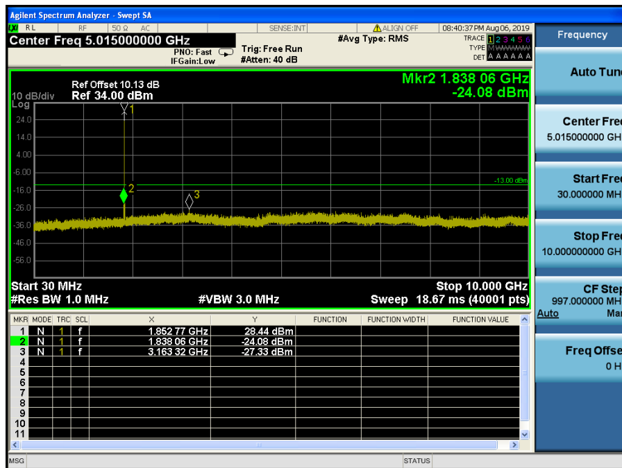
LTE Band 2 / 5MHz / QPSK - RB Size/Offset (1/12) – Low Channel
