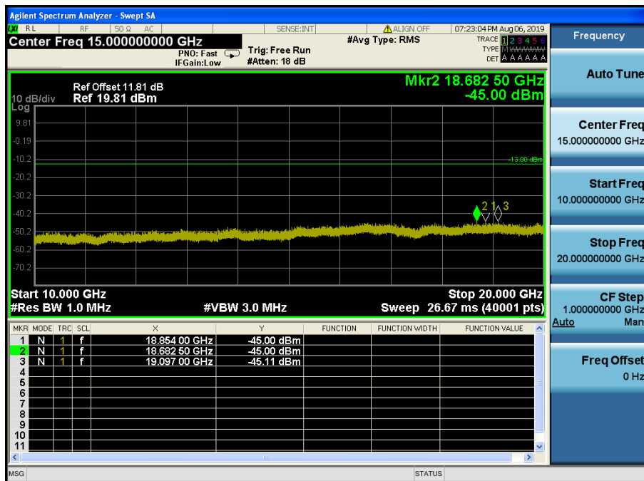
LTE Band 2 / 1.4MHz / QPSK - RB Size/Offset (1/2) – High Channel
