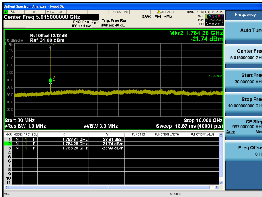
LTE Band 4 / 3MHz / QPSK - RB Size/Offset (1/7) – High Channel
