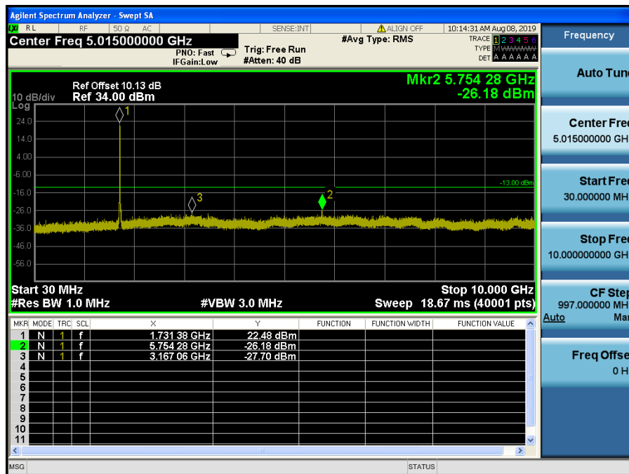
LTE Band 4 / 10MHz / QPSK - RB Size/Offset (50/0)– Mid Channel
