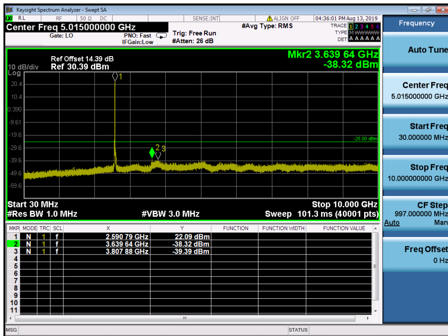
LTE Band 41 / 15MHz / QPSK - RB Size/Offset (36/0) – Mid Channel
