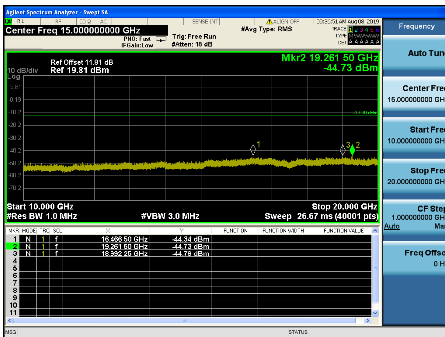
LTE Band 4 / 5MHz / QPSK - RB Size/Offset (12/13) – High Channel
