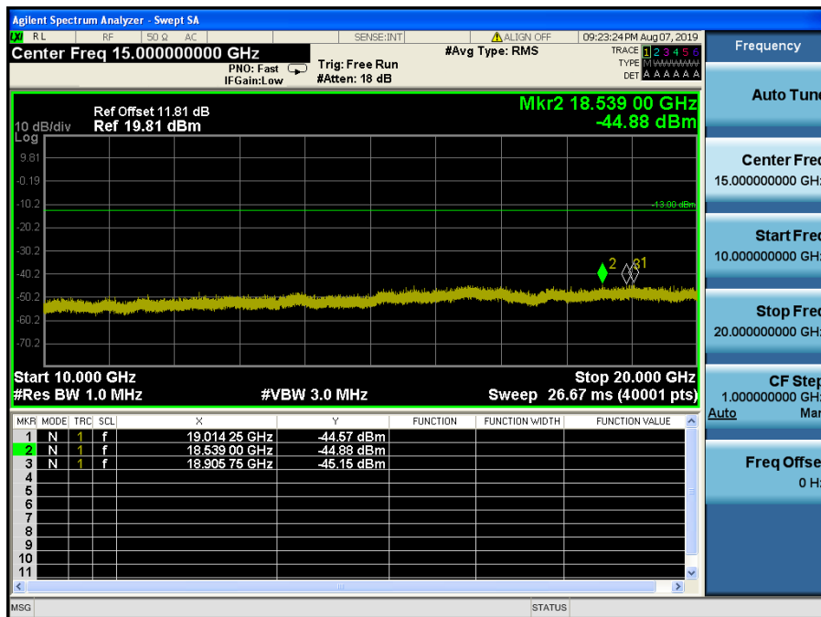
LTE Band 4 / 1.4MHz / QPSK - RB Size/Offset (1/2) – High Channel
