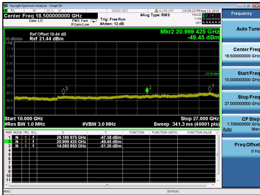
LTE Band 41 / 15MHz / 64QAM - RB Size/Offset (1/36) – High Channel
