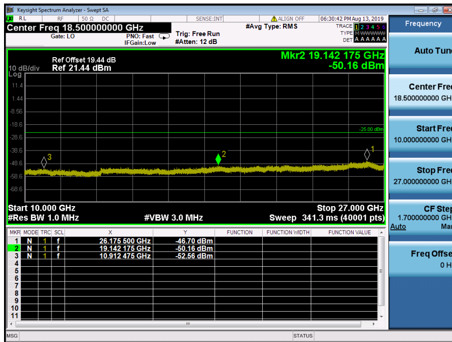
LTE Band 41 / 10MHz / 16QAM - RB Size/Offset (1/25) – Low Channel
