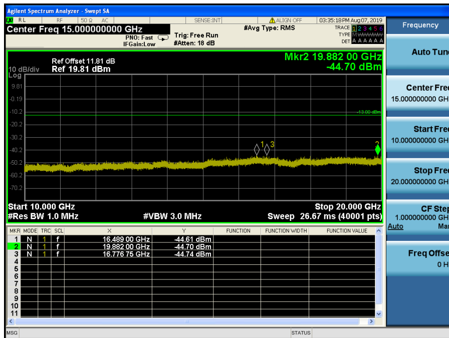
LTE Band 2 / 3MHz / 64QAM - RB Size/Offset (1/0) – Mid Channel
