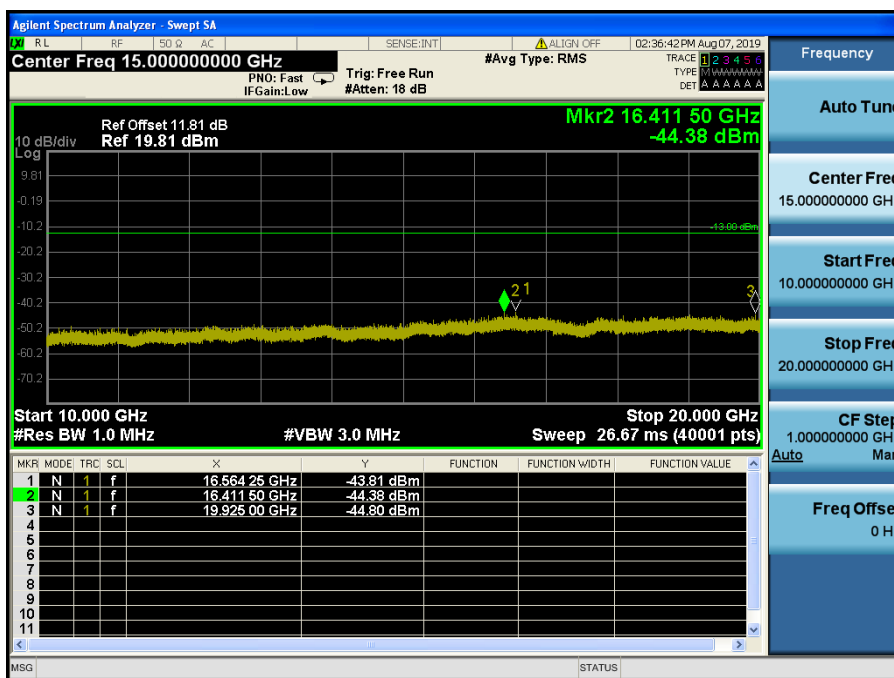
LTE Band 2 / 1.4MHz / 64QAM - RB Size/Offset (1/2) – Low Channel
