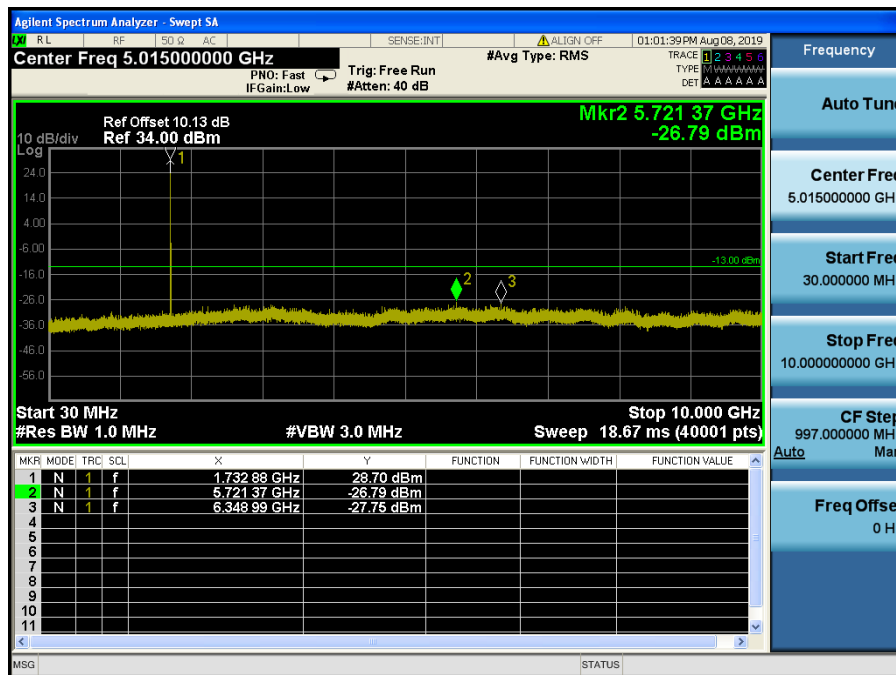
LTE Band 4 / 1.4MHz / 16QAM - RB Size/Offset (1/2) – Mid Channel
