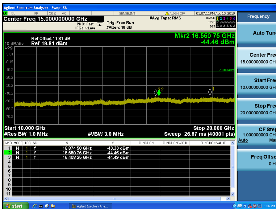
LTE Band 4 / 15MHz / 64QAM - RB Size/Offset (36/18)–Low Channel
