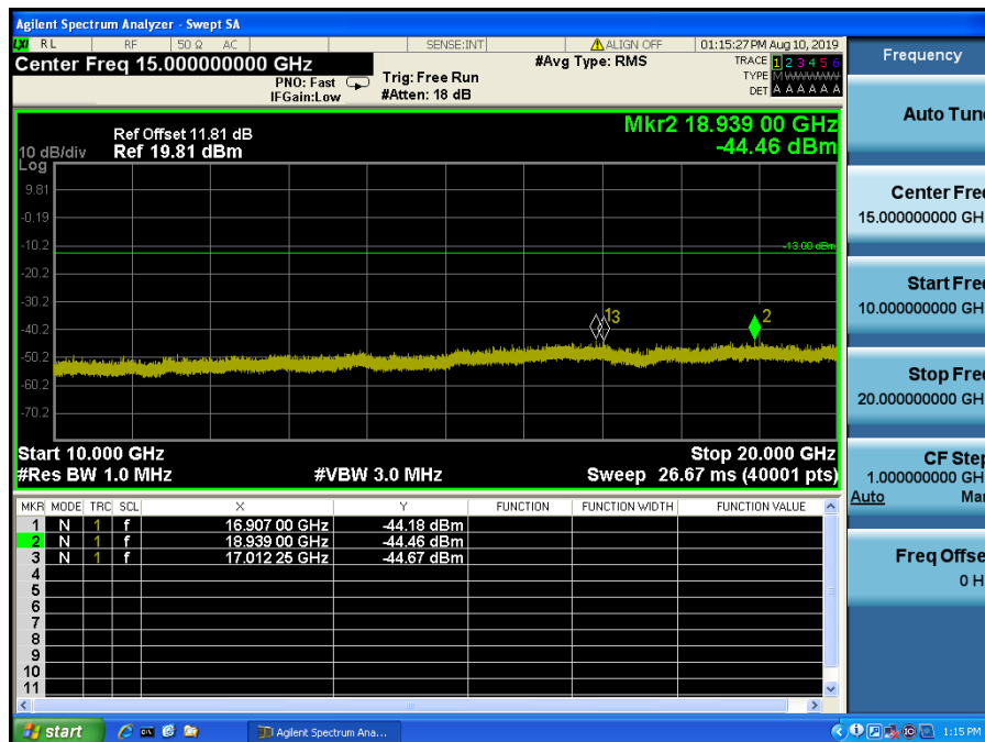
LTE Band 4 / 15MHz / 64QAM - RB Size/Offset (36/0) – Mid Channel
