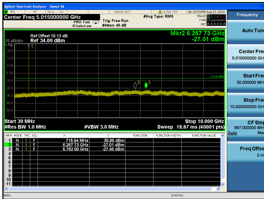
LTE Band 12, 17 / 5MHz / 16QAM - RB Size/Offset (1/24) – High Channel
