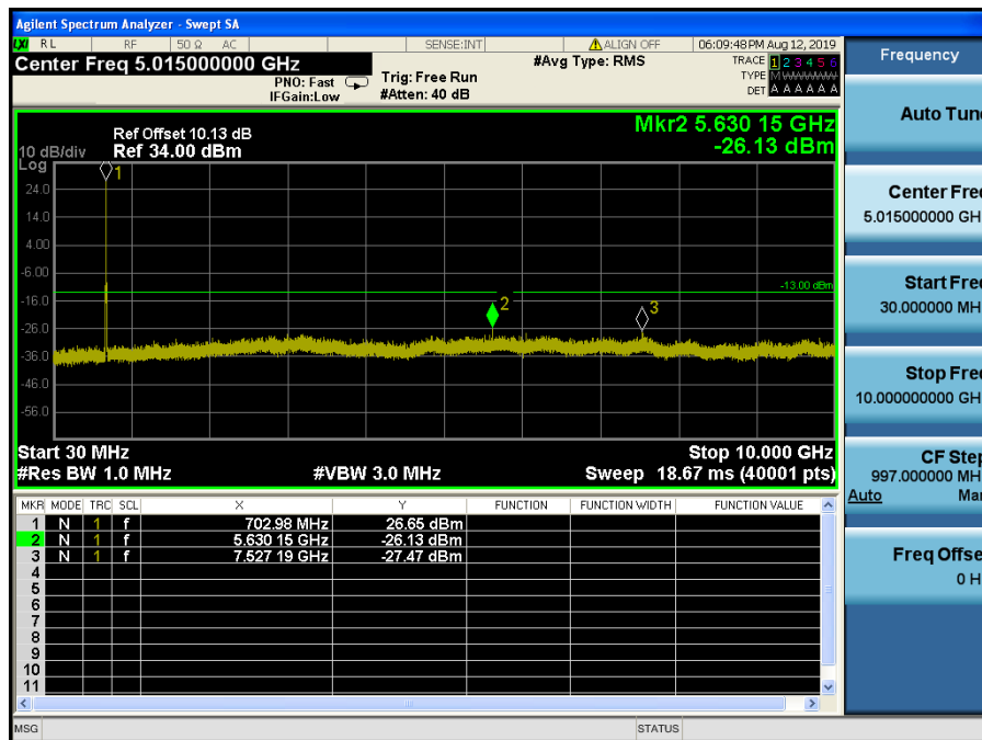
LTE Band 12, 17 / 5MHz / 16QAM - RB Size/Offset (25/0) – Low Channel
