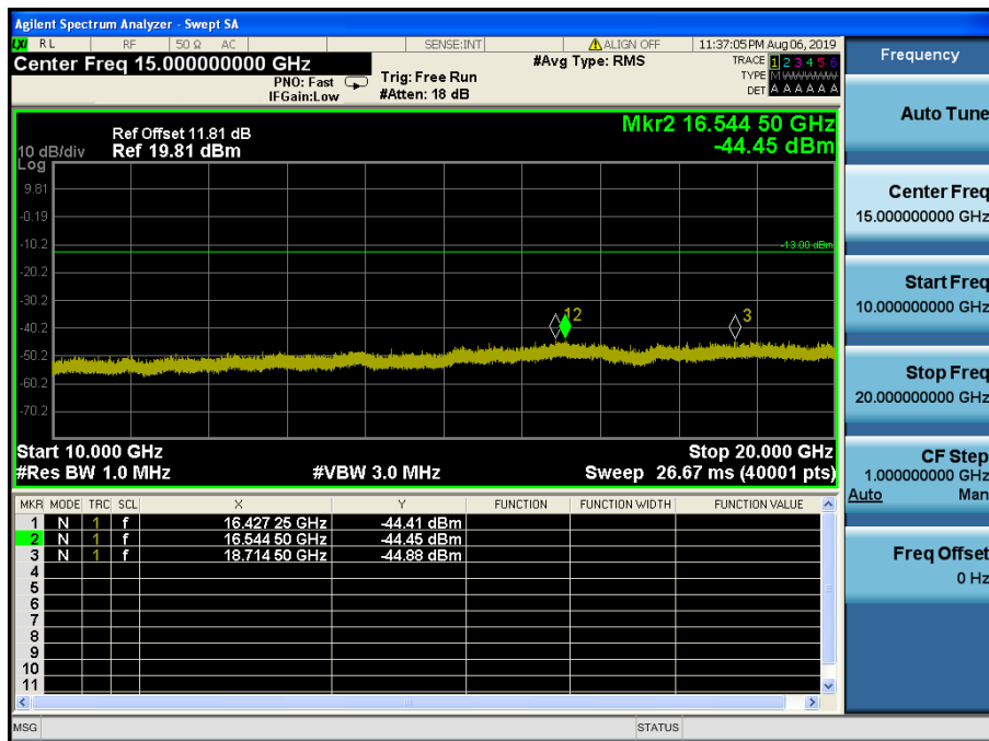
LTE Band 2 / 20MHz / QPSK - RB Size/Offset (50/25) – High Channel
