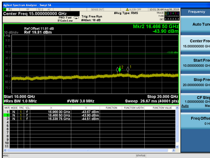
LTE Band 4 / 10MHz / QPSK - RB Size/Offset (25/0) – Low Channel
