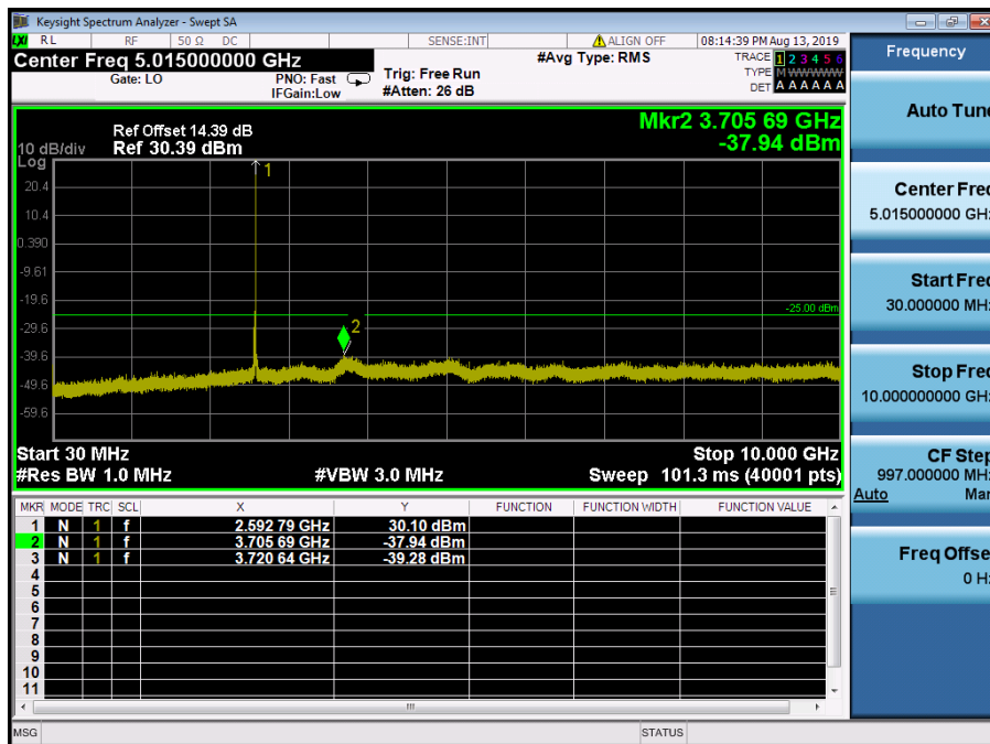
LTE Band 41 / 20MHz / 16QAM - RB Size/Offset (1/50) – Mid Channel
