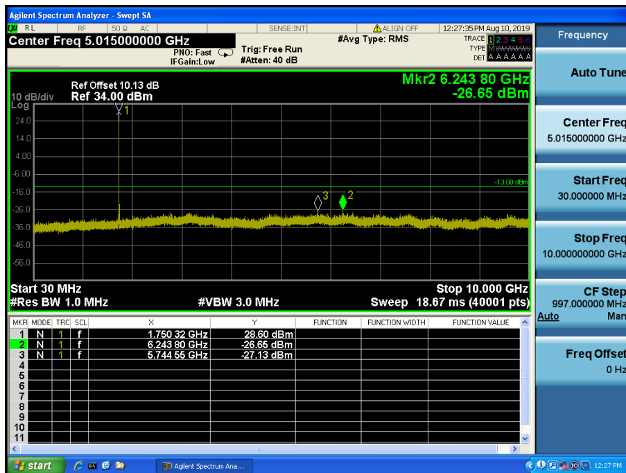
LTE Band 4 / 10MHz / 64QAM - RB Size/Offset (1/25) – High Channel
