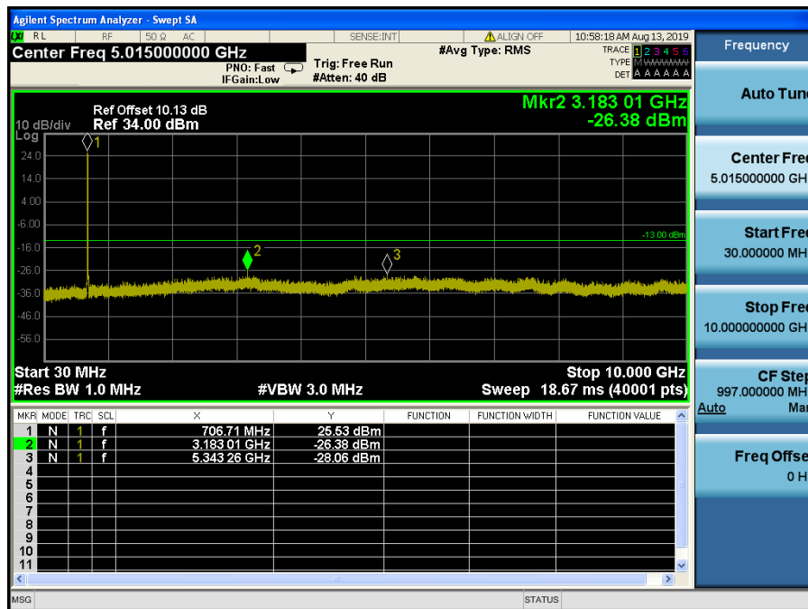
LTE Band 12, 17 / 5MHz / 64QAM - RB Size/Offset (25/0) – Mid Channel
