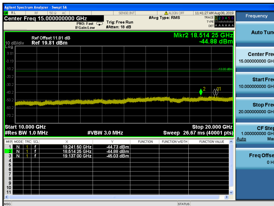
LTE Band 4 / 20MHz / QPSK - RB Size/Offset (1/50)–Mid Channel
