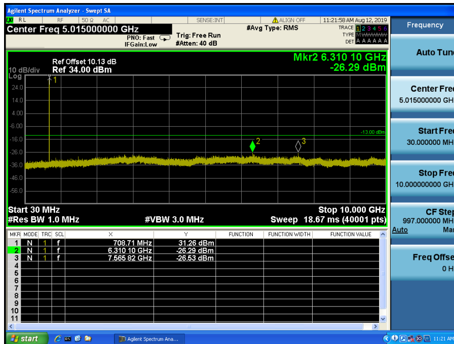
LTE Band 12, 17 / 10MHz / QPSK - RB Size/Offset (1/49) – Low Channel
