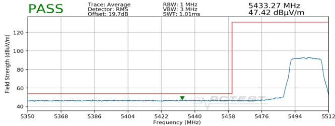
Plot 7-196. Radiated Lower Band Edge Plot SISO ANT2 (Average – UNII Band 2C)
