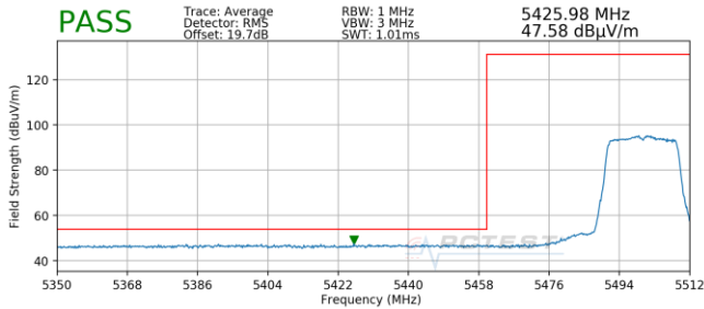
Plot 7-175. Radiated Lower Band Edge Plot SISO ANT1 (Average – UNII Band 2C)
