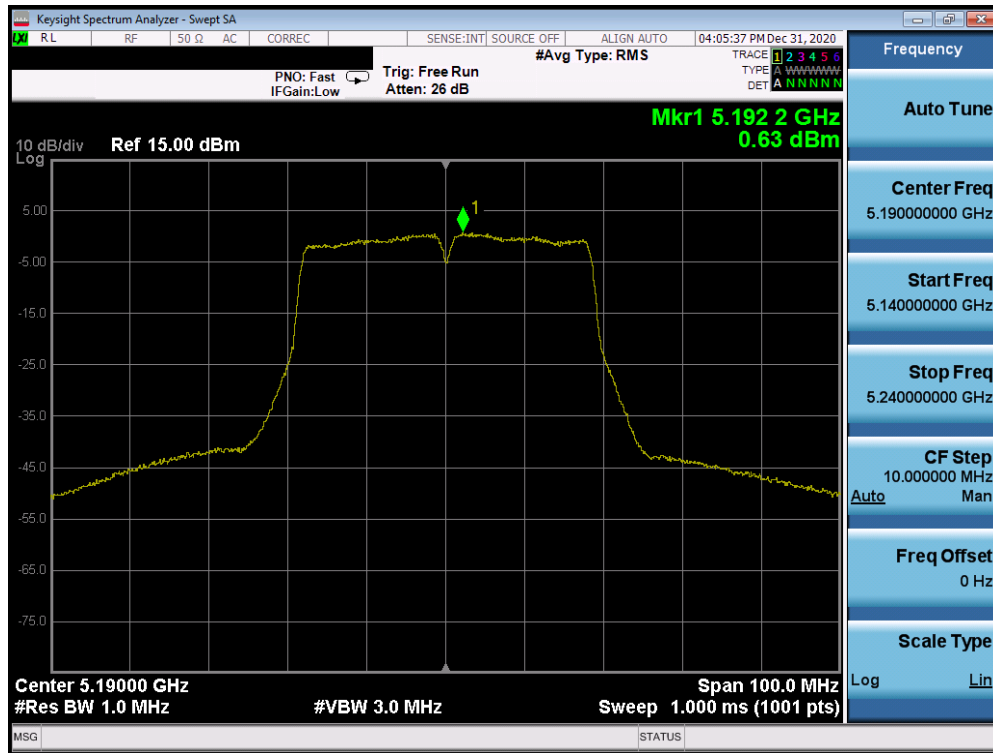
Plot 7-46. Power Spectral Density Plot (40MHz 802.11n (UNII Band 1) – Ch. 38)
