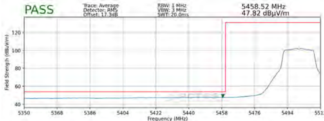
Plot 7-89. Radiated Lower Band Edge Plot (Average – UNII Band 2C)
