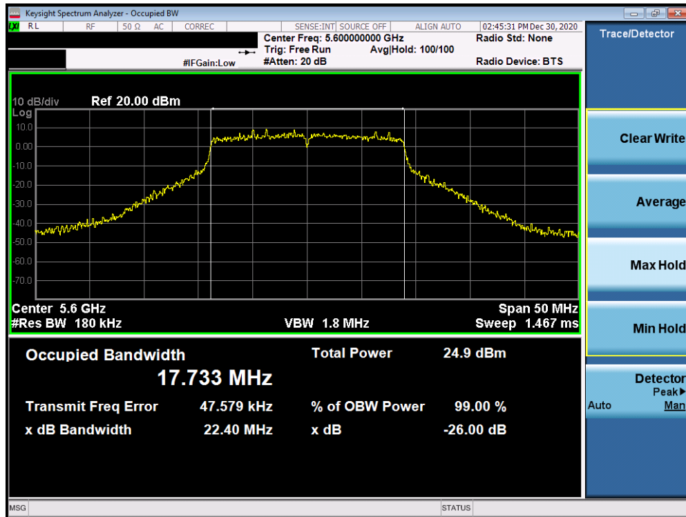
Plot 7-23. 26dB Bandwidth Plot (20MHz 802.11n (UNII Band 2C) – Ch. 120)
