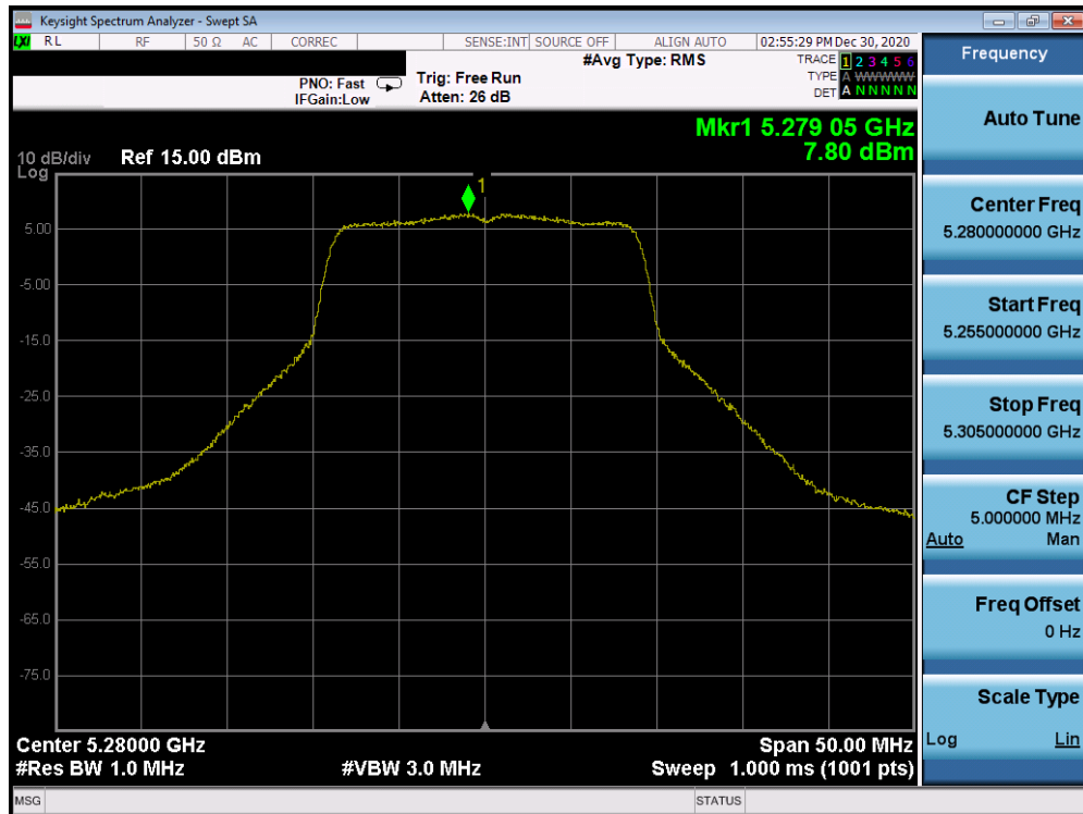
Plot 7-53. Power Spectral Density Plot (20MHz 802.11n (UNII Band 2A) – Ch. 56)
