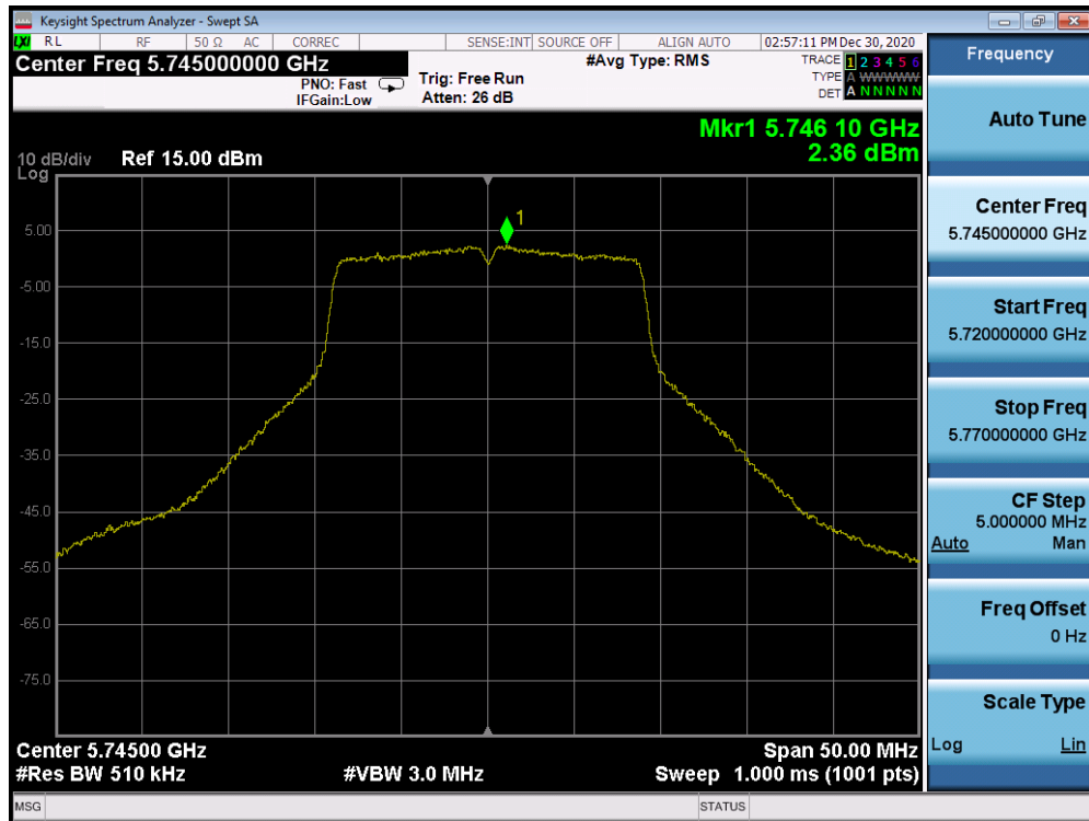
Plot 7-73. Power Spectral Density Plot (20MHz 802.11n (UNII Band 3) – Ch. 149)
