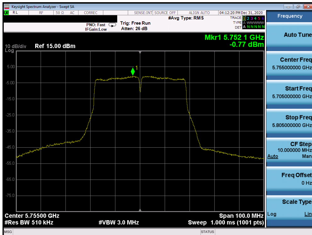
Plot 7-76. Power Spectral Density Plot (40MHz 802.11n (UNII Band 3) – Ch. 151)
