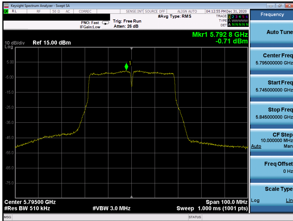
Plot 7-77. Power Spectral Density Plot (40MHz 802.11n (UNII Band 3) – Ch. 159)
