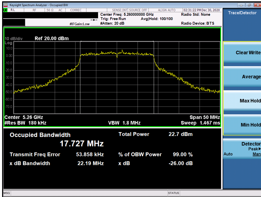
Plot 7-13. 26dB Bandwidth Plot (20MHz 802.11n (UNII Band 2A) – Ch. 52)
