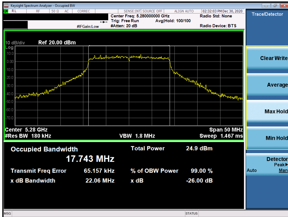
Plot 7-14. 26dB Bandwidth Plot (20MHz 802.11n (UNII Band 2A) – Ch. 56)
