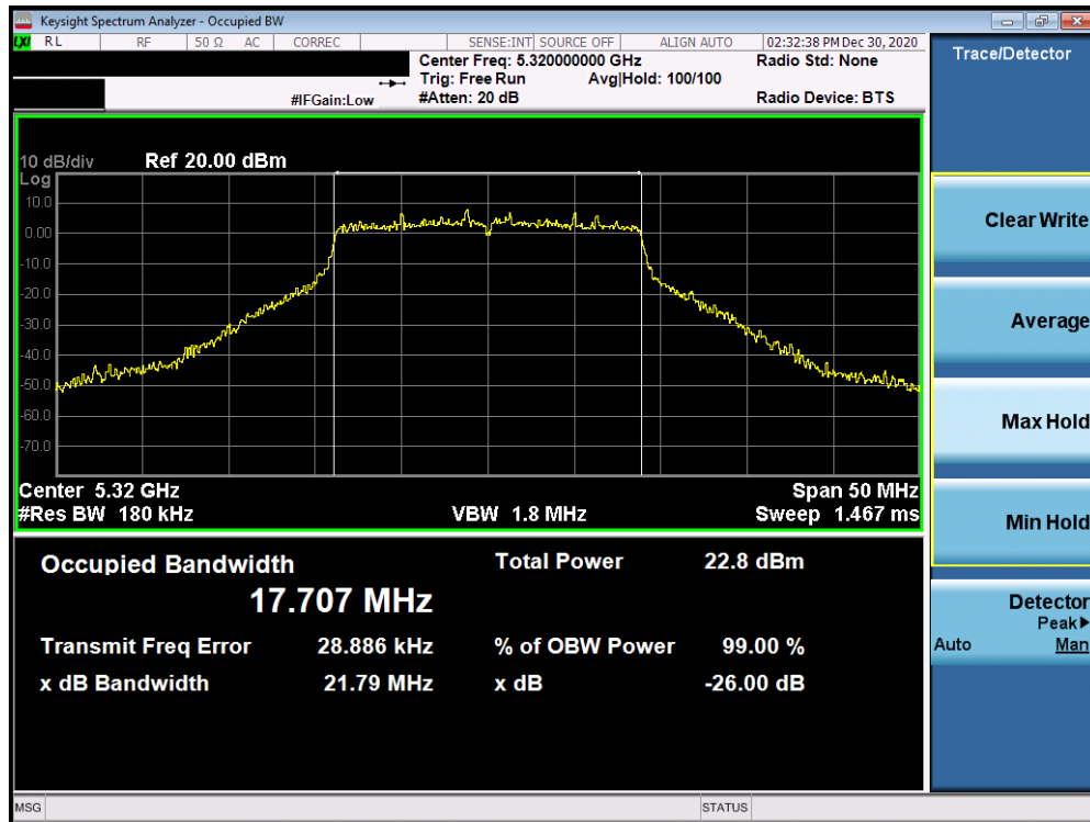
Plot 7-15. 26dB Bandwidth Plot (20MHz 802.11n (UNII Band 2A) – Ch. 64)
