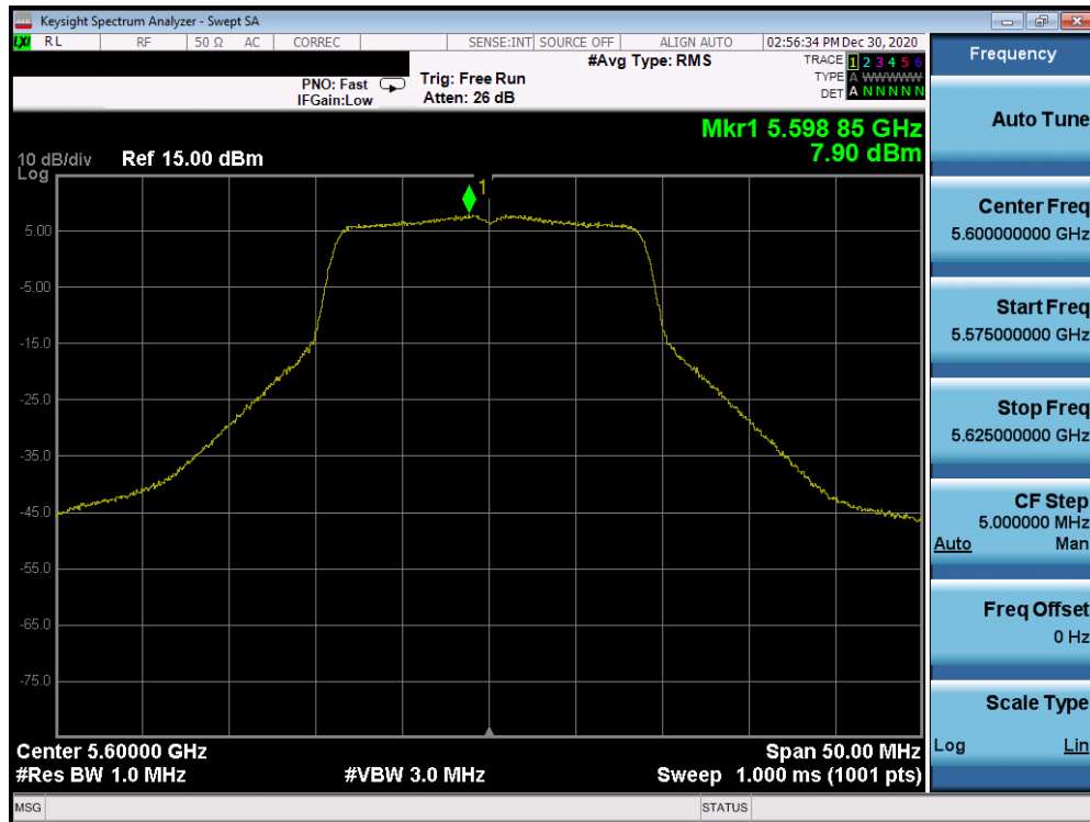
Plot 7-62. Power Spectral Density Plot (20MHz 802.11n (UNII Band 2C) – Ch. 120)
