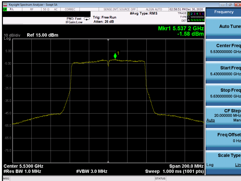
Plot 7-67. Power Spectral Density Plot (80MHz 802.11ac (UNII Band 2C) – Ch. 106)
