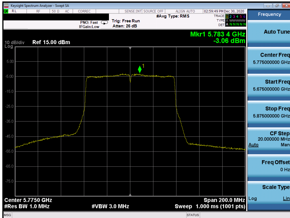
Plot 7-78. Power Spectral Density Plot (80MHz 802.11ac (UNII Band 3) – Ch. 155)
