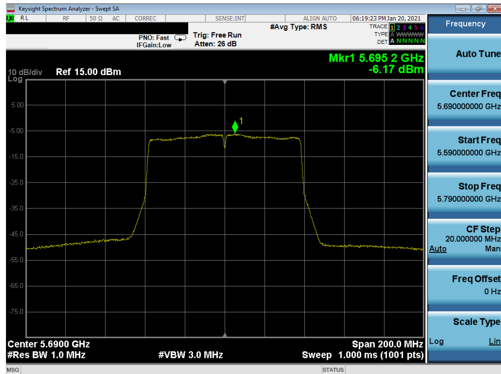
Plot 7-69. Power Spectral Density Plot (80MHz 802.11ac (UNII Band 2C) – Ch. 138)
