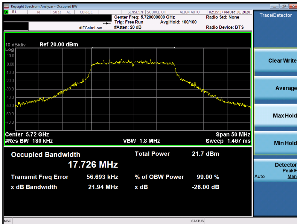
Plot 7-24. 26dB Bandwidth Plot (20MHz 802.11n (UNII Band 2C) – Ch. 144)
