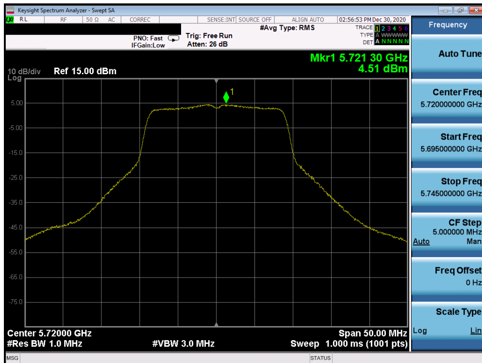
Plot 7-63. Power Spectral Density Plot (20MHz 802.11n (UNII Band 2C) – Ch. 144)
