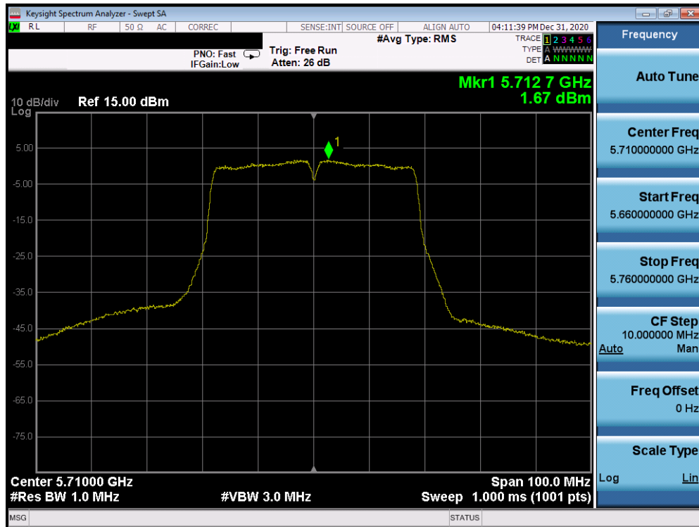
Plot 7-66. Power Spectral Density Plot (40MHz 802.11n (UNII Band 2C) – Ch. 142)
