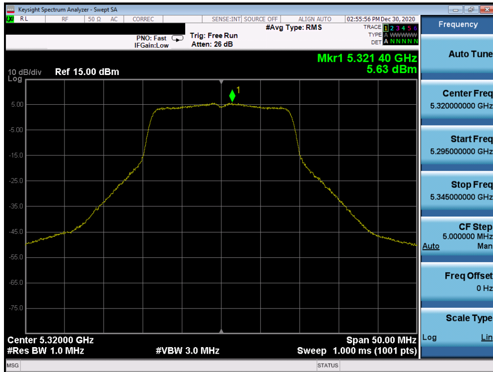
Plot 7-54. Power Spectral Density Plot (20MHz 802.11n (UNII Band 2A) – Ch. 64)
