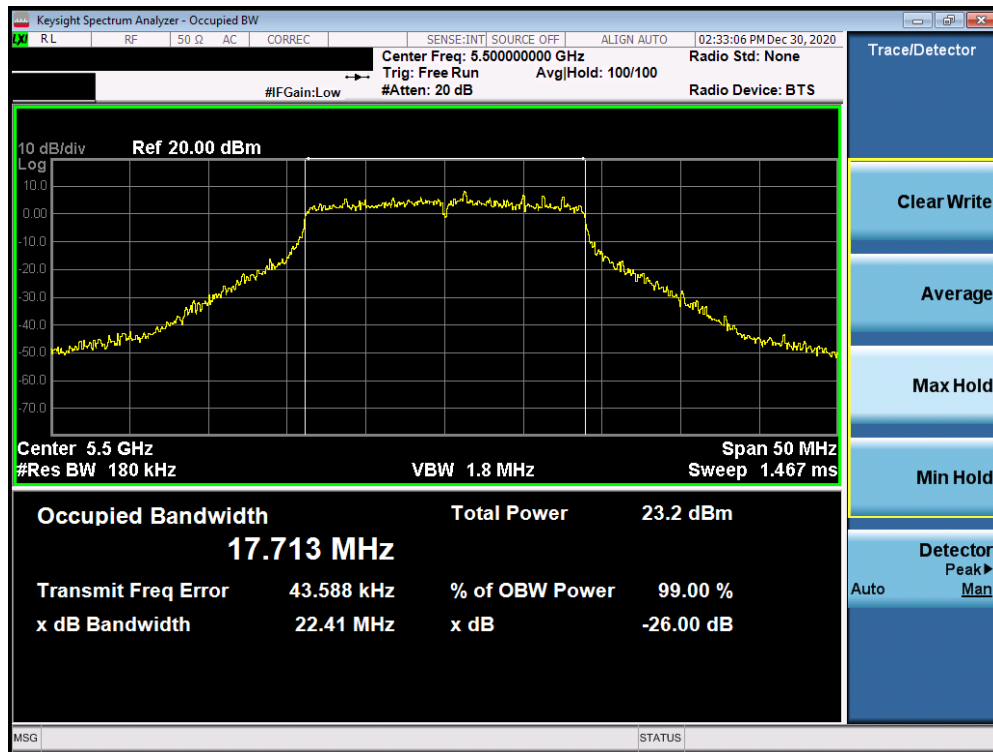
Plot 7-22. 26dB Bandwidth Plot (20MHz 802.11n (UNII Band 2C) – Ch. 100)
