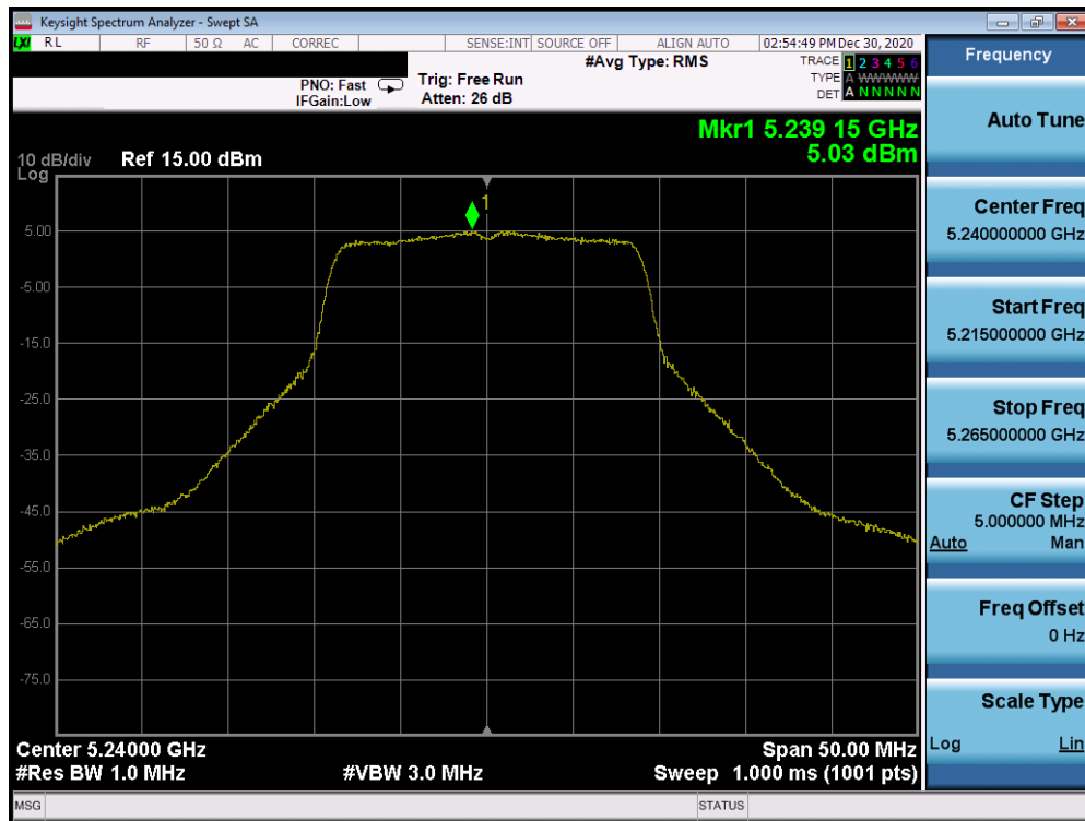
Plot 7-45. Power Spectral Density Plot (20MHz 802.11n (UNII Band 1) – Ch. 48)
