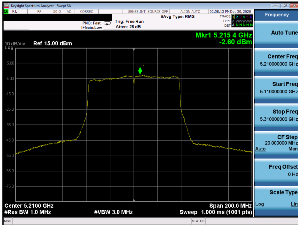
Plot 7-48. Power Spectral Density Plot (80MHz 802.11ac (UNII Band 1) – Ch. 42)
