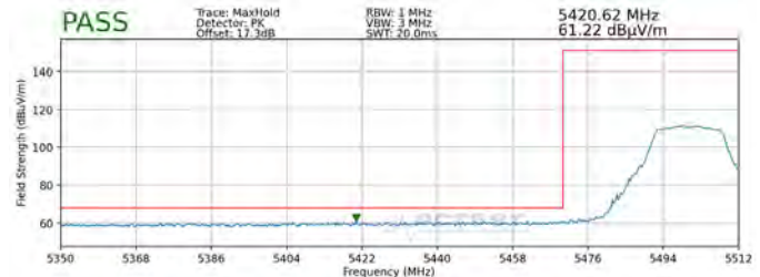
Plot 7-90. Radiated Lower Band Edge Plot (Peak – UNII Band 2C)
