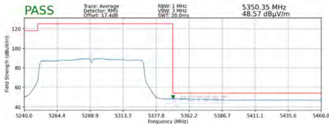
Plot 7-101. Radiated Upper Band Edge Plot (Average – UNII Band 2A)
