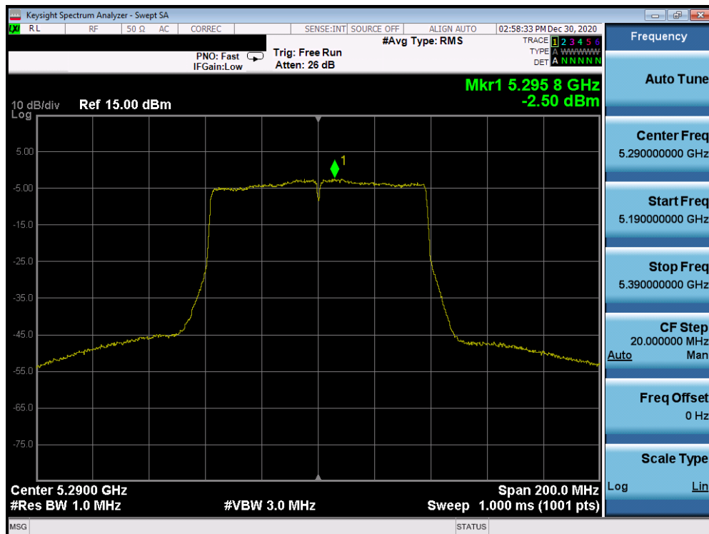
Plot 7-57. Power Spectral Density Plot (80MHz 802.11ac (UNII Band 2A) – Ch. 58)
