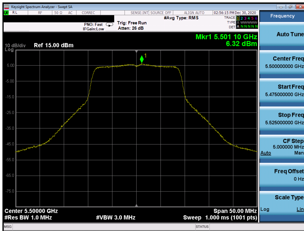
Plot 7-61. Power Spectral Density Plot (20MHz 802.11n (UNII Band 2C) – Ch. 100)
