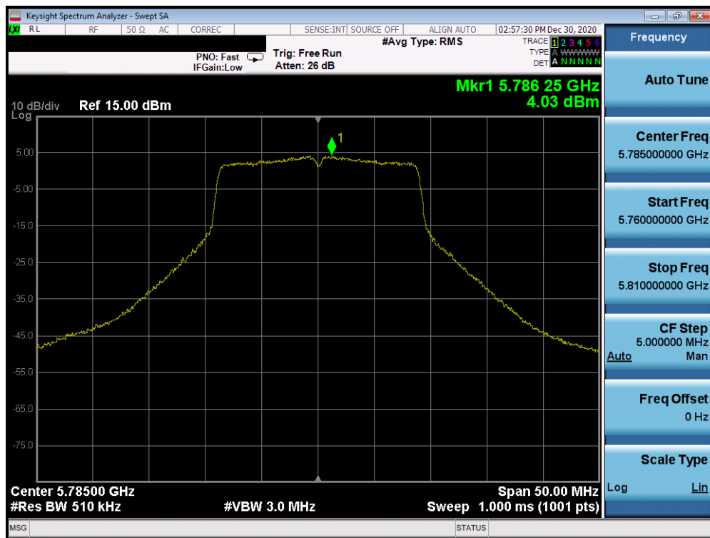
Plot 7-74. Power Spectral Density Plot (20MHz 802.11n (UNII Band 3) – Ch. 157)
