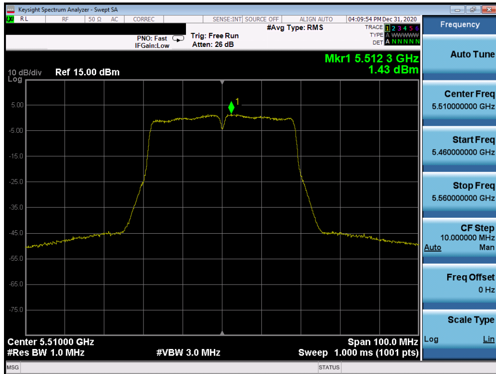
Plot 7-64. Power Spectral Density Plot (40MHz 802.11n (UNII Band 2C) – Ch. 102)
