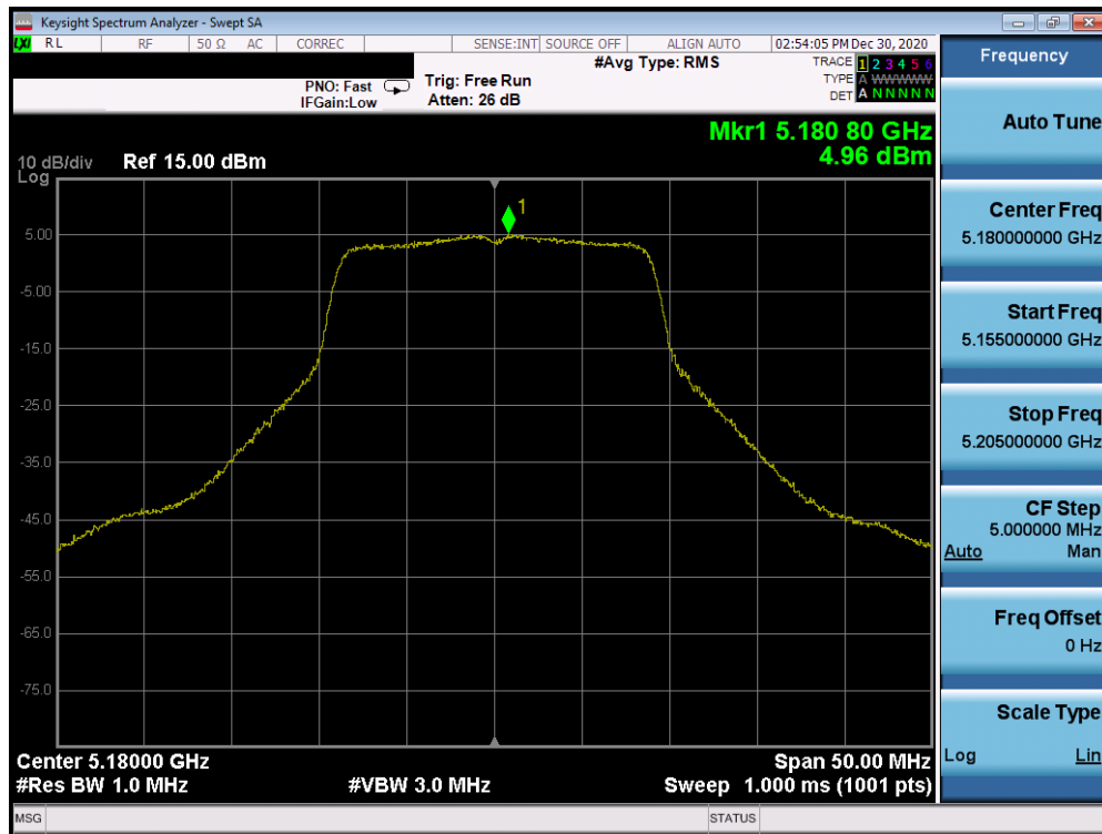
Plot 7-43. Power Spectral Density Plot (20MHz 802.11n (UNII Band 1) – Ch. 36)
