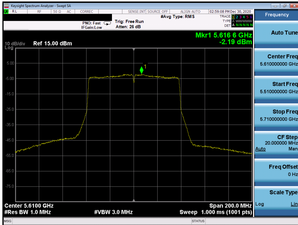
Plot 7-68. Power Spectral Density Plot (80MHz 802.11ac (UNII Band 2C) – Ch. 122)
