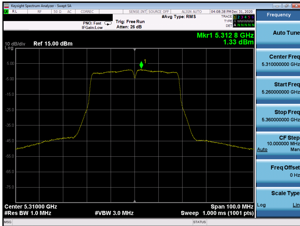
Plot 7-56. Power Spectral Density Plot (40MHz 802.11n (UNII Band 2A) – Ch. 62)
