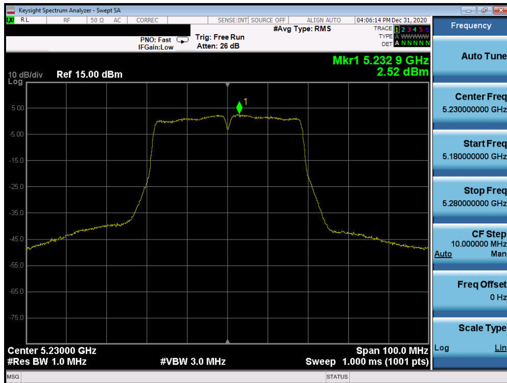
Plot 7-47. Power Spectral Density Plot (40MHz 802.11n (UNII Band 1) – Ch. 46)
