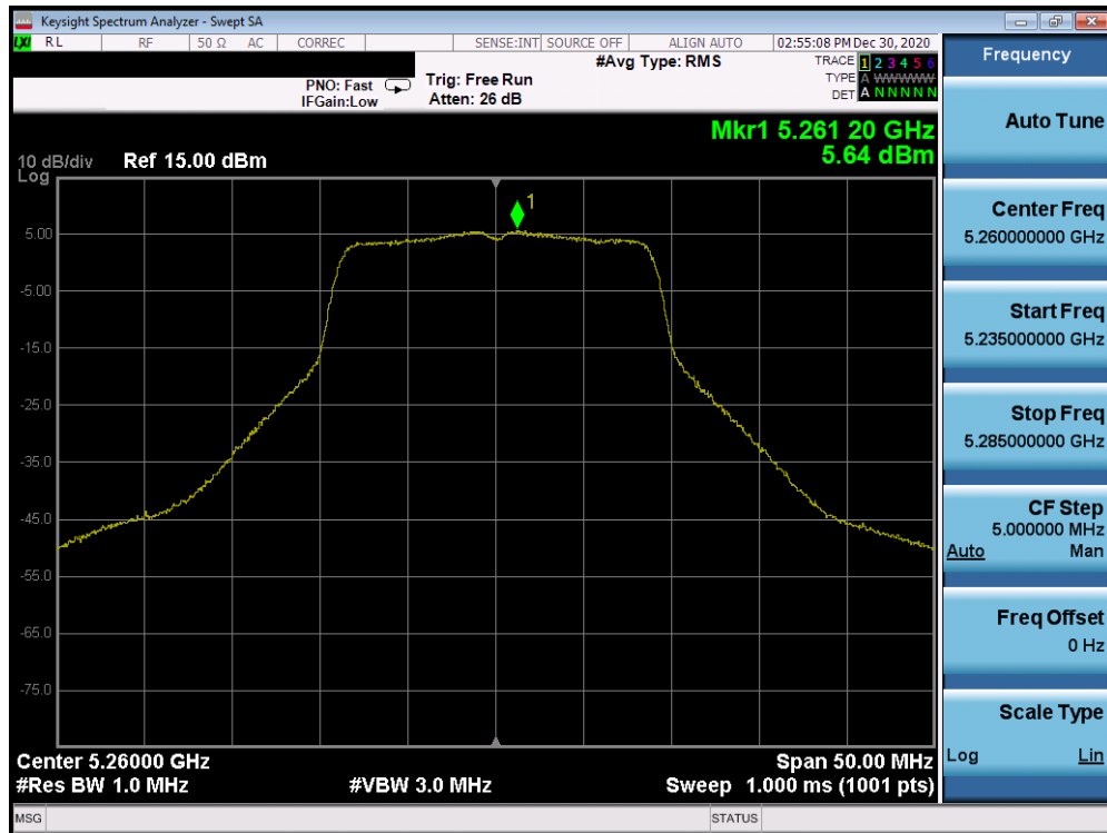
Plot 7-52. Power Spectral Density Plot (20MHz 802.11n (UNII Band 2A) – Ch. 52)
