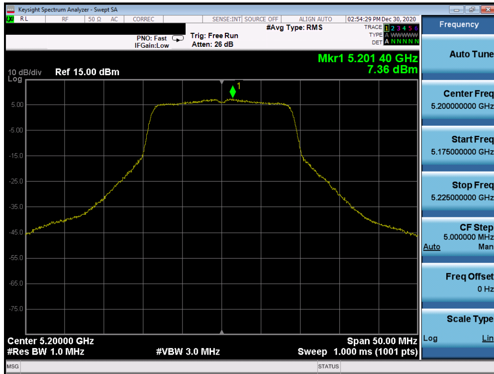
Plot 7-44. Power Spectral Density Plot (20MHz 802.11n (UNII Band 1) – Ch. 40)
