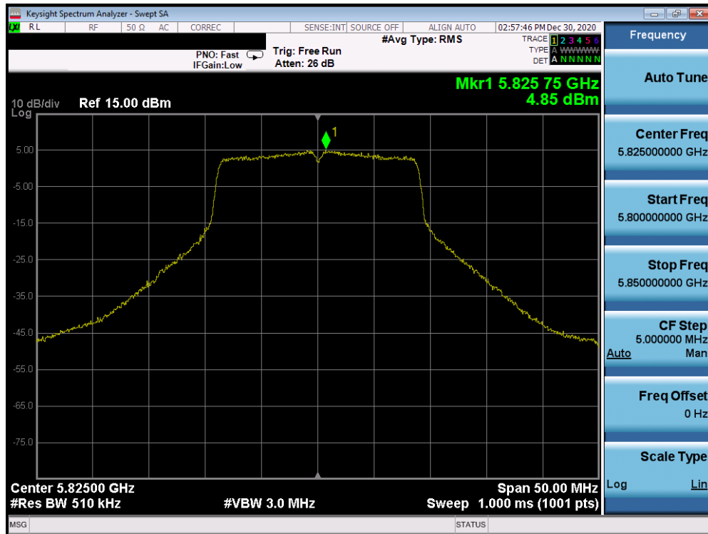
Plot 7-75. Power Spectral Density Plot (20MHz 802.11n (UNII Band 3) – Ch. 165)
