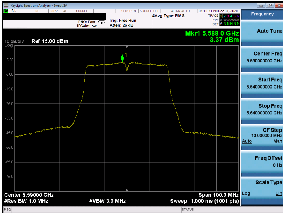
Plot 7-65. Power Spectral Density Plot (40MHz 802.11n (UNII Band 2C) – Ch. 118)
