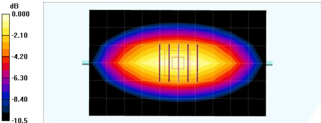
0 dB = 1.14mW/g
