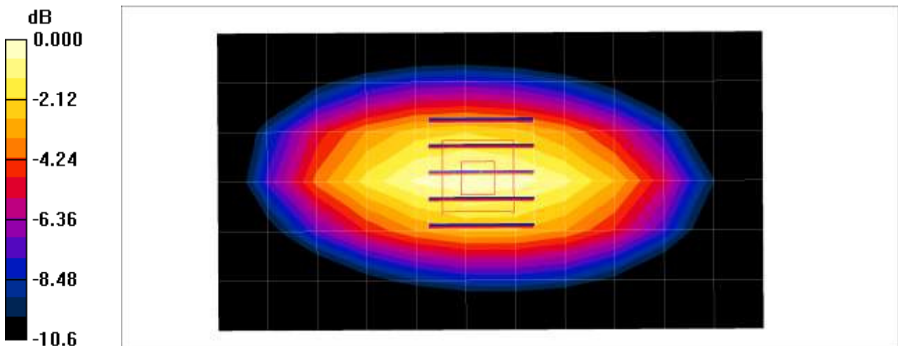
0 dB = 1.01mW/g
