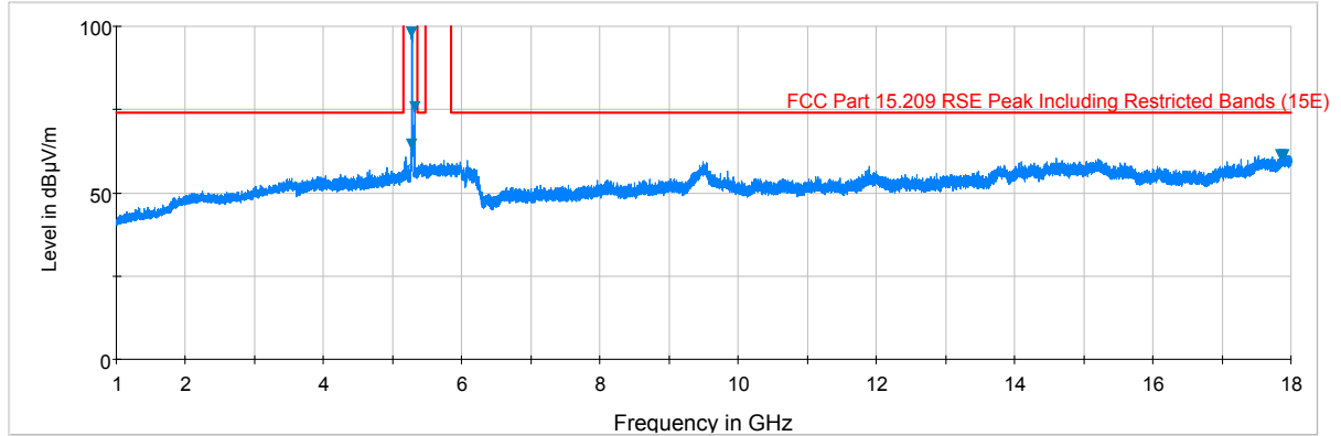
Plot 7-78. Radiated Spurious Plot above 1GHz (802.11a – U2A Ch. 56, Ant. Pol. V)
