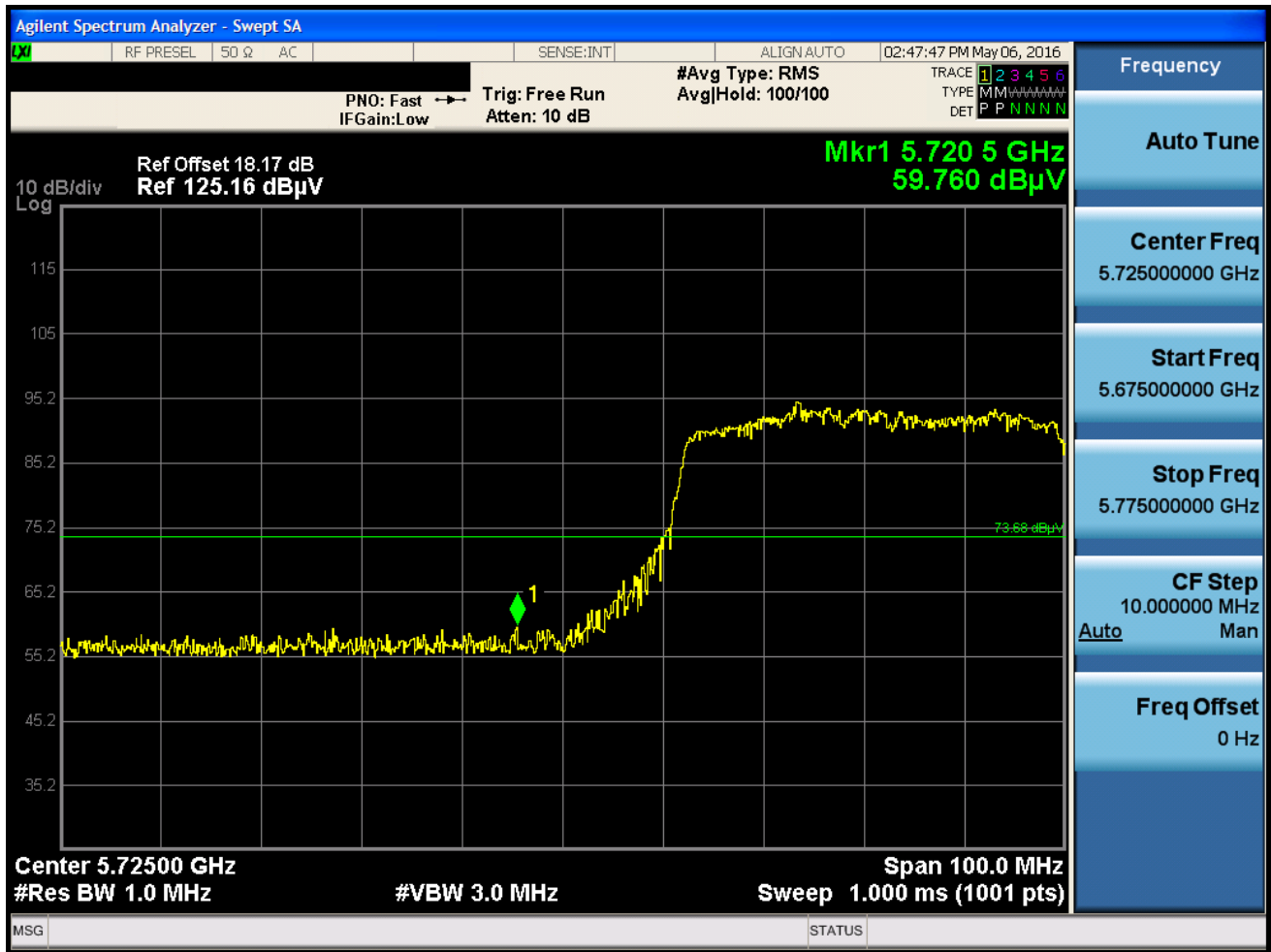
Plot 7-116. Radiated Restricted Lower Band Edge Plot (Peak – UNII Band 3)
