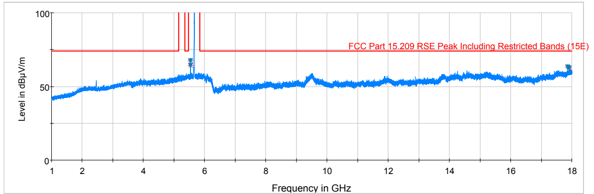
Plot 7-79. Radiated Spurious Plot above 1GHz (802.11a – U2C Ch. 116, Ant. Pol. H)
