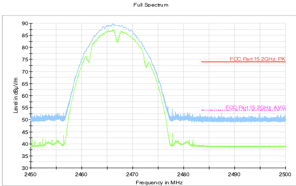
Fig.A.6.2.4 Transmitter Spurious Emission - Radiated (Power): 802.11b, ch12, 2.45 GHz - 2.50GHz
