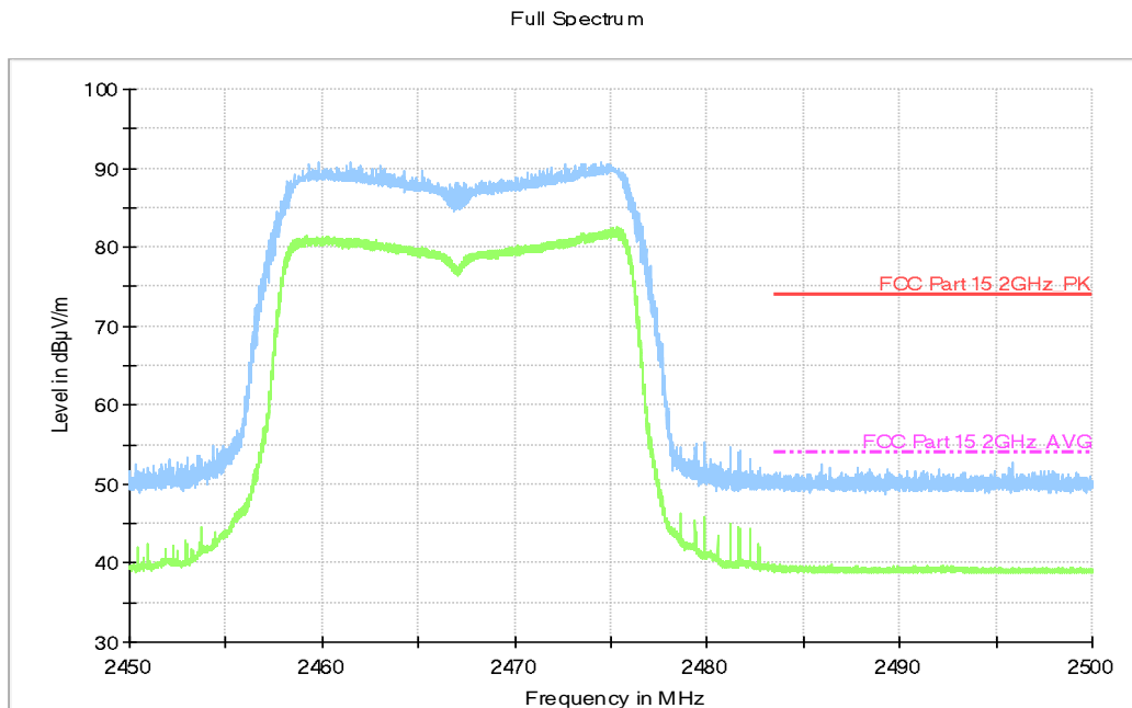
Fig.A.6.2.14 Transmitter Spurious Emission - Radiated (Power): 802.11n-HT20, ch12, 2.45 GHz - 2.50GHz
