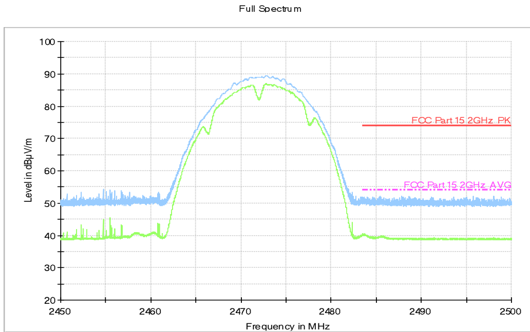
Fig.A.6.2.5 Transmitter Spurious Emission - Radiated (Power): 802.11b, ch13, 2.45 GHz - 2.50GHz
