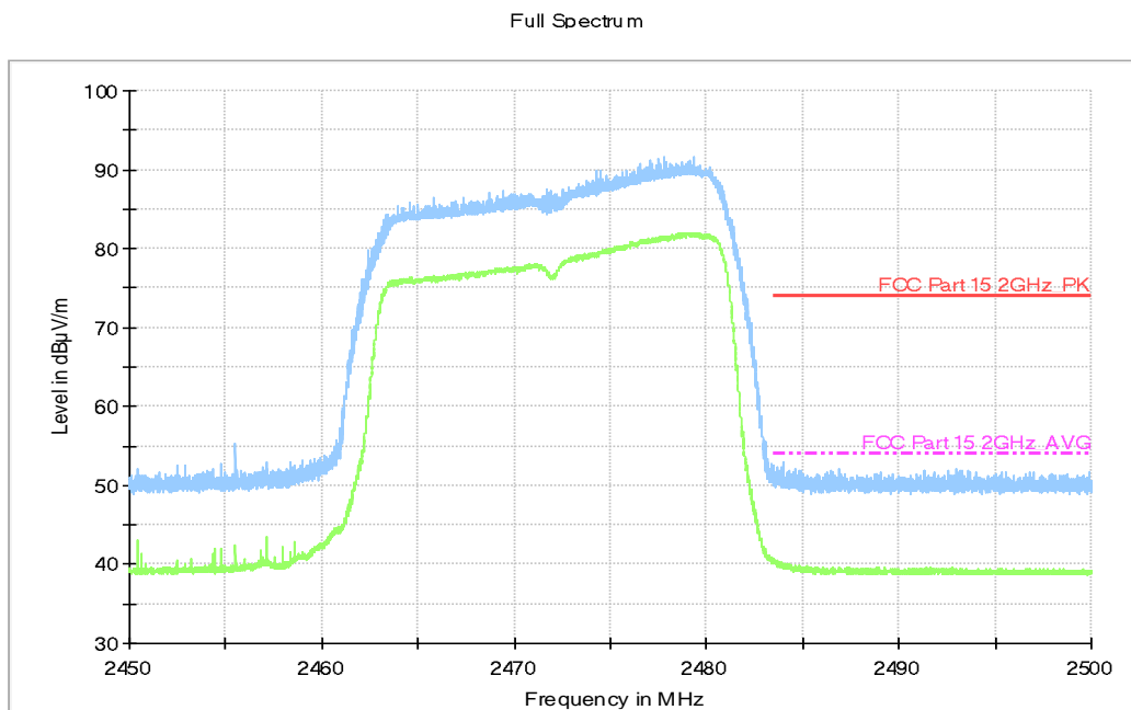
Fig.A.6.2.15 Transmitter Spurious Emission - Radiated (Power): 802.11n-HT20, ch13, 2.45 GHz - 2.50GHz
