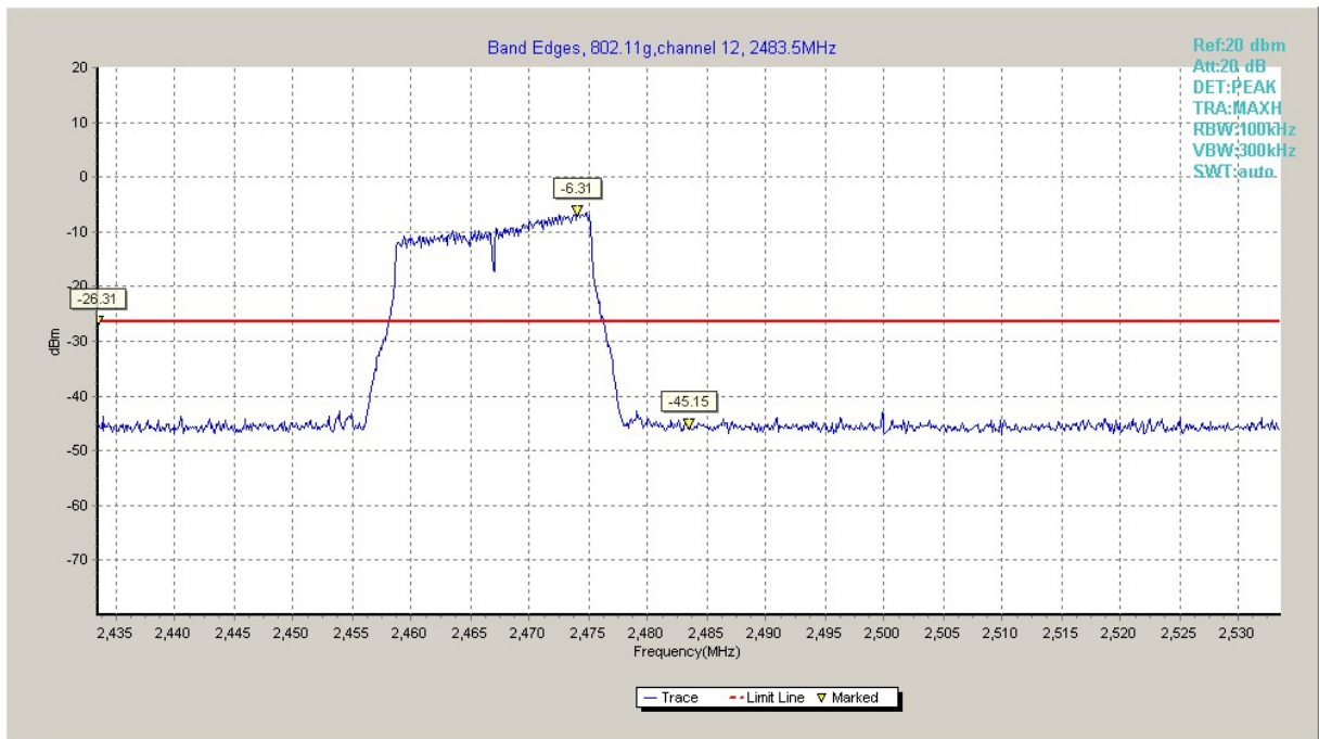
Fig.A.5.7 Band Edges (802.11g, Ch 12)
