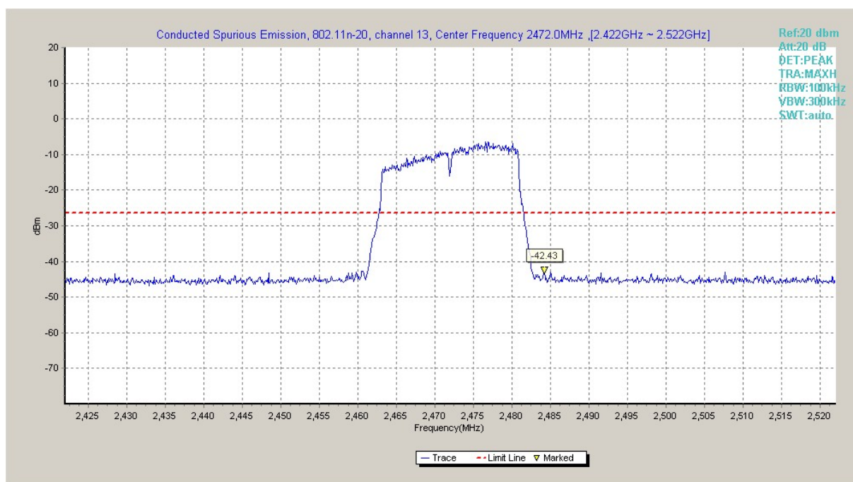
Fig.A.6.1.113 Transmitter Spurious Emission - Conducted (802.11n-HT20, Ch13, Center Frequency)
