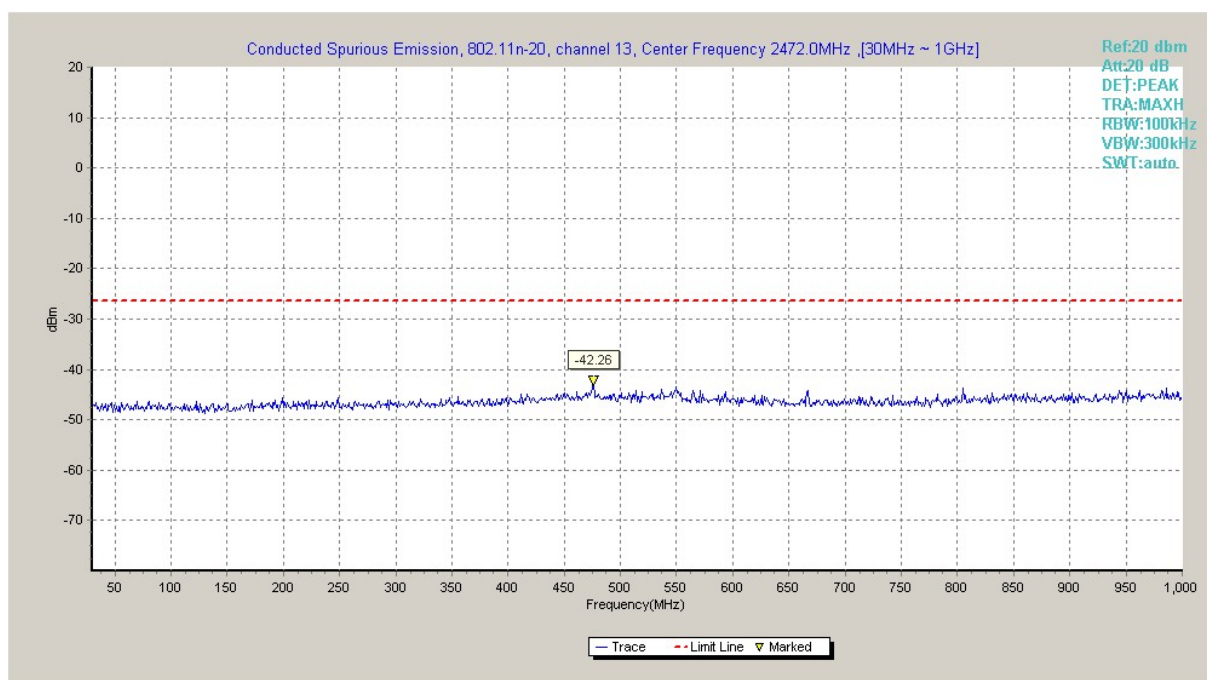
Fig.A.6.1.114 Transmitter Spurious Emission - Conducted (802.11n-HT20, Ch13, 30 MHz-1 GHz)
