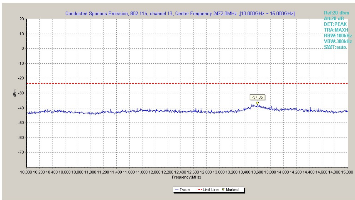
Fig.A.6.1.38 Transmitter Spurious Emission - Conducted (802.11b, Ch13, 10 GHz-15 GHz)
