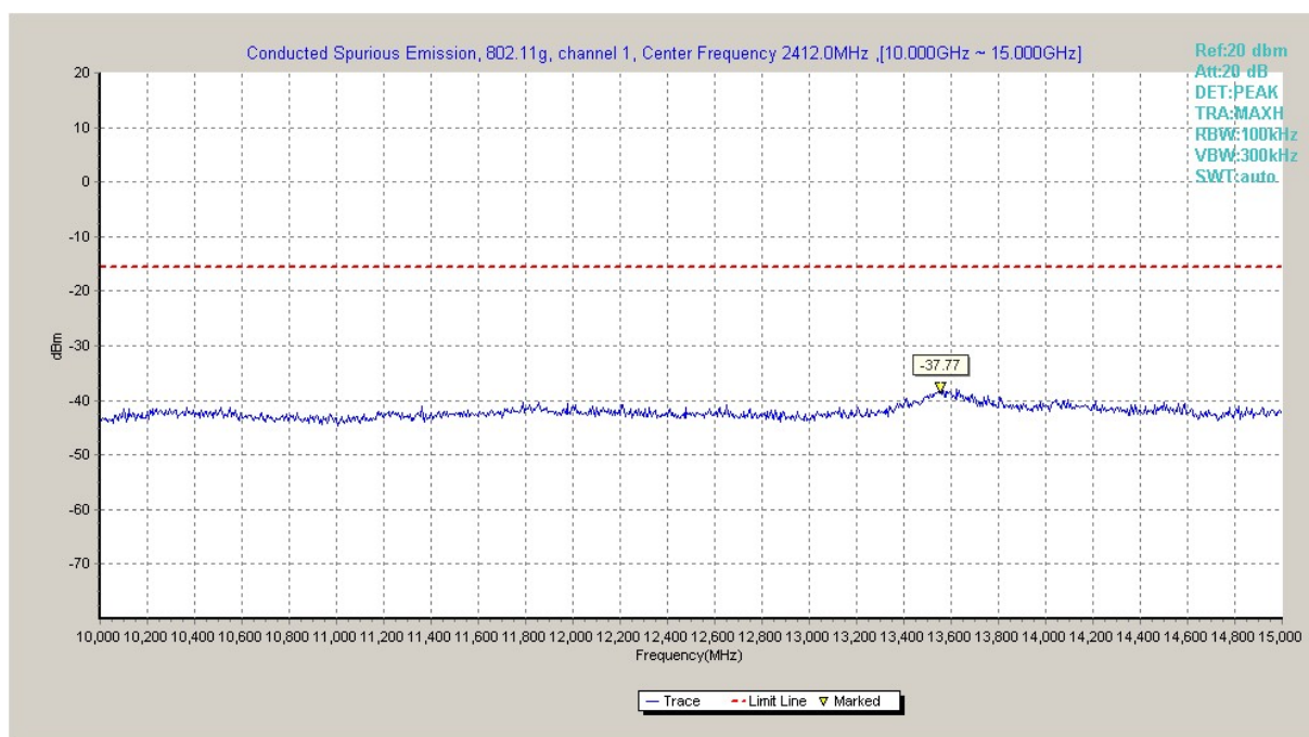
Fig.A.6.1.46 Transmitter Spurious Emission - Conducted (802.11g, Ch1, 10 GHz-15 GHz)
