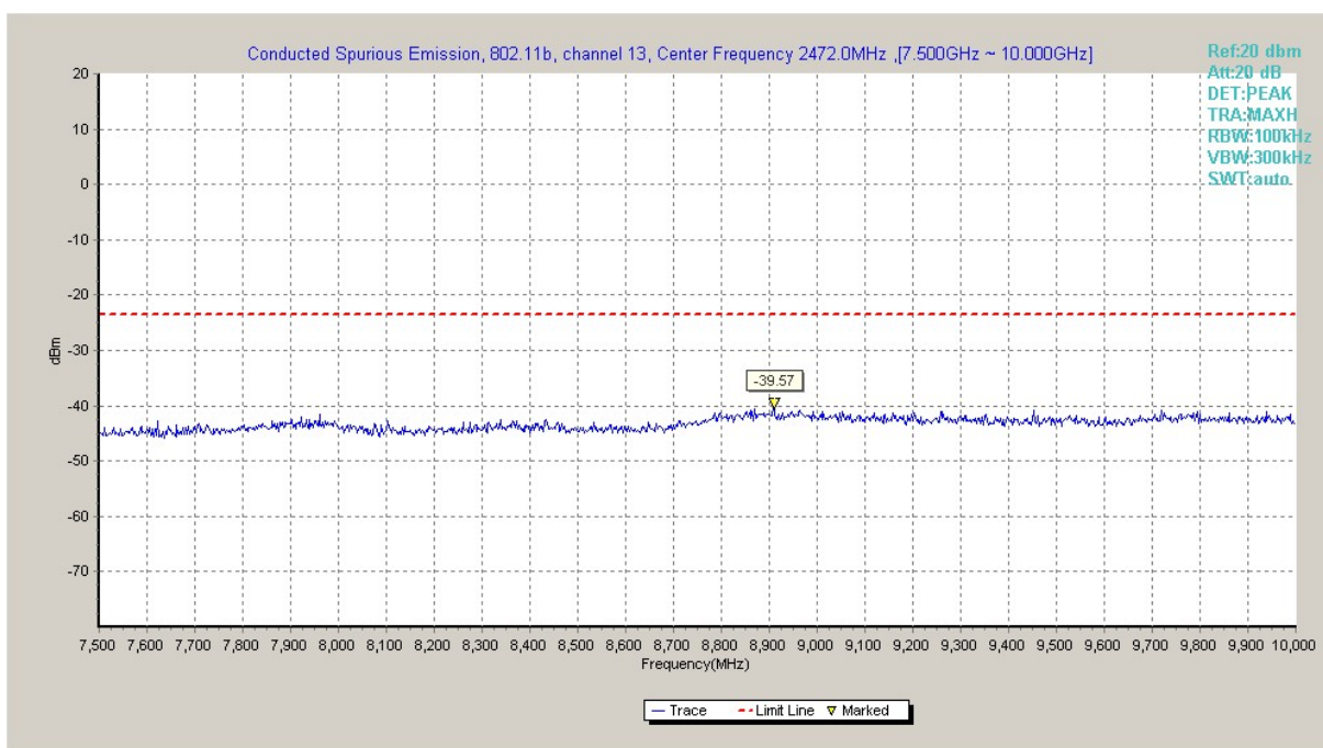
Fig.A.6.1.37 Transmitter Spurious Emission - Conducted (802.11b, Ch13, 7.5 GHz-10 GHz)
