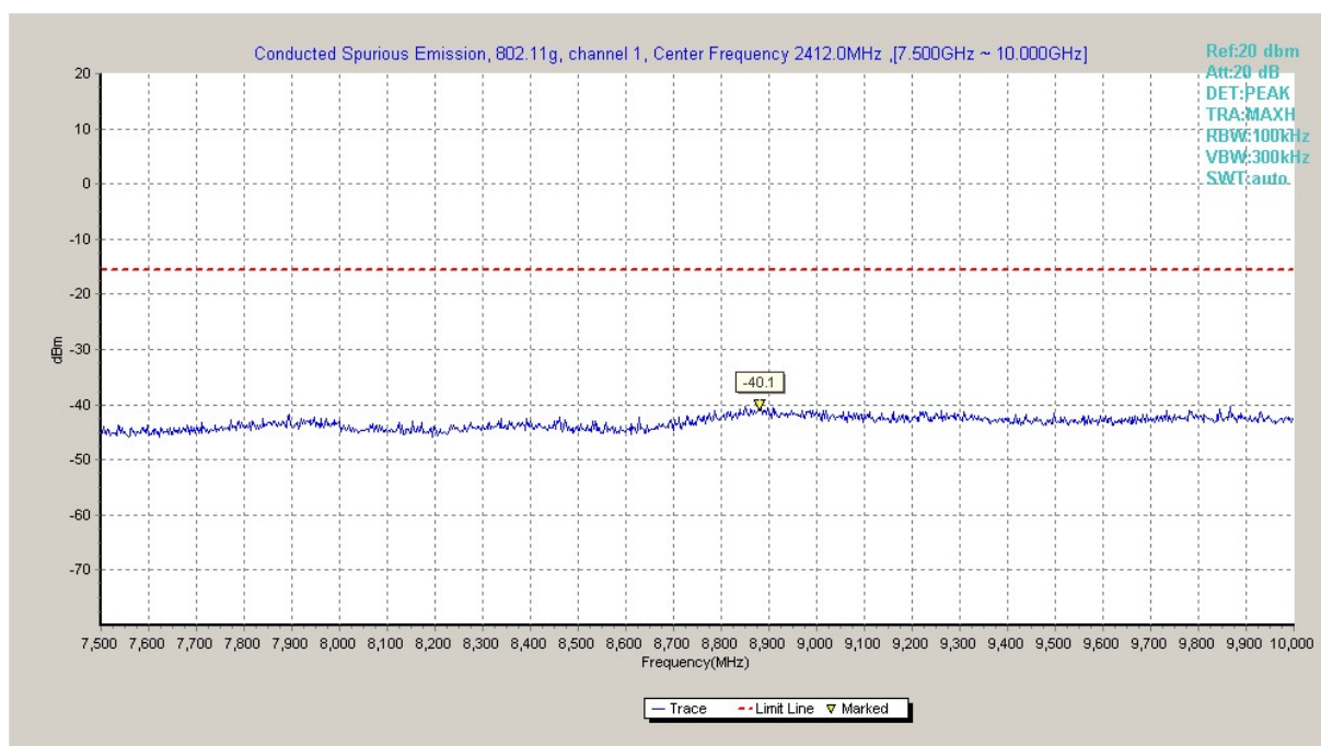
Fig.A.6.1.45 Transmitter Spurious Emission - Conducted (802.11g, Ch1, 7.5 GHz-10 GHz)
