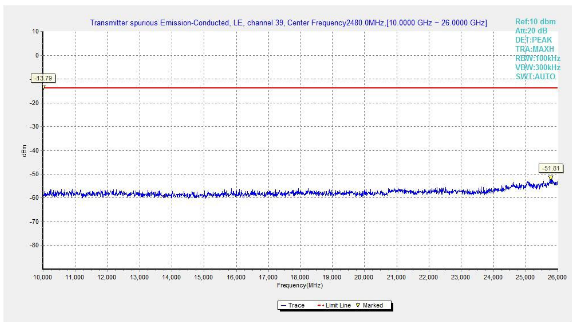
Fig.19. Transmitter Spurious Emission - Conducted: GFSK, 2480 MHz, 10GHz - 26GHz
