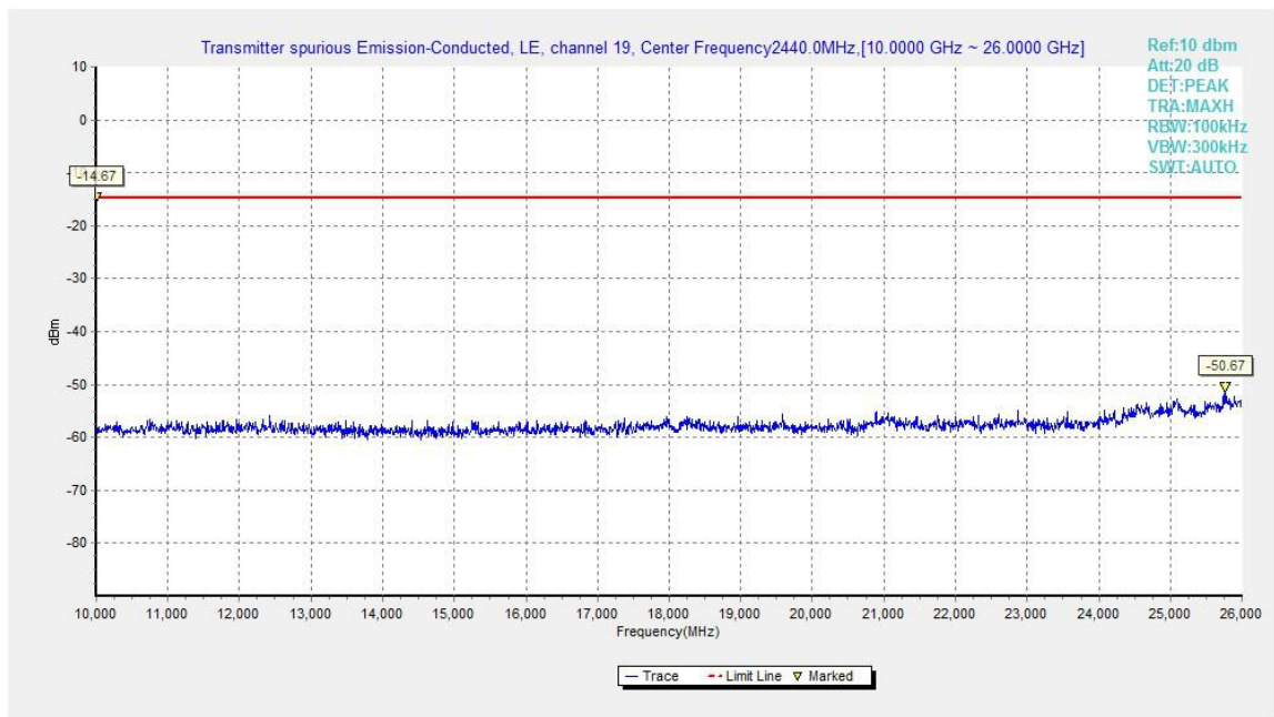
Fig.14. Transmitter Spurious Emission - Conducted: GFSK, 2440 MHz, 10GHz – 26GHz
