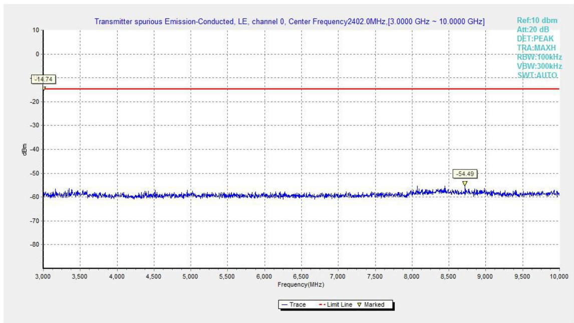
Fig.8. Transmitter Spurious Emission - Conducted: GFSK, 2402 MHz, 3GHz - 10GHz
