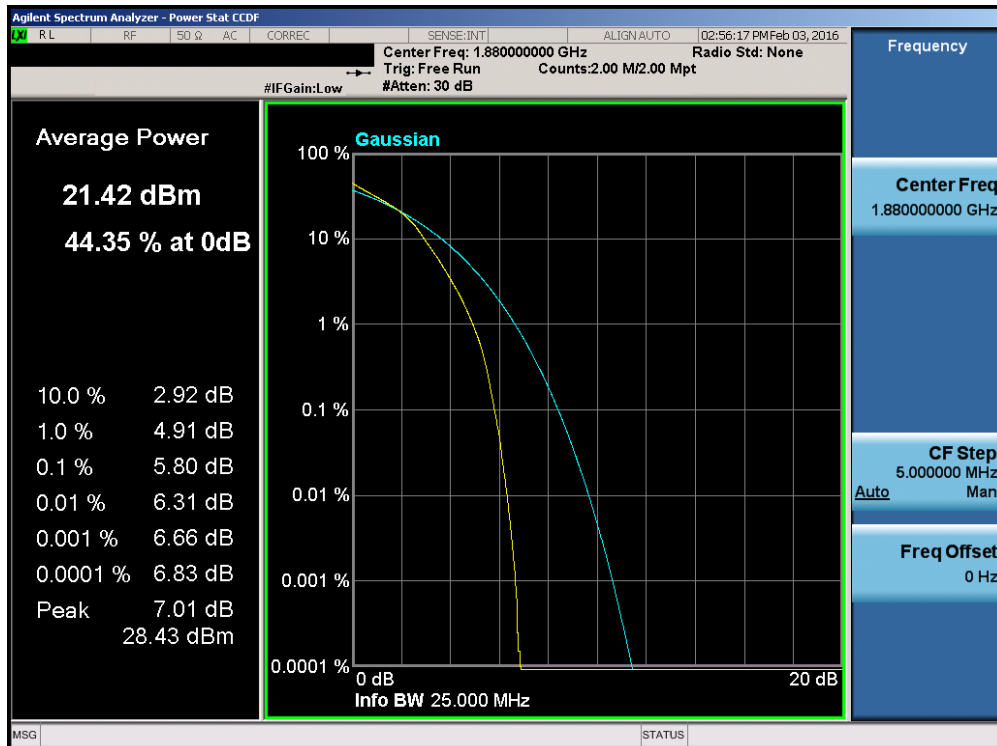
Plot 7-126. PAR Plot (Band 2 – 20.0MHz 16-QAM – RB Size 100)
