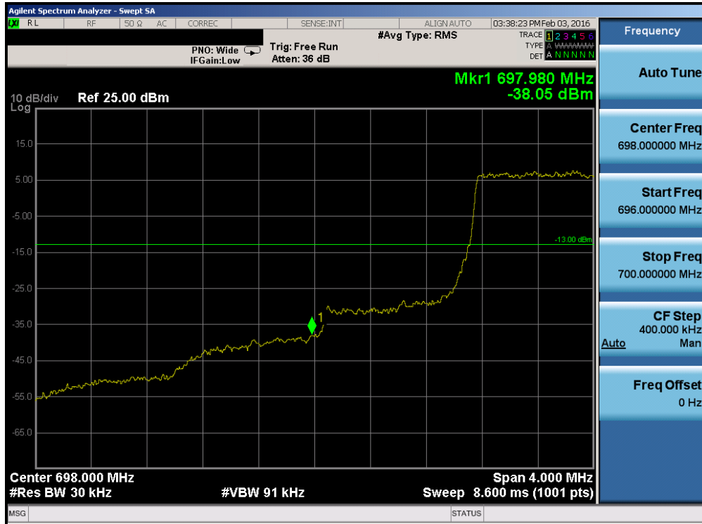
Plot 7-51. Lower Band Edge Plot (Band 12 – 1.4MHz QPSK – RB Size 6)
