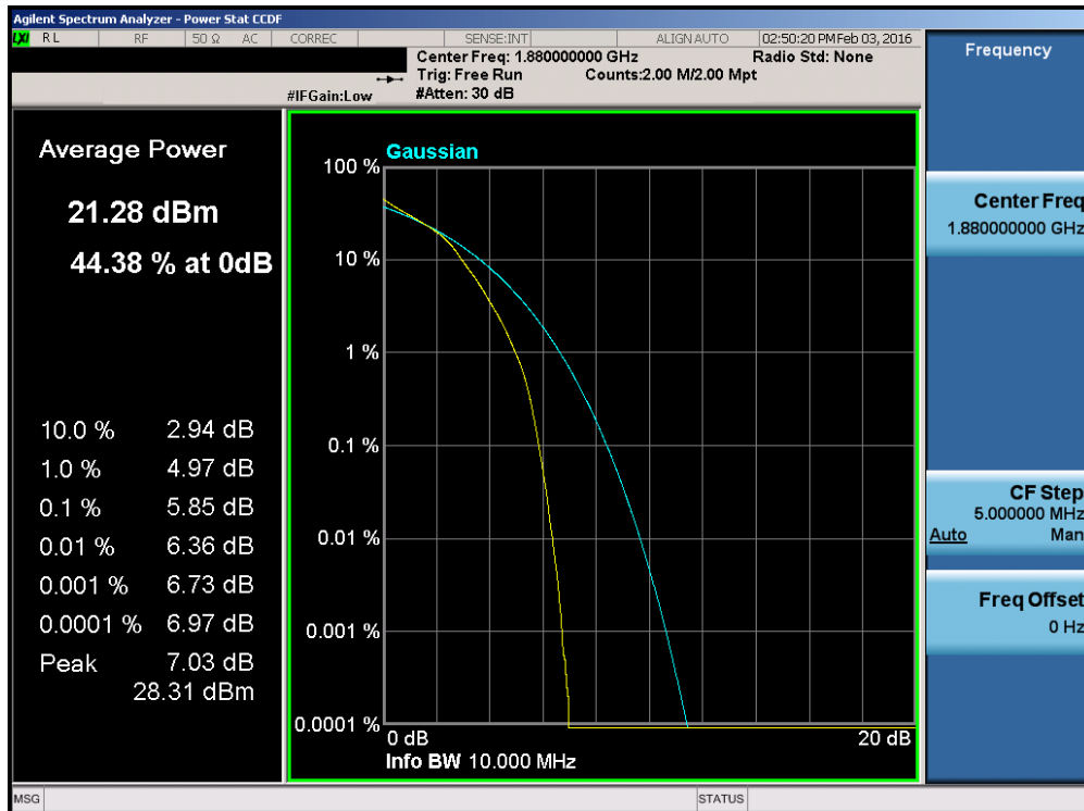
Plot 7-122. PAR Plot (Band 2 – 10.0MHz 16-QAM – RB Size 50)
