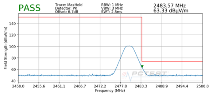
Plot 7-2. Radiated Restricted Upper Band Edge Measurement (Peak)
