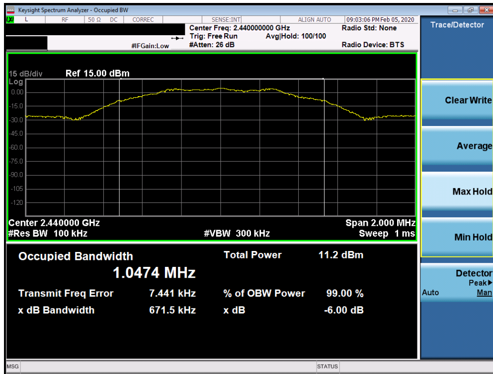
Plot 7-8. 6dB Bandwidth Plot (Bluetooth (LE), 1Mbps – Ch. 19)
