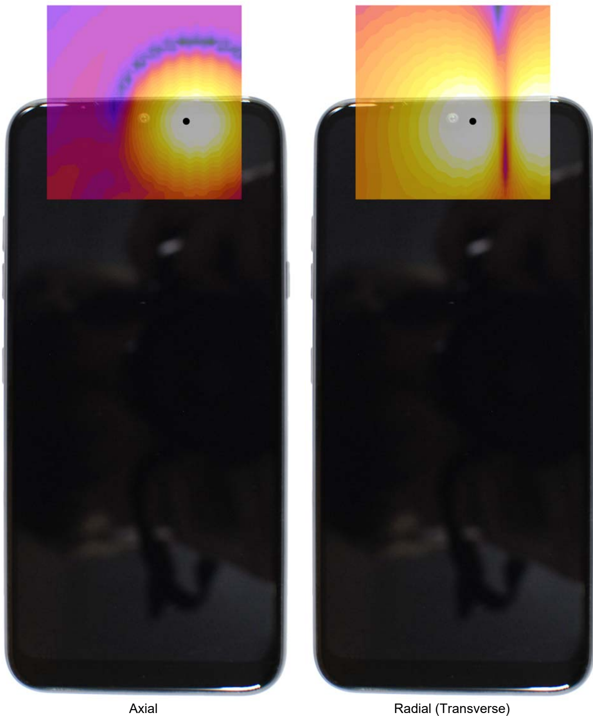
Figure 16-3 T-Coil Scan Overlay Magnetic Field Distributions
