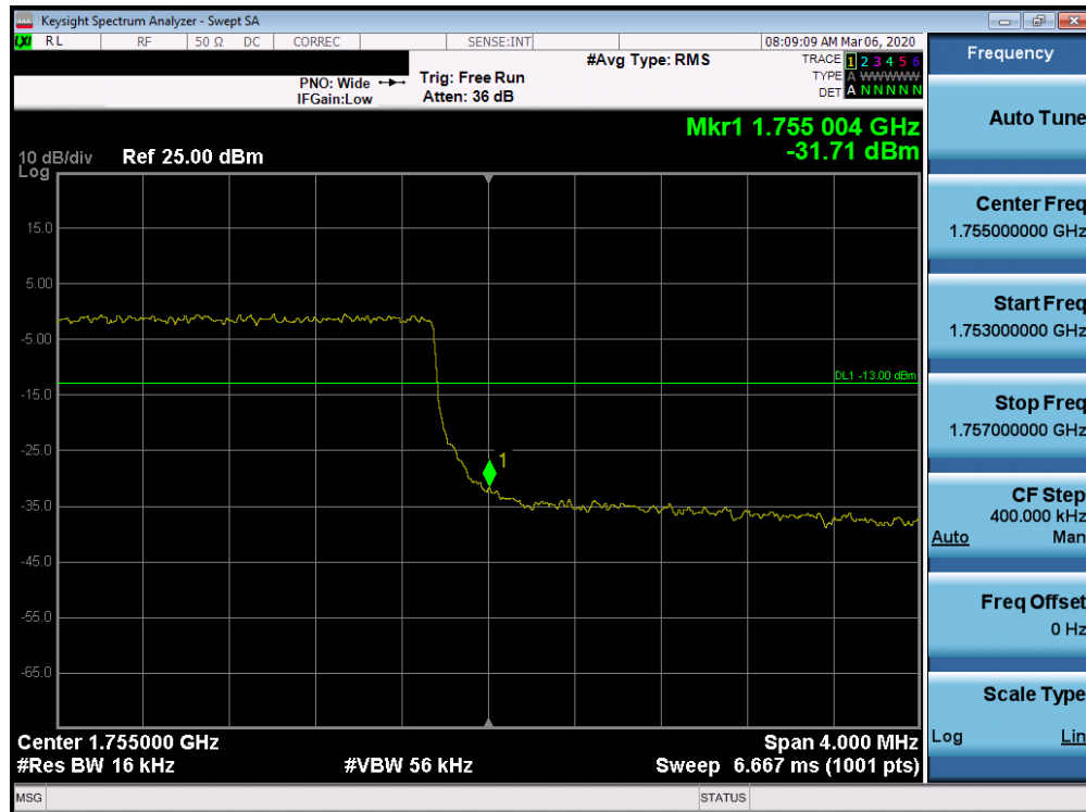
Plot 7-111. Upper Band Edge Plot (Band 4 - 5.0MHz QPSK - Full RB Configuration)
