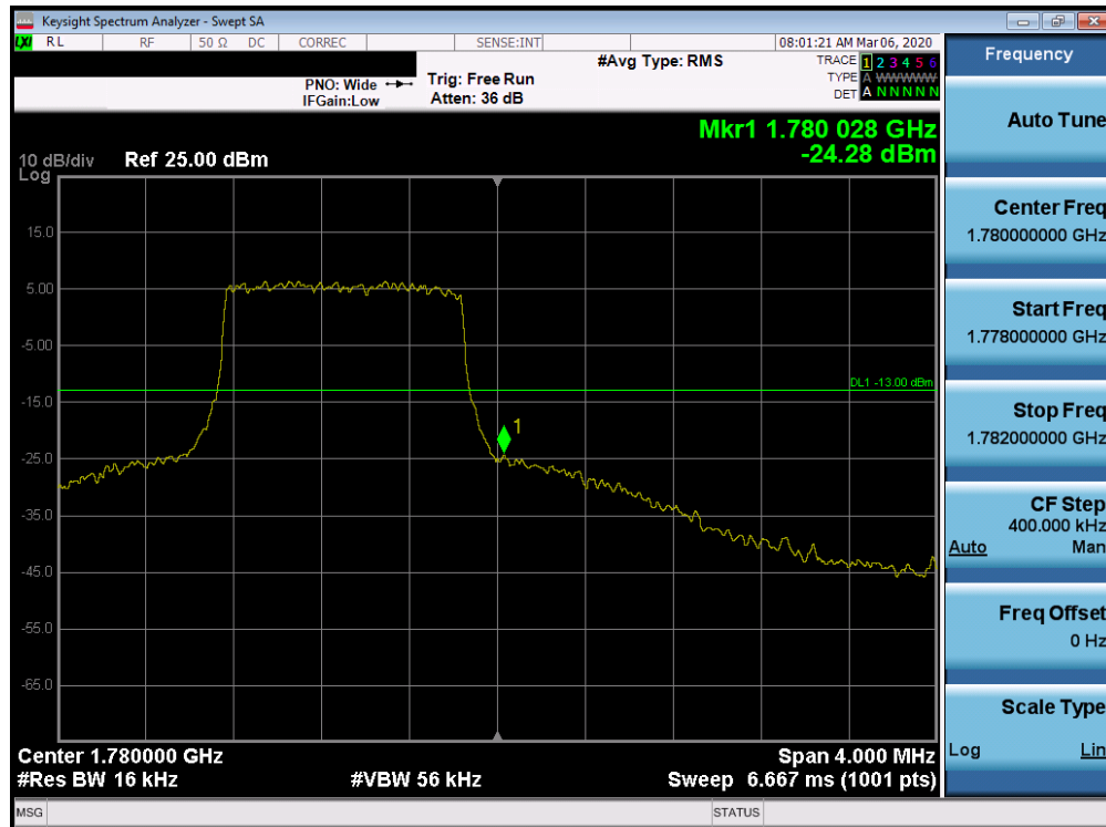
Plot 7-101. Upper Band Edge Plot (Band 66 - 1.4MHz QPSK - Full RB Configuration)
