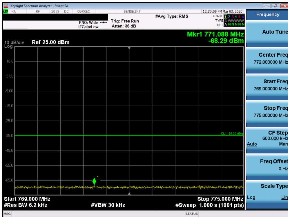
Plot 7-13. Lower Extended Band Edge Plot (LTE Band 14 - 10MHz QPSK - Full RB Configuration)
