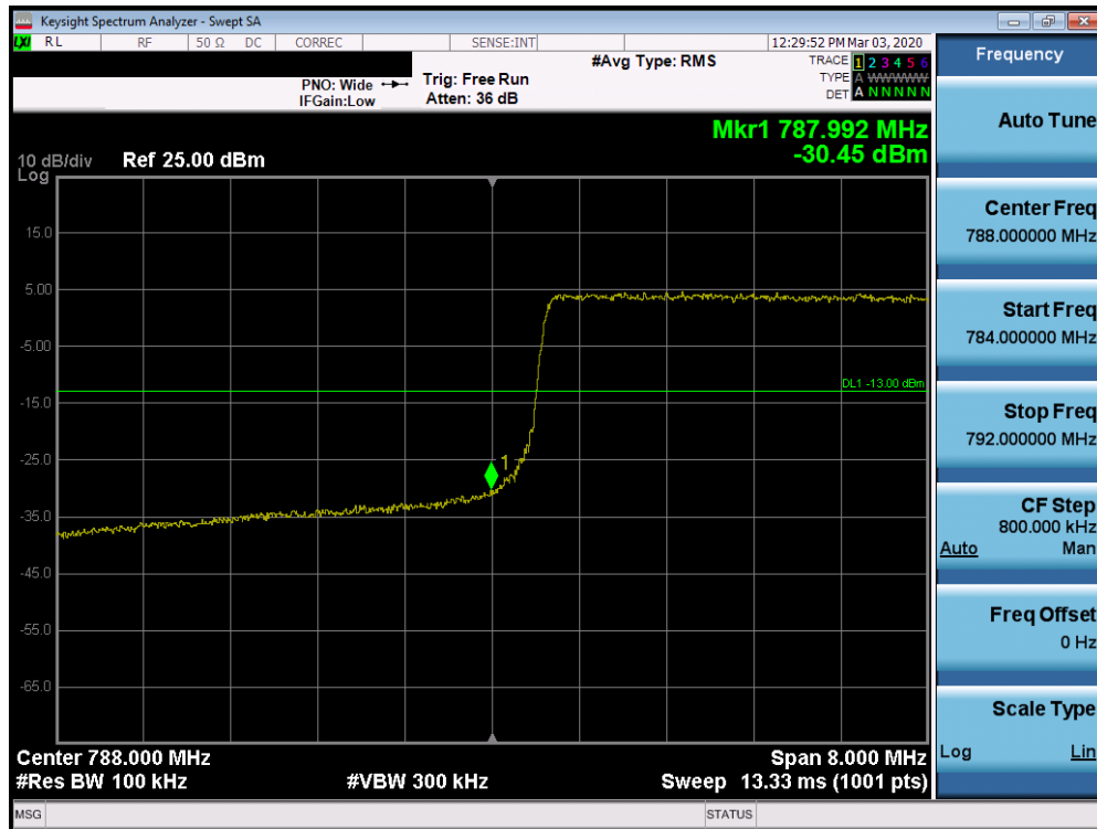
Plot 7-12. Lower Band Edge Plot (Band 14 - 10MHz QPSK – Full RB Configuration)
