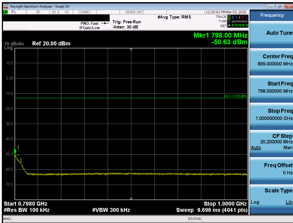
Plot 7-6. Conducted Spurious Plot (LTE Band 14 – 10 MHz QPSK - RB Size 1, RB Offset 0 - Mid Channel)
