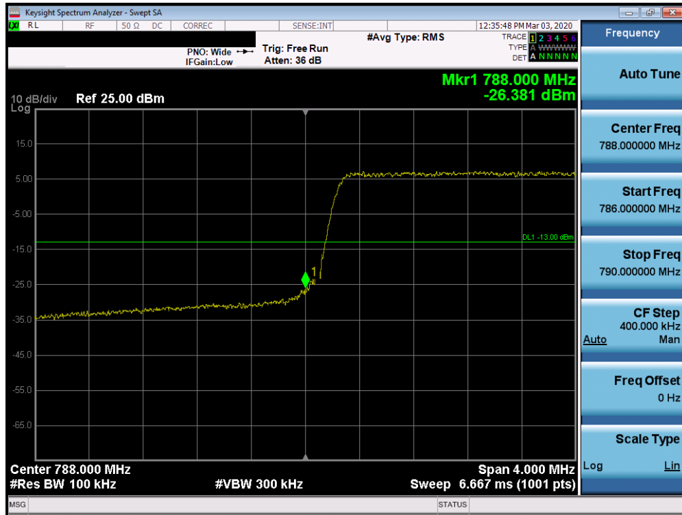
Plot 7-8. Lower Band Edge Plot (Band 14 - 5MHz QPSK – Full RB Configuration)
