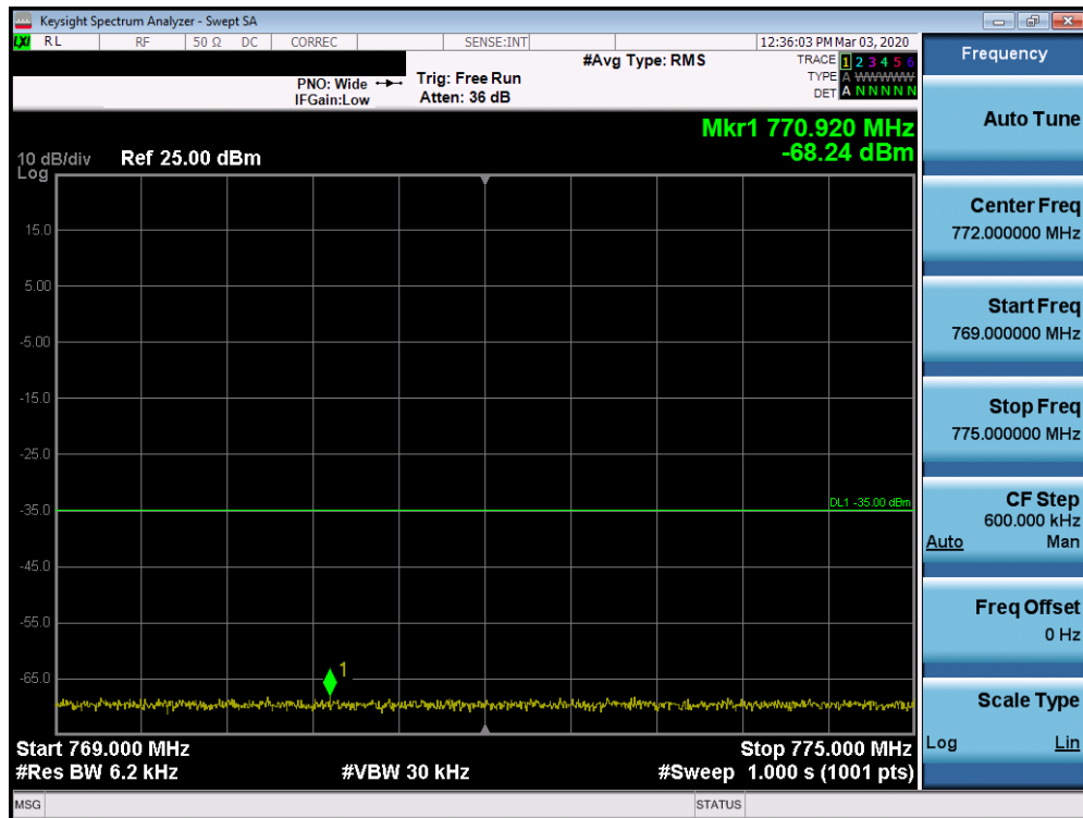
Plot 7-9. Lower Extended Band Edge Plot (Band 14 - 5MHz QPSK – Full RB Configuration)
