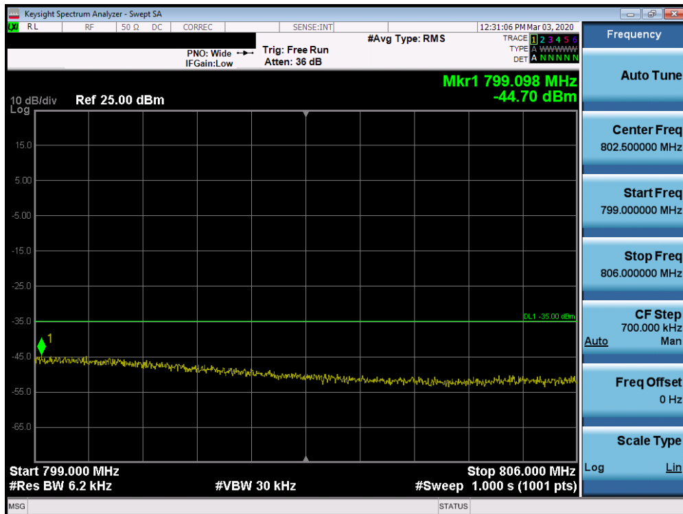
Plot 7-15. Upper Extended Band Edge Plot (LTE Band 14 - 10MHz QPSK - Full RB Configuration)
