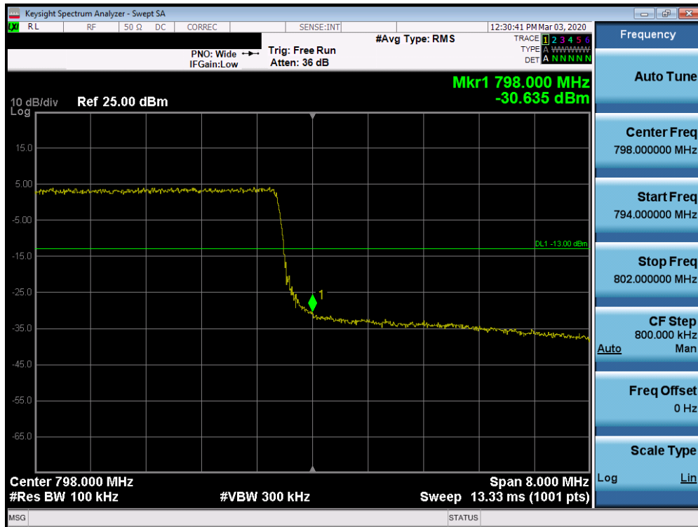
Plot 7-14. Upper Band Edge Plot (Band 14 - 10MHz QPSK – Full RB Configuration)
