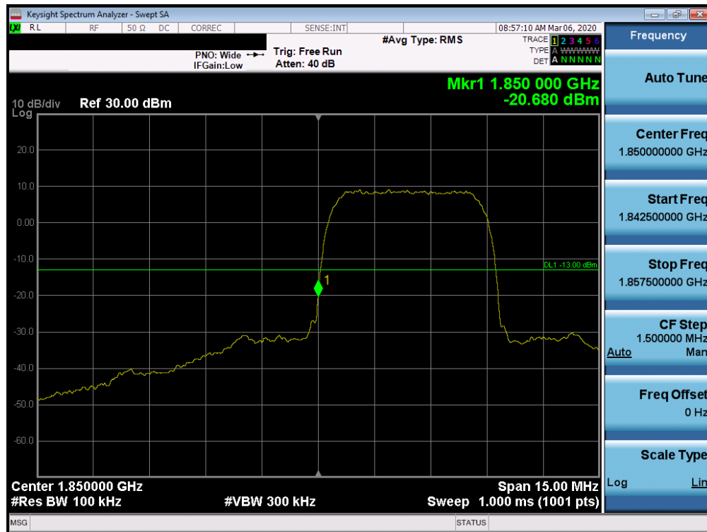
Plot 7-9. Band Edge Plot (PCS WCDMA Mode – Low Channel)
