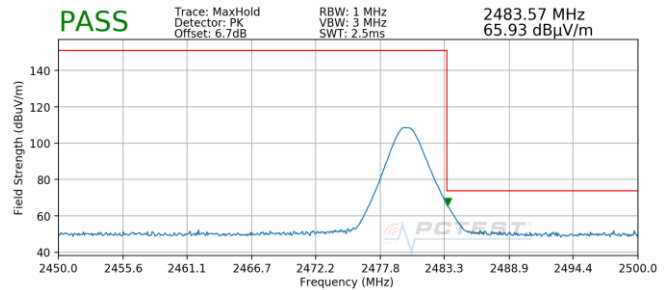
Plot 7-6. Radiated Restricted Upper Band Edge Measurement (Peak)
