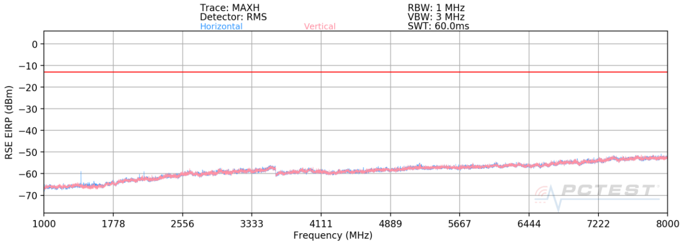
Plot 7-7. Radiated Spurious Plot (LTE Band 12)
