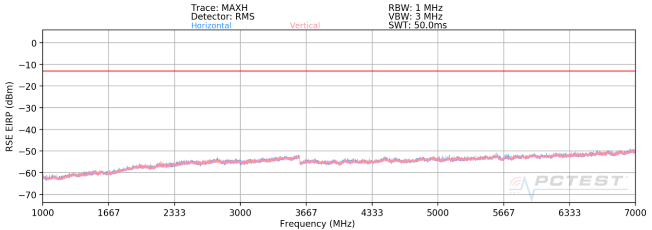
Plot 7-10. Radiated Spurious Plot (LTE Band 71)
