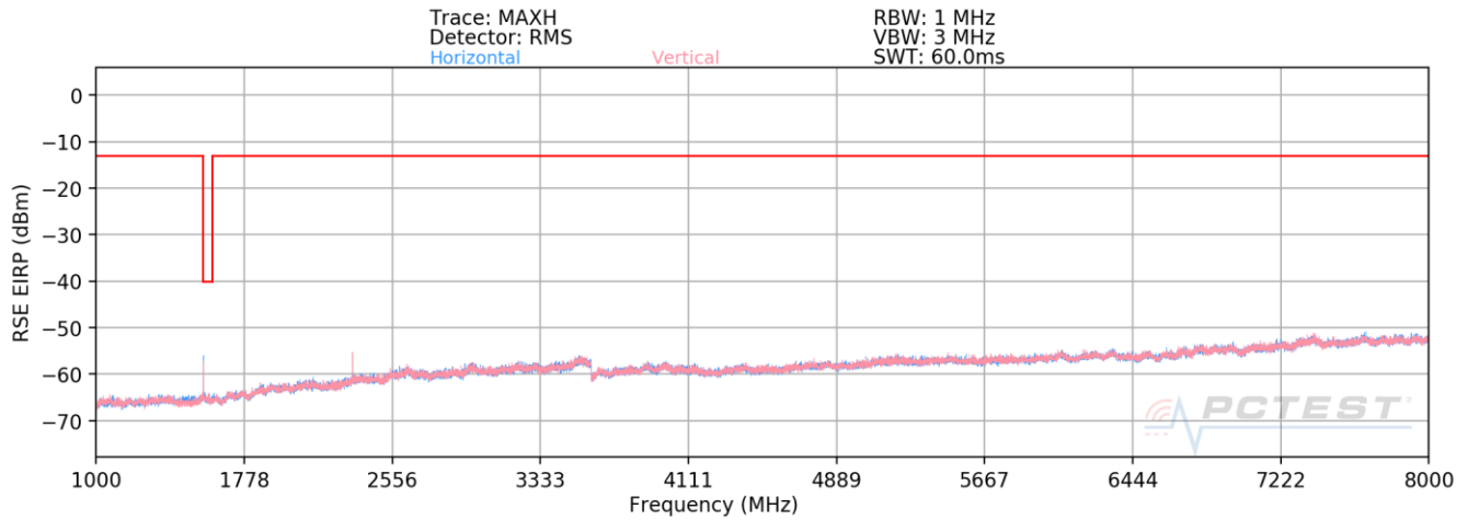
Plot 7-8. Radiated Spurious Plot (LTE Band 13)
