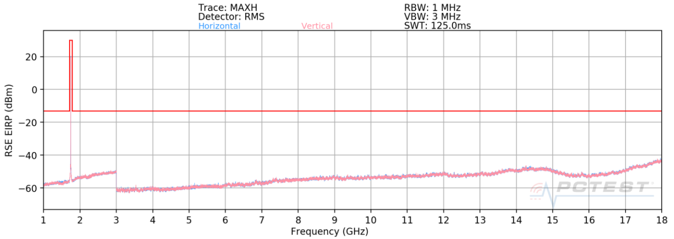
Plot 7-6. Radiated Spurious Plot (LTE Band 66/4)
