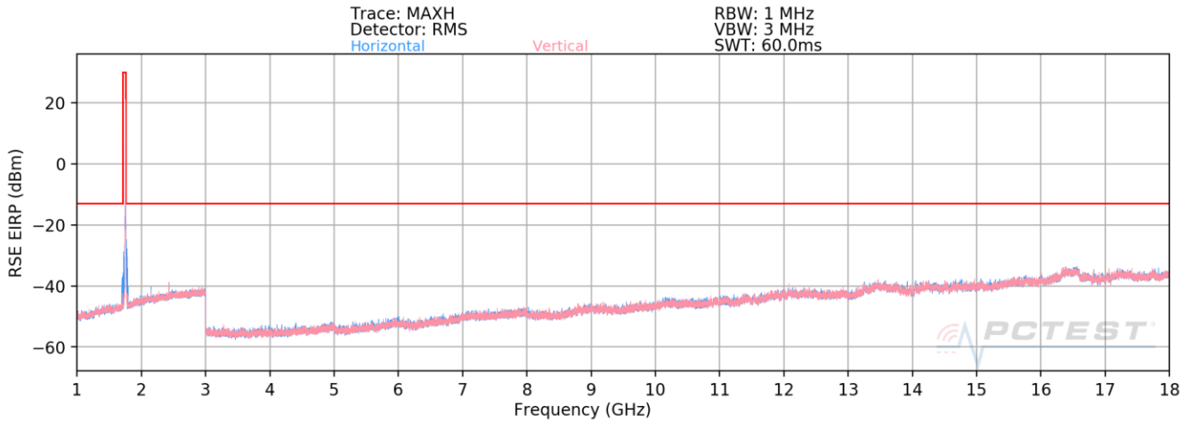
Plot 7-11. Radiated Spurious Plot (WCDMA AWS)
