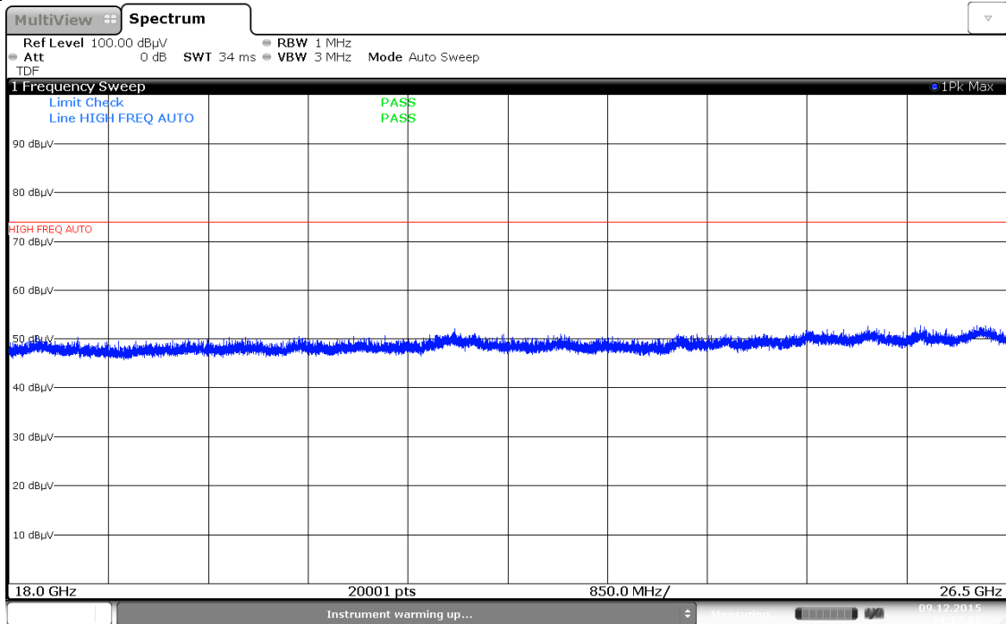
Plot 7-45. Radiated Spurious Plot above 18GHz (Pol. H)
