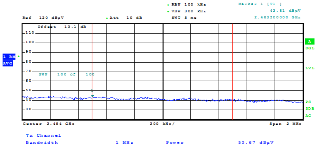
Plot 7-57. Radiated Restricted Upper Band Edge Measurement (Average)
