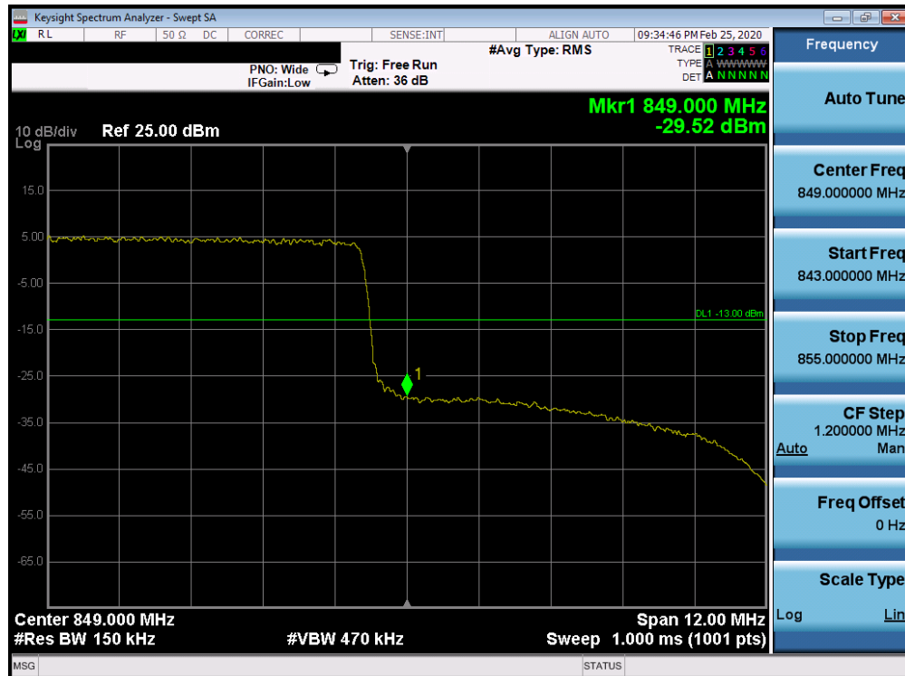
Plot 7-196. Upper Band Edge Plot (Band 26 - 15.0MHz QPSK - Full RB Configuration)
