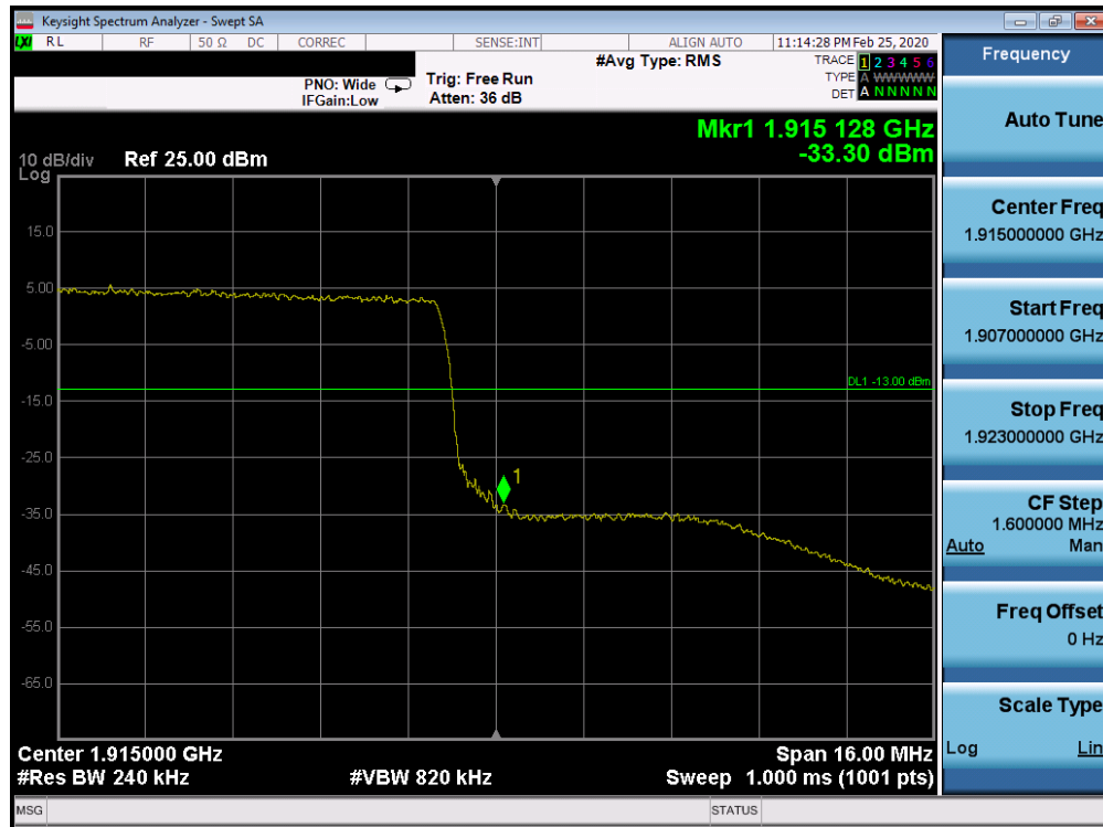
Plot 7-265. Upper Band Edge Plot (Band 25 - 20.0MHz QPSK - Full RB Configuration)
