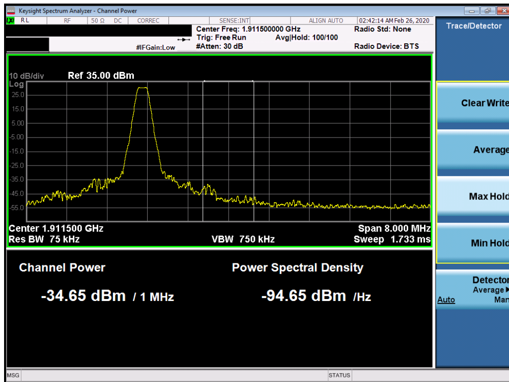
Plot 7-78. 8MHz Span Plot (PCS GSM Mode - High Channel)
