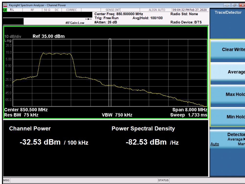
Plot 7-82. 8MHz Span Plot (Cellular CDMA Mode - High Channel)
