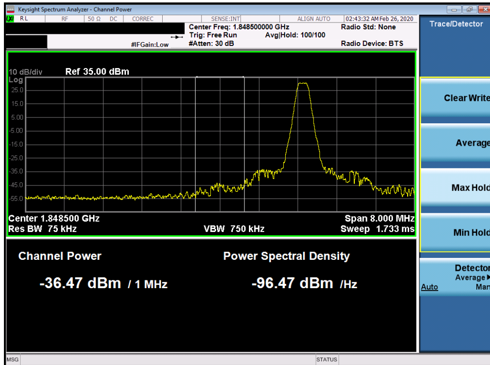
Plot 7-76. 8MHz Span Plot (PCS GSM Mode - Low Channel)
