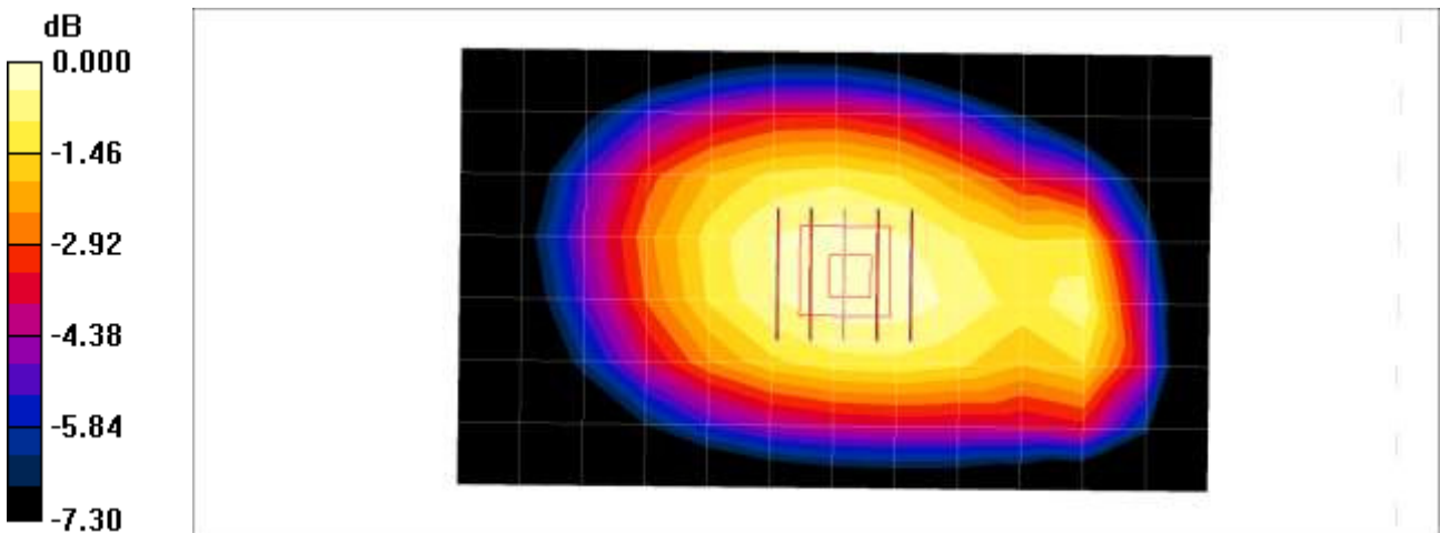
0 dB = 0.282mW/g
