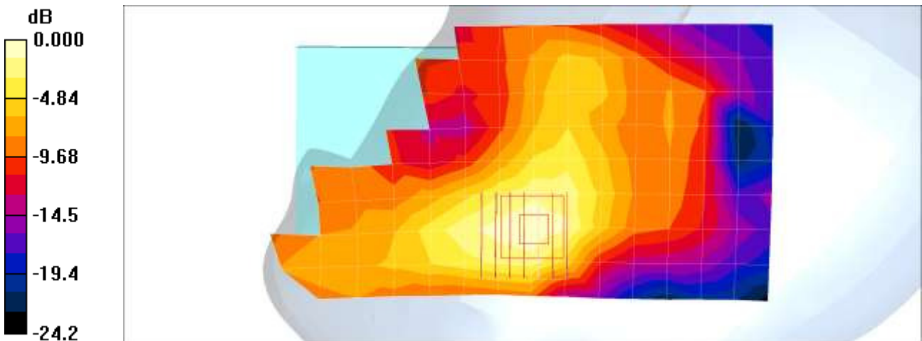
0 dB = 0.262mW/g
