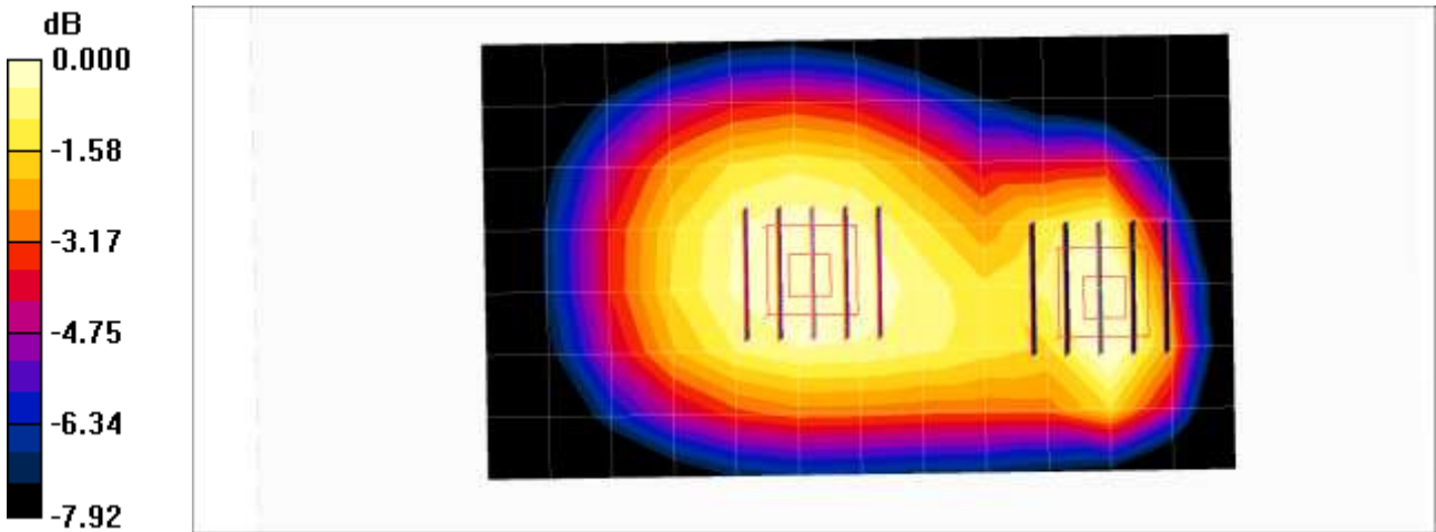
0 dB = 0.593mW/g
