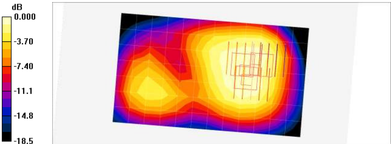
0 dB = 0.642mW/g
