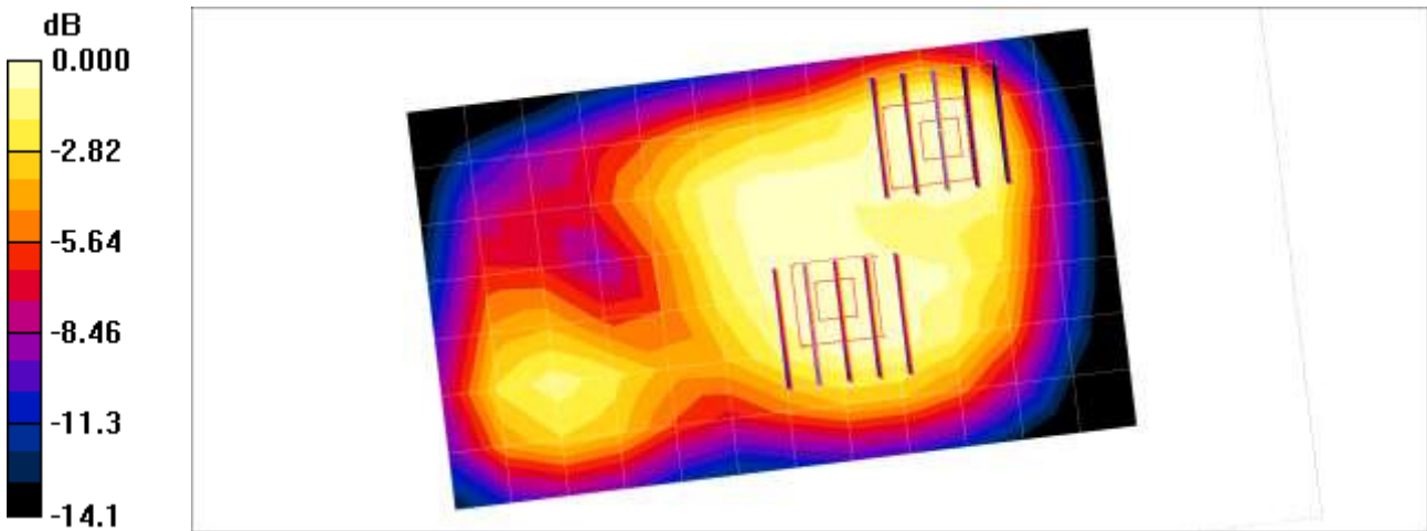
0 dB = 0.506mW/g
