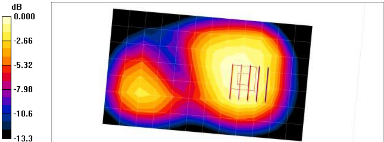
0 dB = 0.503mW/g
