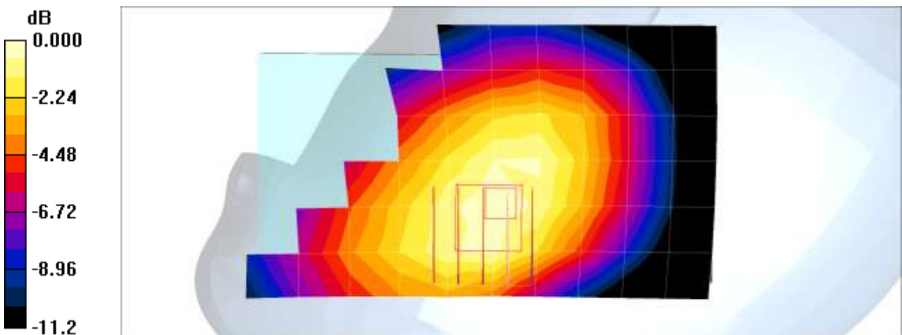
0 dB = 0.359mW/g
