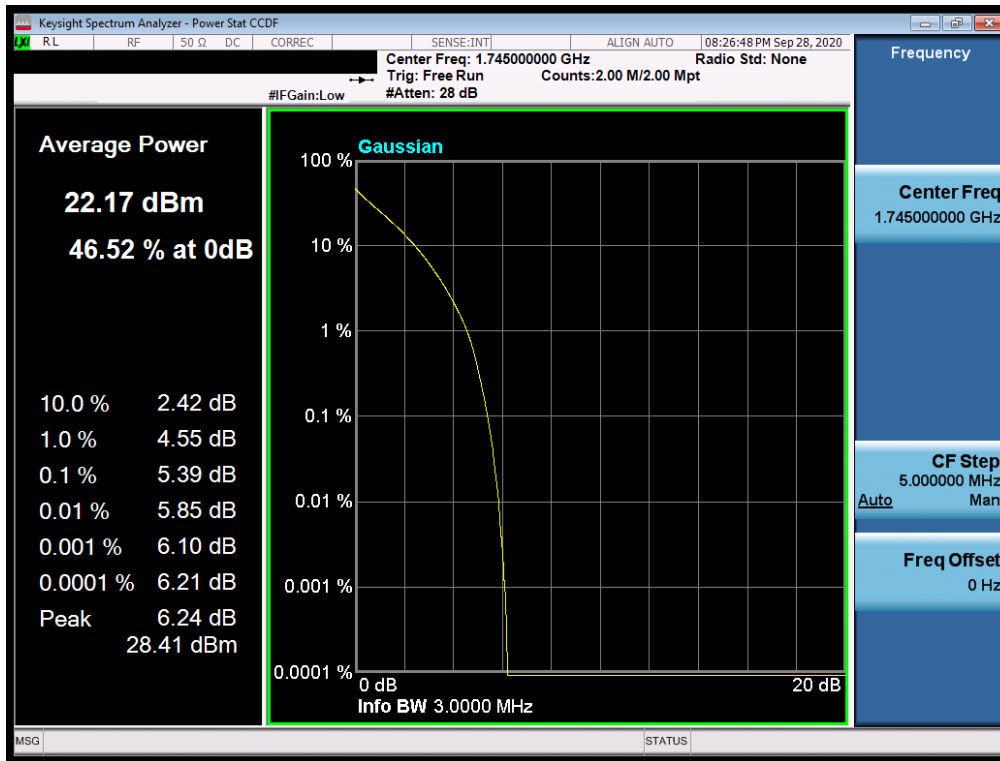
Plot 7-157. PAR Plot (LTE Band 66/4 - 3MHz QPSK - Full RB Configuration)
