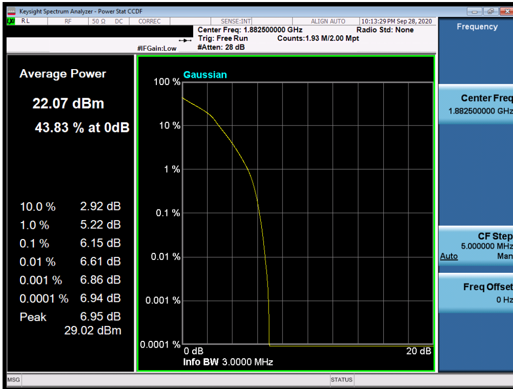
Plot 7-112. PAR Plot (LTE Band 25/2 - 3MHz 16-QAM - Full RB Configuration)
