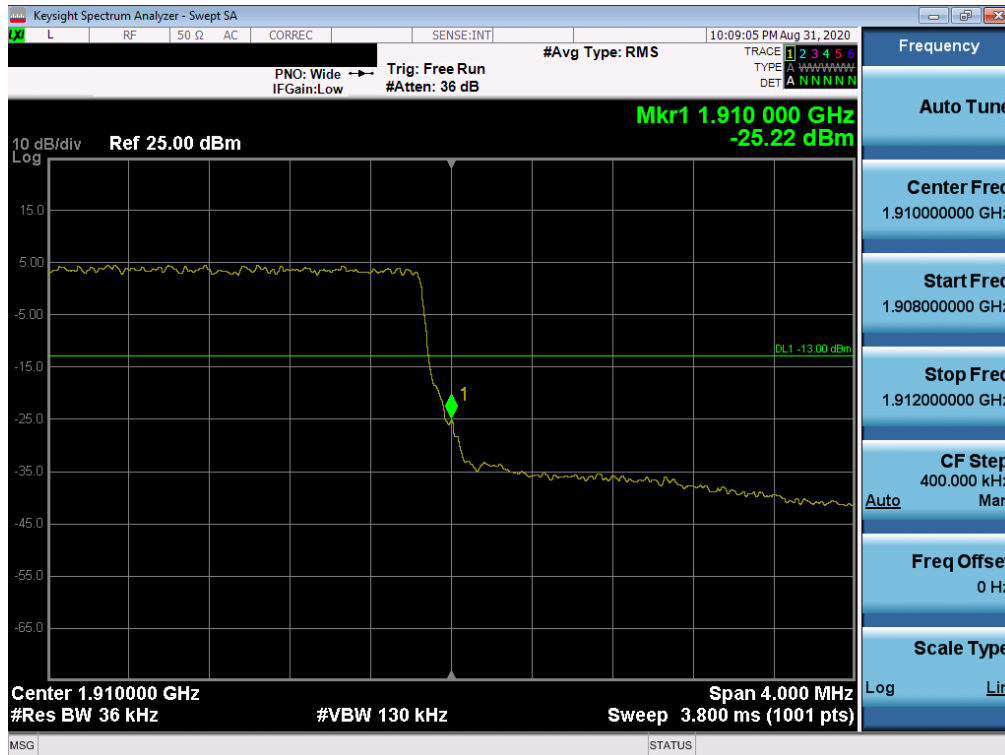
Plot 7-81. Upper Band Edge Plot (LTE Band 2 - 3MHz QPSK – Full RB Configuration)
