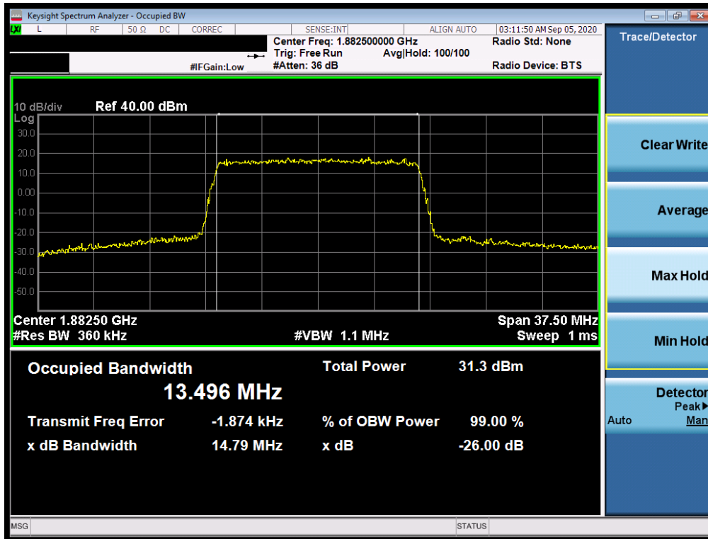
Plot 7-5. Occupied Bandwidth Plot (LTE Band 25/2 - 15MHz 16-QAM - Full RB Configuration)
