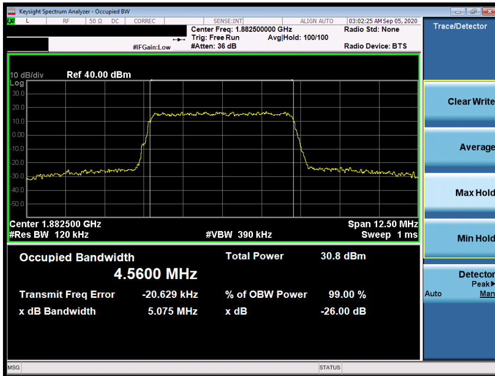
Plot 7-10. Occupied Bandwidth Plot (LTE Band 25/2 - 5MHz QPSK - Full RB Configuration)
