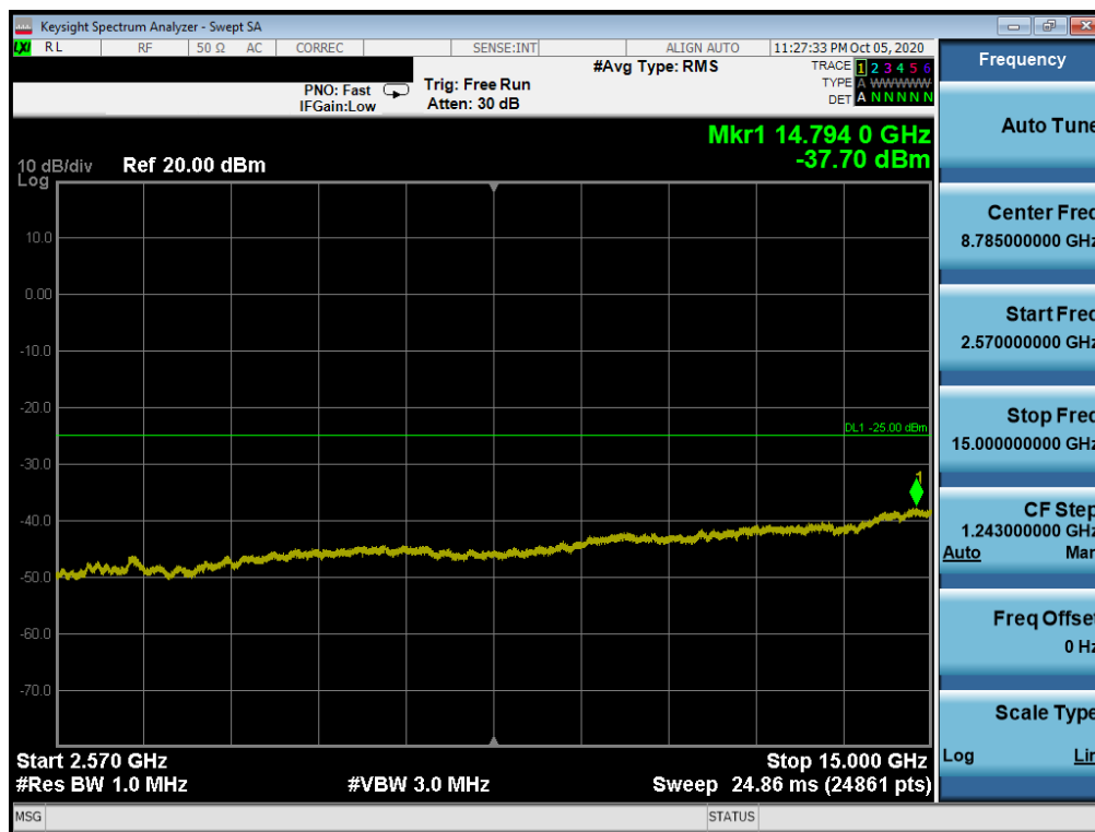
Plot 7-14. Conducted Spurious Plot (LTE Band 7 - 20MHz QPSK - RB Size 1, RB Offset 0 - Low Channel)
