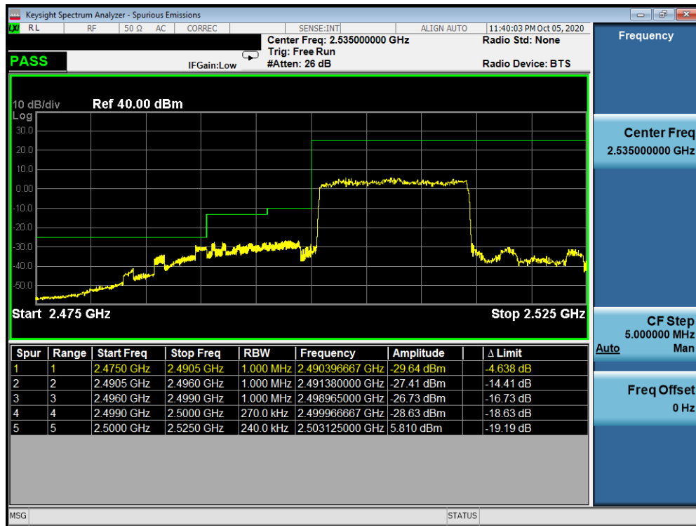
Plot 7-24. Lower ACP Plot (LTE Band 7 - 15MHz QPSK – Full RB Configuration)
