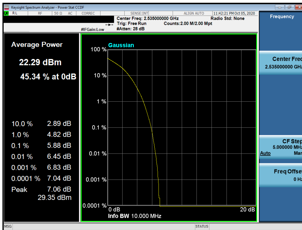
Plot 7-36. PAR Plot (LTE Band 7 - 10MHz 16-QAM - Full RB Configuration)
