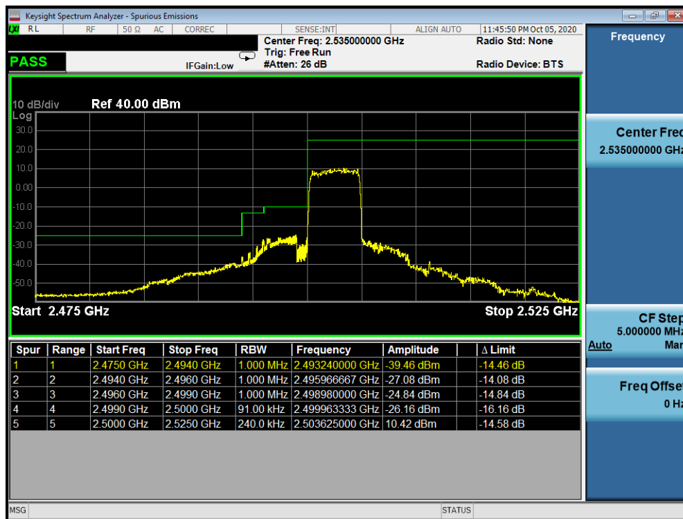
Plot 7-28. Lower ACP Plot (LTE Band 7 - 5MHz QPSK - Full RB Configuration)
