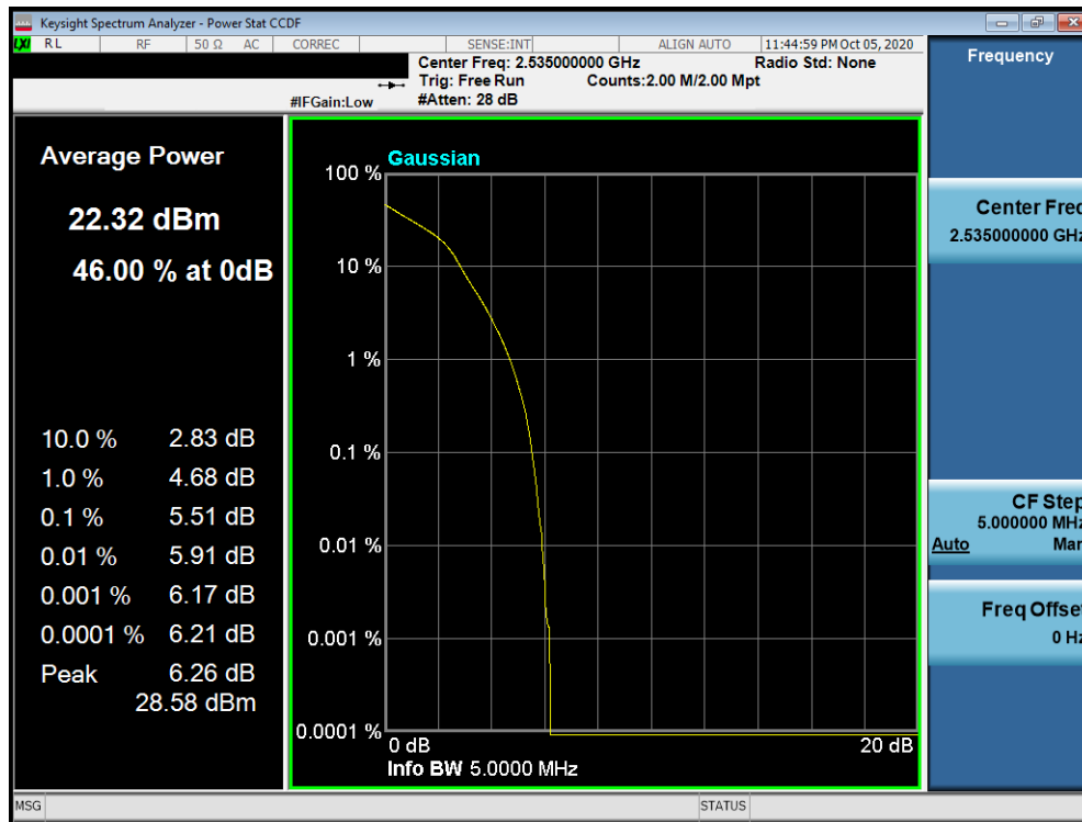
Plot 7-38. PAR Plot (LTE Band 7 - 5MHz 16-QAM - Full RB Configuration)
