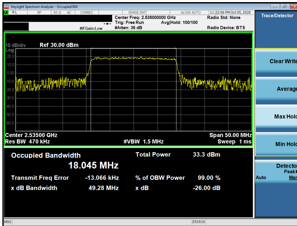
Plot 7-1. Occupied Bandwidth Plot (LTE Band 7 - 20MHz QPSK - Full RB Configuration)
