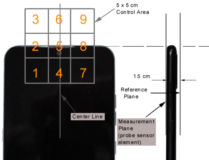
Figure 17-3 5x5 Scan grid above WD (Acoustic scan area pictured)
