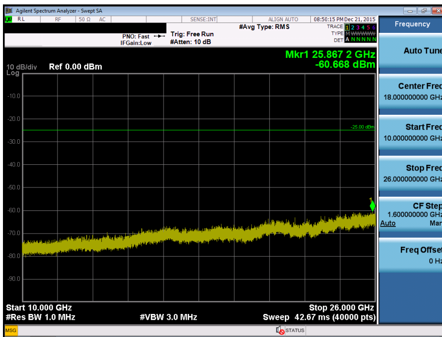
BAND7. Conducted Spurious Plot 2 (10MHz Ch.21400 QPSK RB 1, Offset 0)
