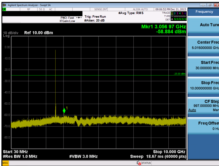
BAND7. Conducted Spurious Plot 1 (10MHz Ch.21400 QPSK RB 1, Offset 0)
