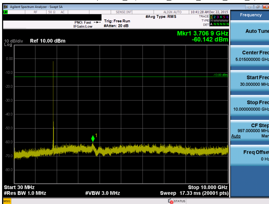
BAND 2. Conducted Spurious_1 (18675ch_15MHz_QPSK_RB 1_0)
