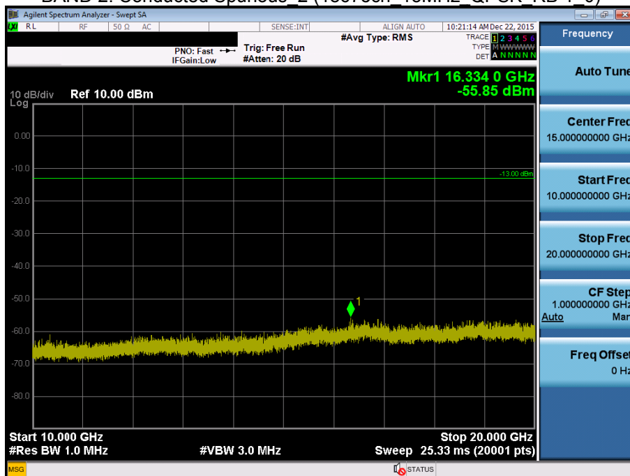
BAND 2. Conducted Spurious_2 (18675ch_15MHz_QPSK_RB 1_0)
