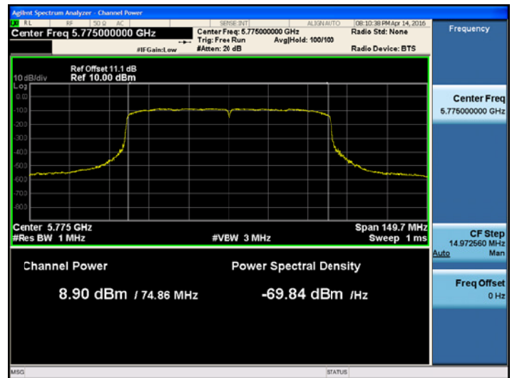
802.11ac_VHT80 UNII 3 BAND Average Power (5775 MHz) CH 155 MCS0
