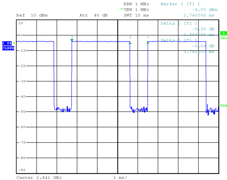
Figure 8-1 Bluetooth Transmission Plot
