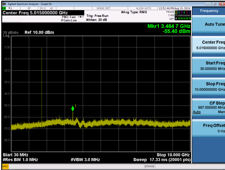
BAND 4. Conducted Spurious Plot_1 (20175ch_1.4MHz_QPSK_RB 1_0)
