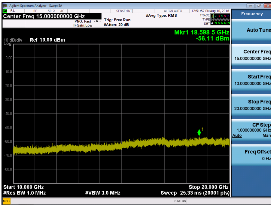
BAND 4. Conducted Spurious Plot_2 (20175ch_1.4MHz_QPSK_RB 1_0)
