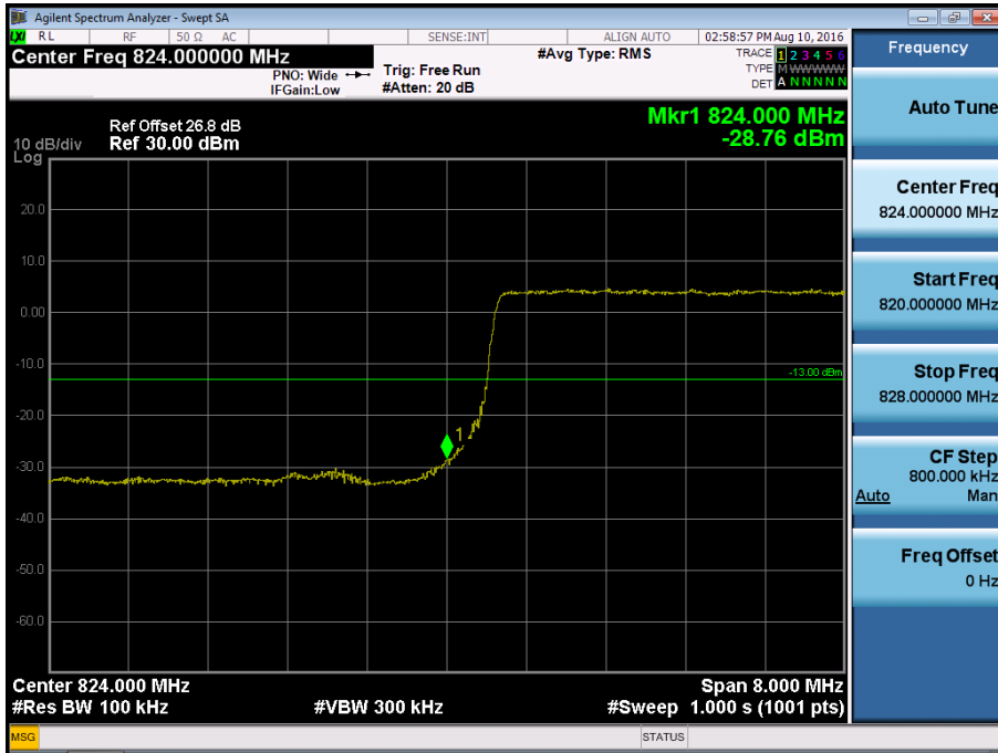
BAND 5. Lower Band Edge Plot (10M BW Ch.20450 QPSK_RB50_Offset 0)
