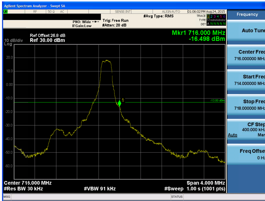
BAND 12. Upper Band Edge Plot (1.4M BW Ch.23173 QPSK_RB1_Offset 5)
