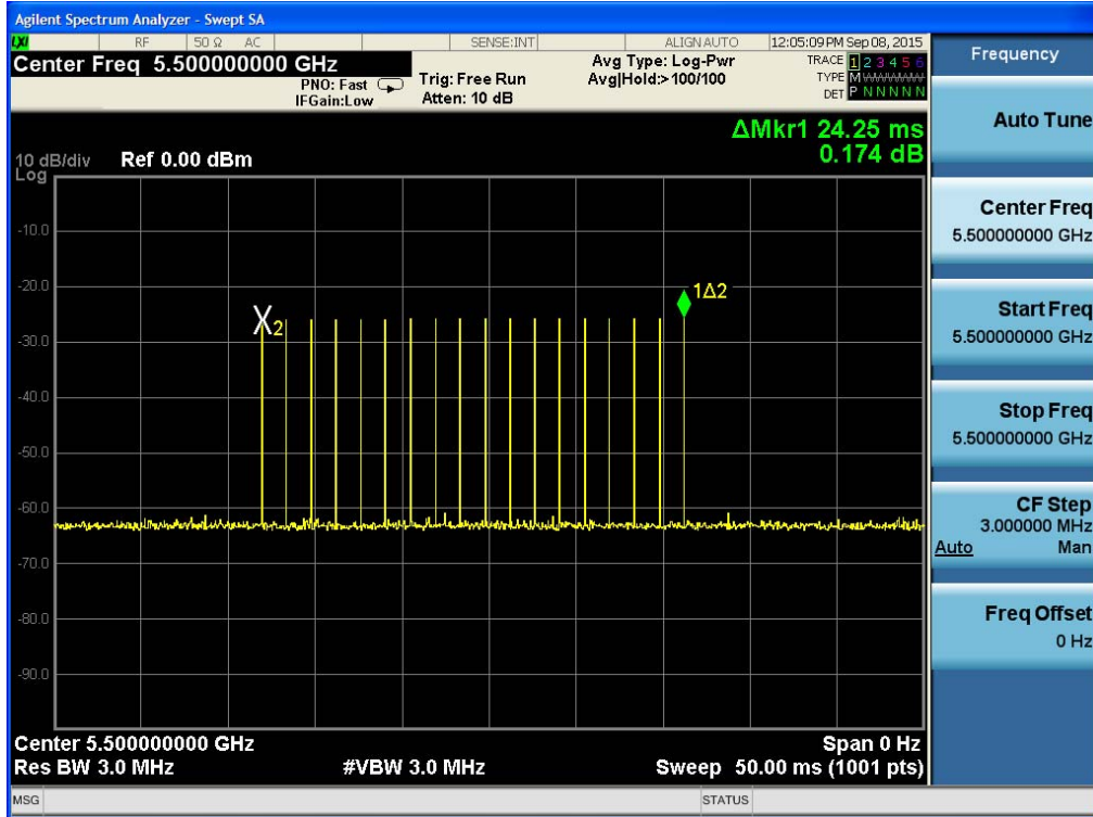
Type0 Radar Pulse Number – Ch.100
