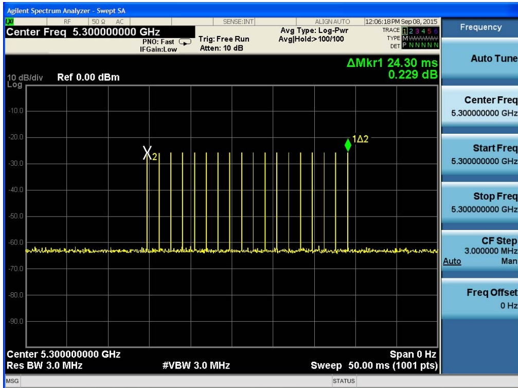
Type0 Radar Pulse Number – Ch.60
